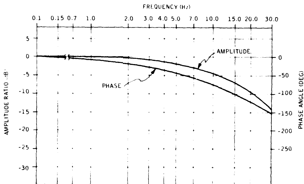
Figure B-3. Servomotor Frequency Response.
