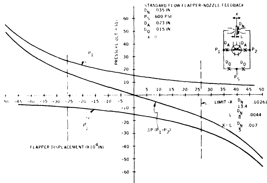
Figure 11. Standard Flow Flapper-Nozzle Feedback.
