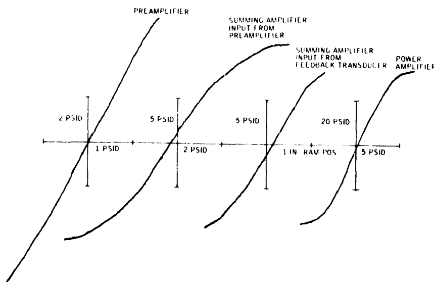
Figure 17. Amplifier Gain Curves.
