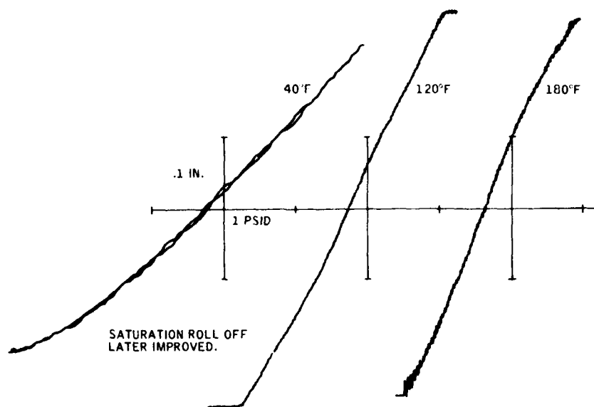
Figure 24. Servoactuator Gain Curves (Final Configuration).
