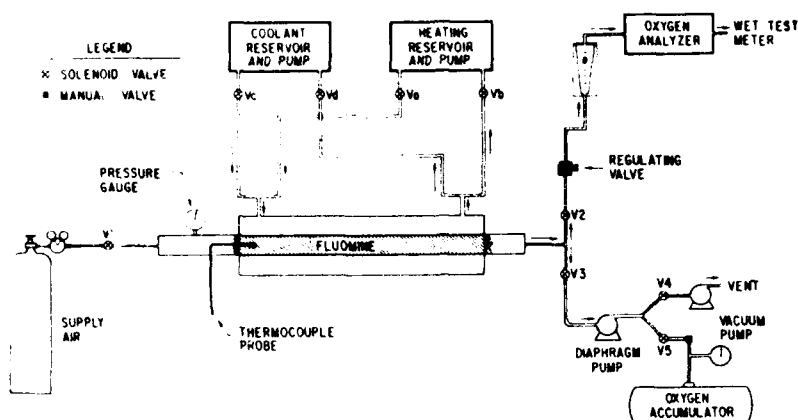
Figure 2. Schematic diagram of laboratory apparatus for study of fluomine off-gassing.
