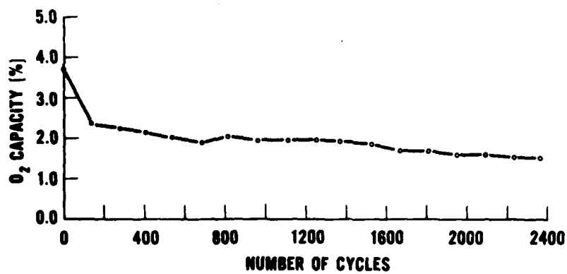
Figure 14. Run 1C: (a) Major contaminants in fluomine product oxygen; (b) Degradation of fluomine with use.
