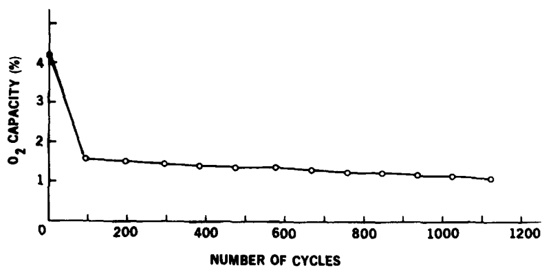
Figure 13. Run 2B--Effects of using pure oxygen supply gas on (a) fluomine off-gassing and (b) fluomine degradation.
