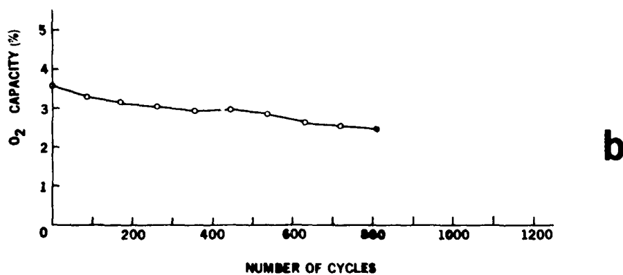
Figure 6. Run 4A--Effects of supply air containing 1000 ppm CO and O 2 purity: (a) Major contaminants in fluomine product oxygen; (b) Degradation of fluomine with use.
