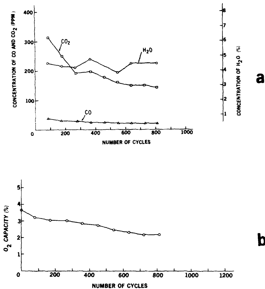
Figure 5. Run 3A: (a) Major contaminants in fluomine product oxygen; (b) Degradation of fluomine with use.
