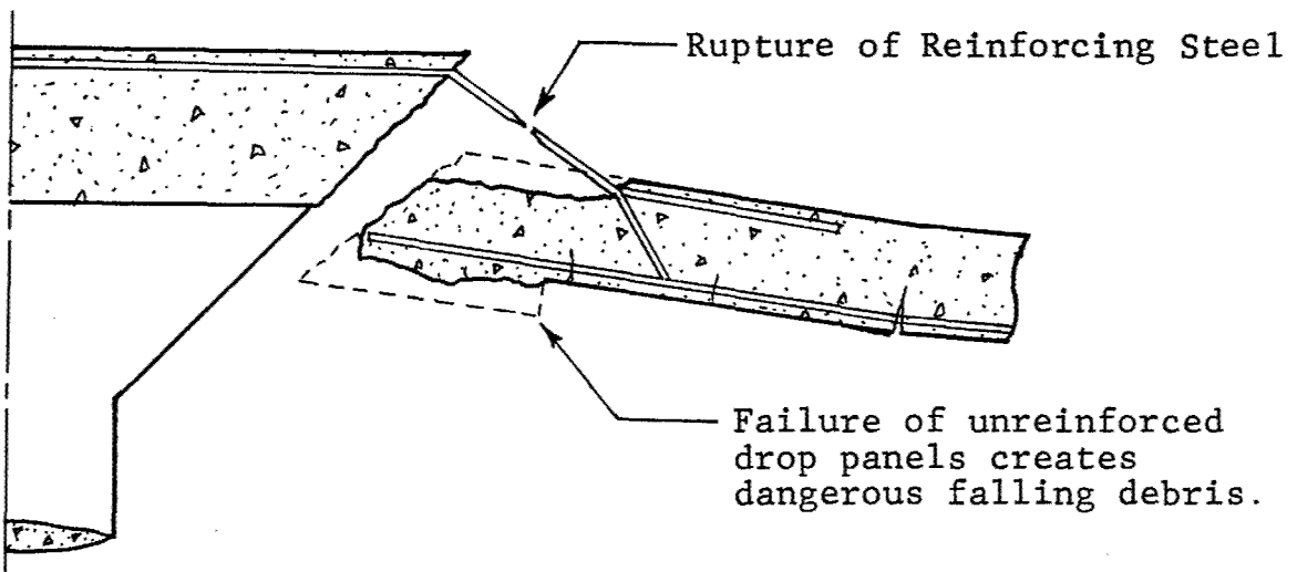
c) Rupture of Reinforcing Steel Leading to Ultimate Collapse of the Slab
