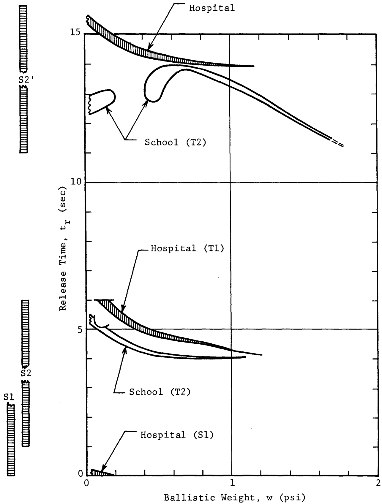
Figure 66 Impact Domains for Targets T1 and T2
