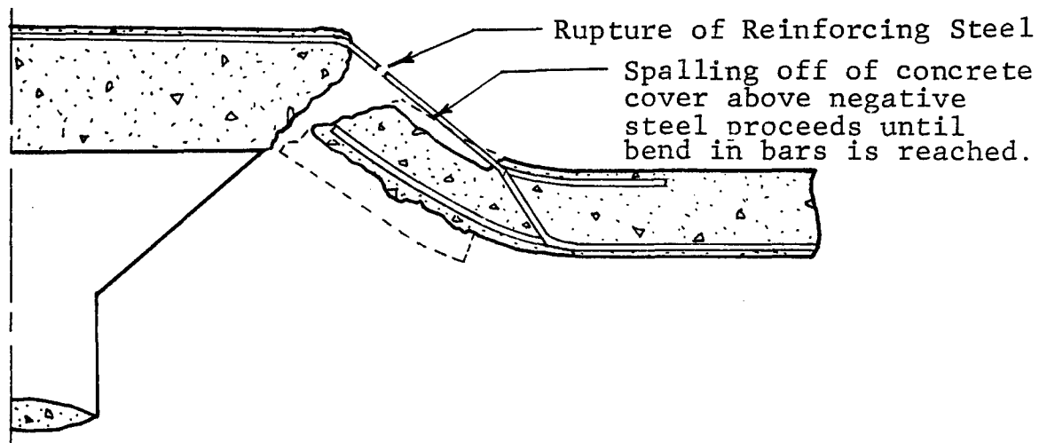
c) Rupture of Reinforcing Steel Leading to Ultimate Collapse of the Slab
