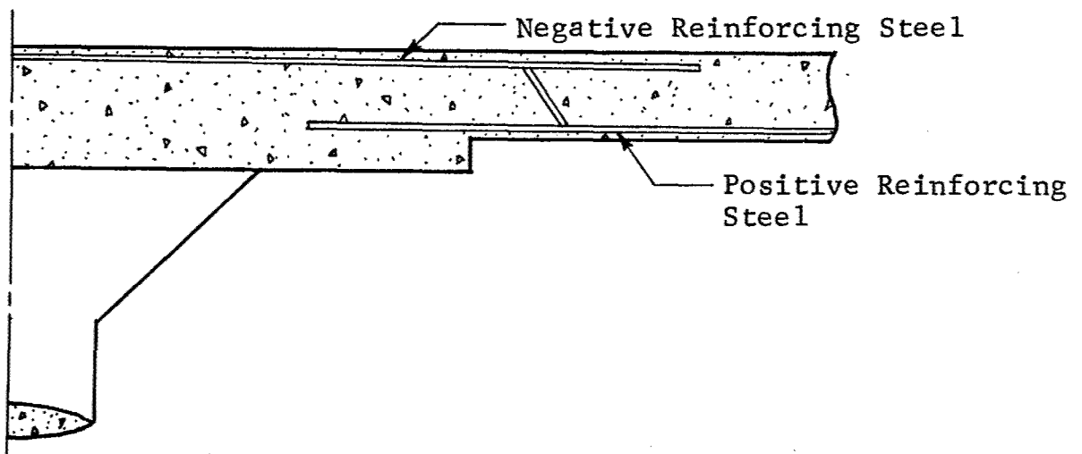
a) Initial Slab Configuration
