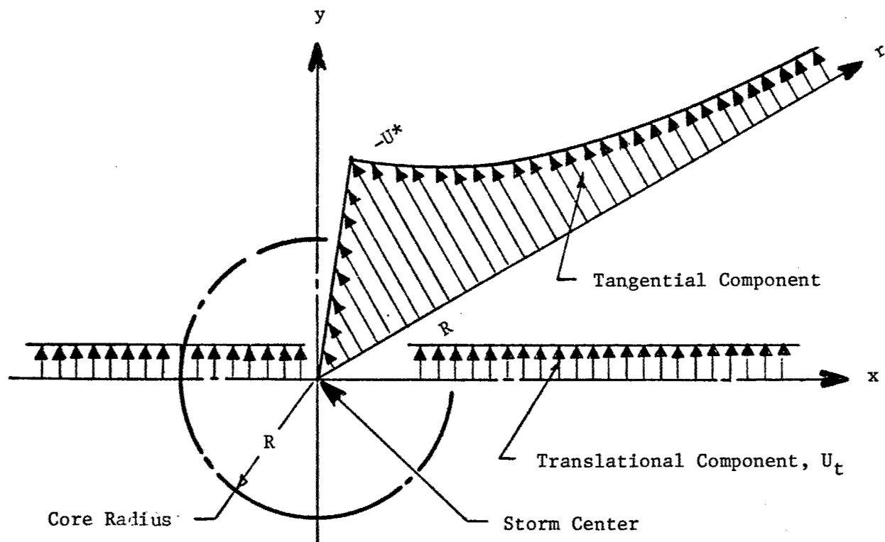
a) Velocity Field
