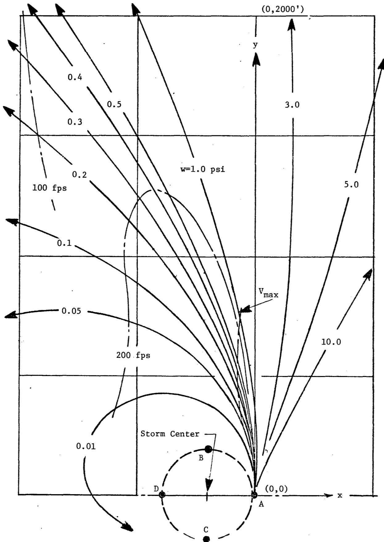
Figure 47 Influence of Ballistic Weight on Debris Trajectories
