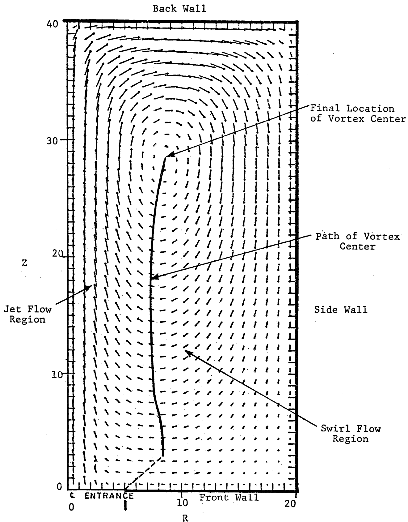
Figure 33 Velocity Diagram - Cycle 750
