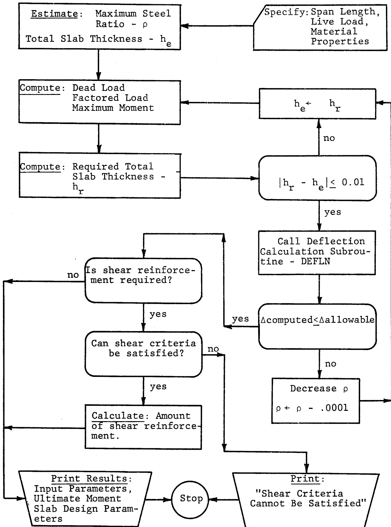
Figure 13 Flowchart for One-Way Slab Design Procedure
