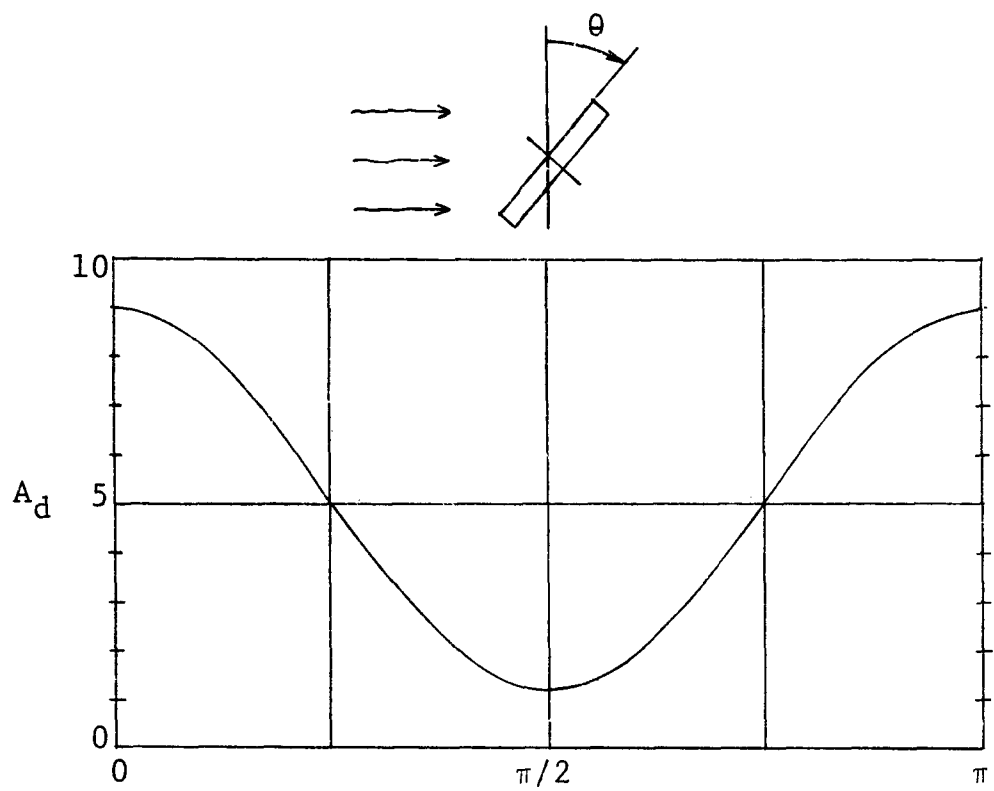
a) Variation of Drag Area ( A_d ) with \theta
