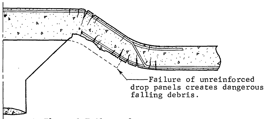
b) Flexural Failure of Concrete at Incipient Collapse
