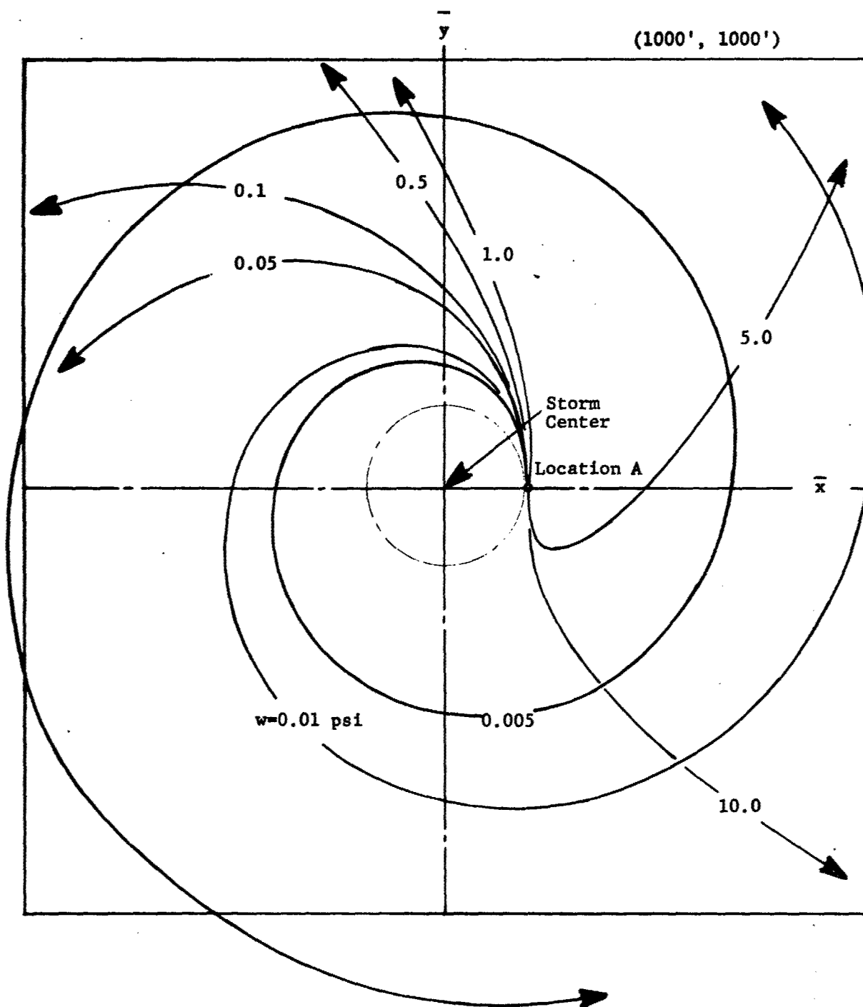
Figure 55 Debris Trajectories Relative to Storm System
