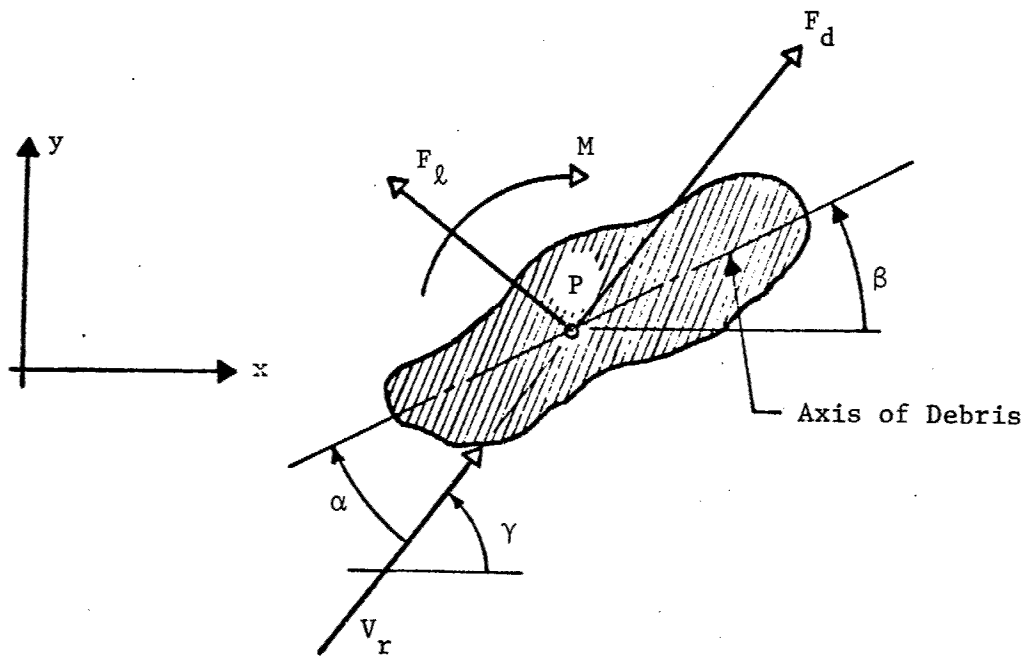
b) Two-Dimensional Rotating Debris Model
