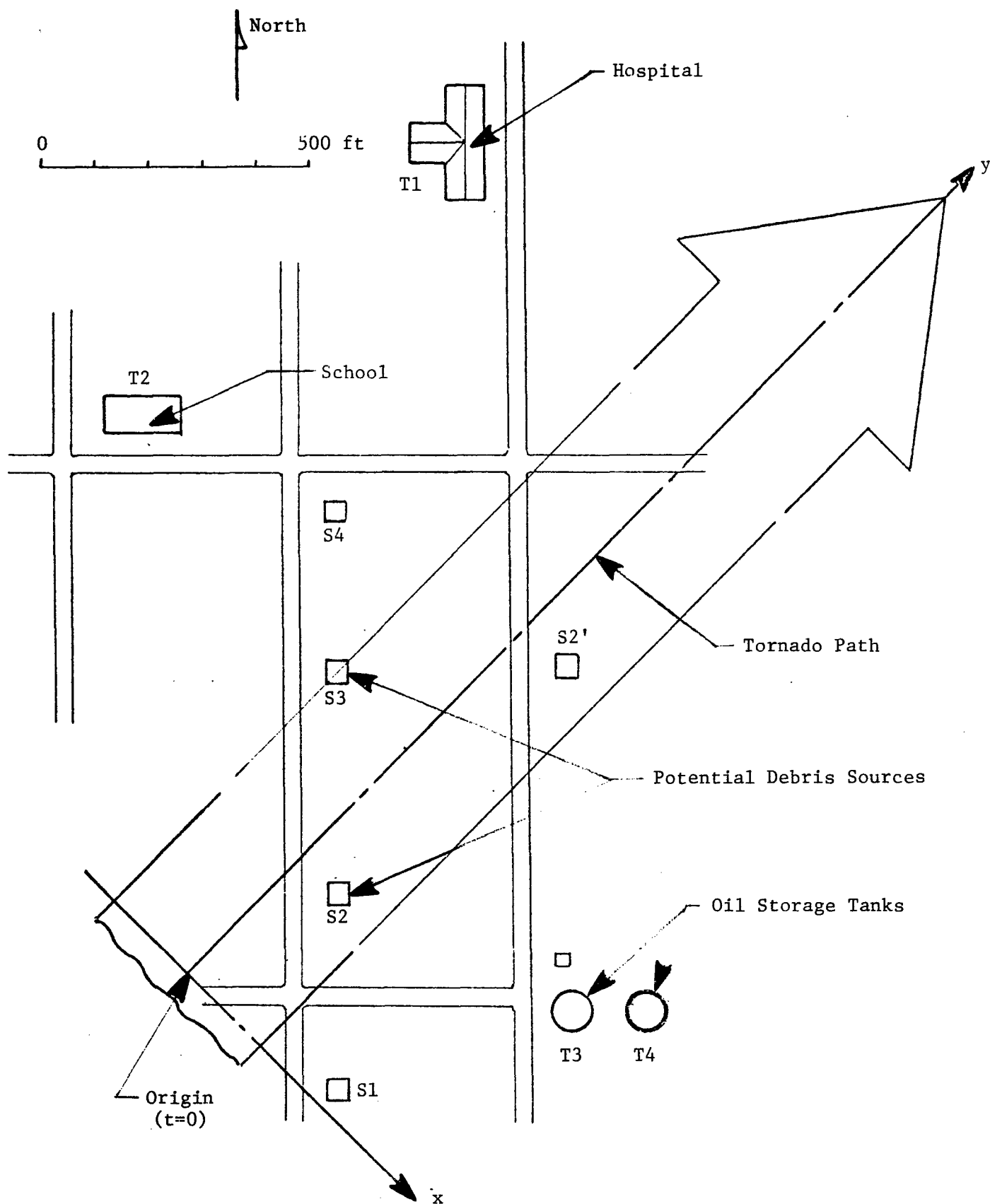
Figure 60 Layout of Targets and Potential Debris Sources
