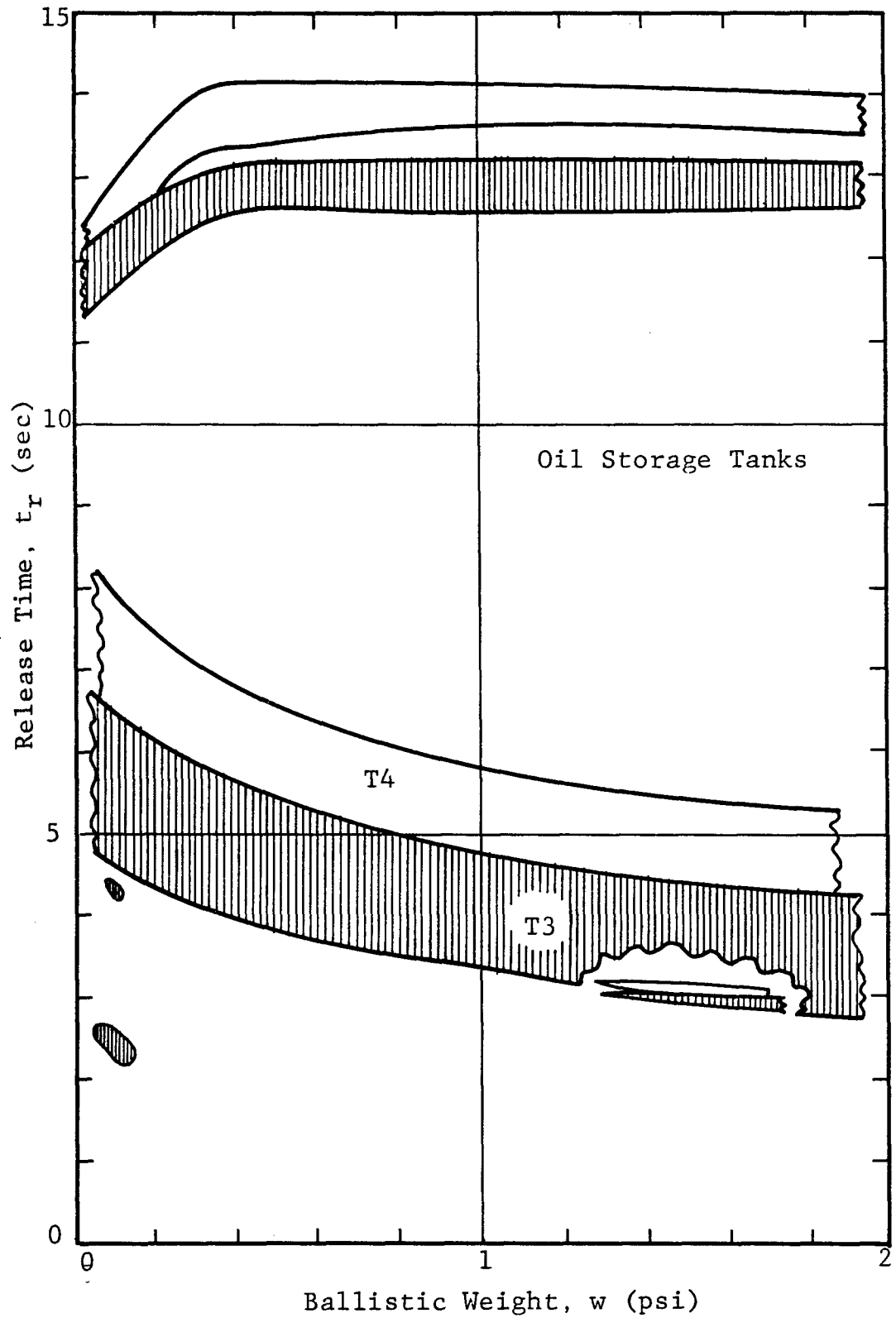
Figure 67 Impact Domains for Targets T3 and T4
