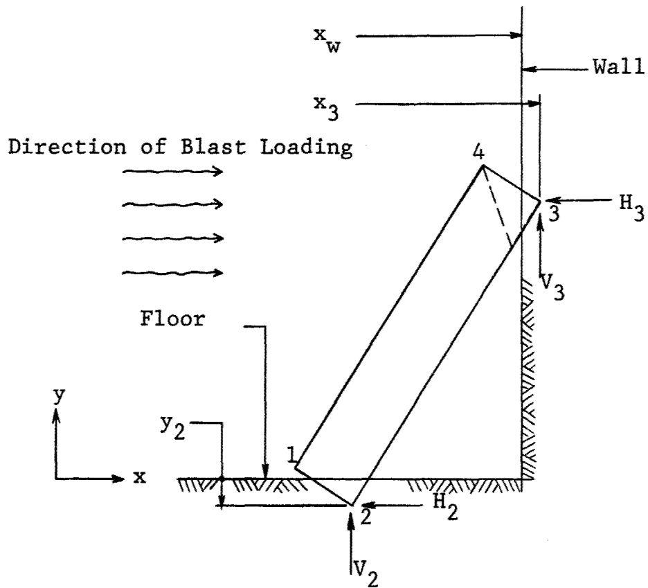
a) Example of Contact Force Designation
