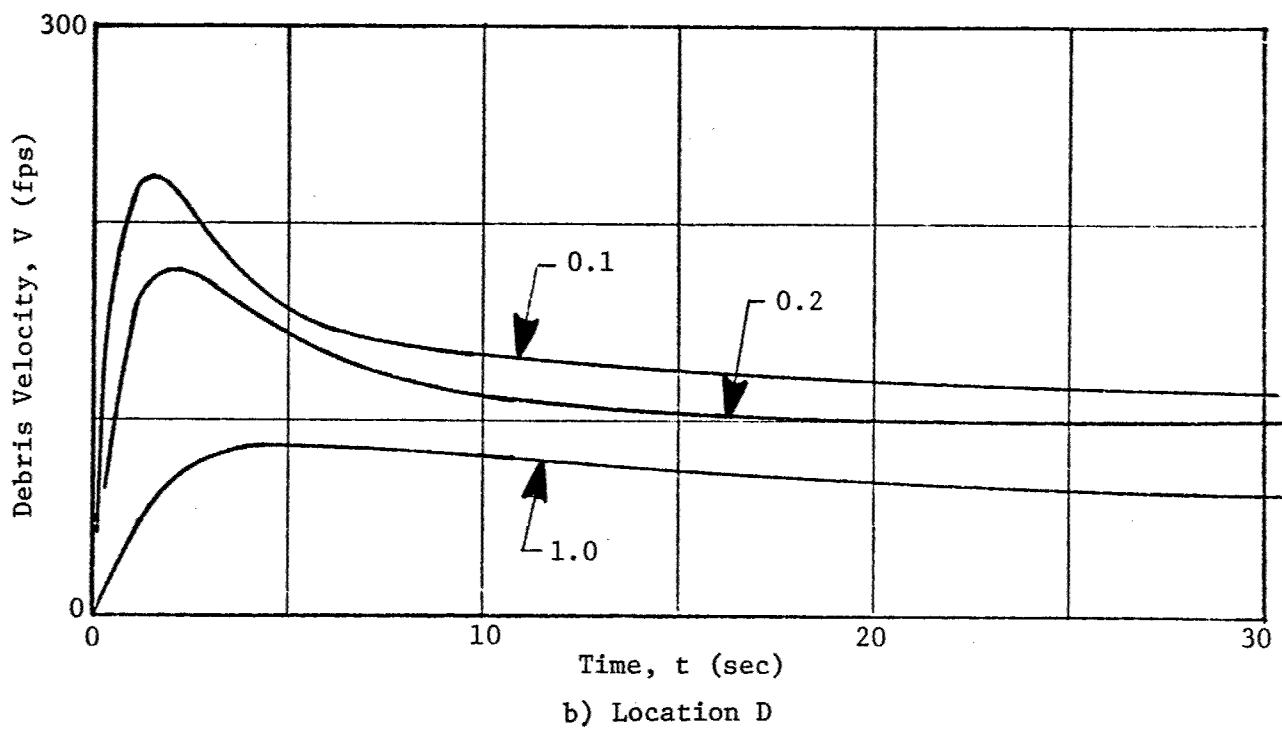
Figure 52 Influence of Ballistic Weight on Velocity Histories
