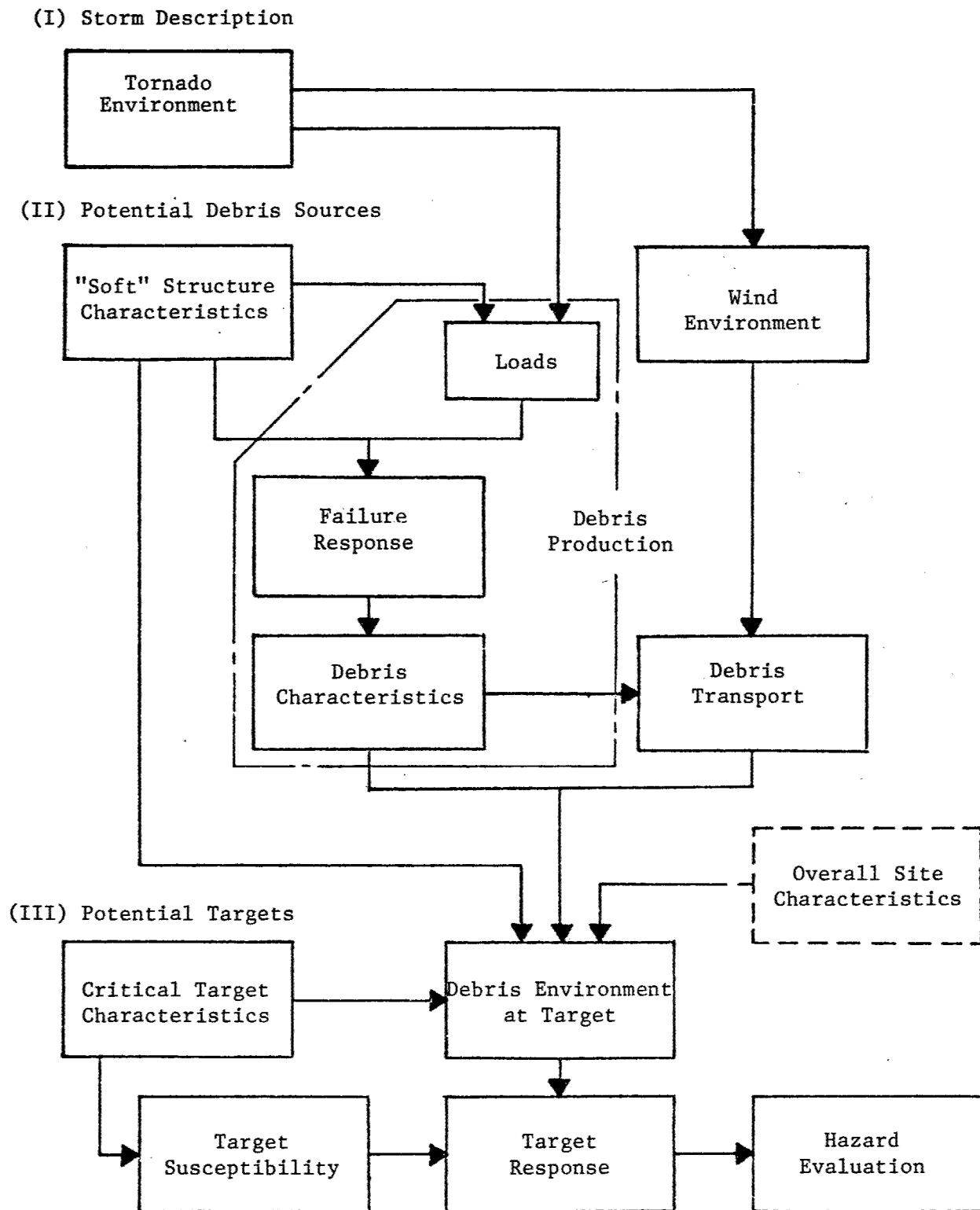
Figure 41 Activity Sequence for Evaluating Debris Hazard Resulting from a Tornado Exposure
