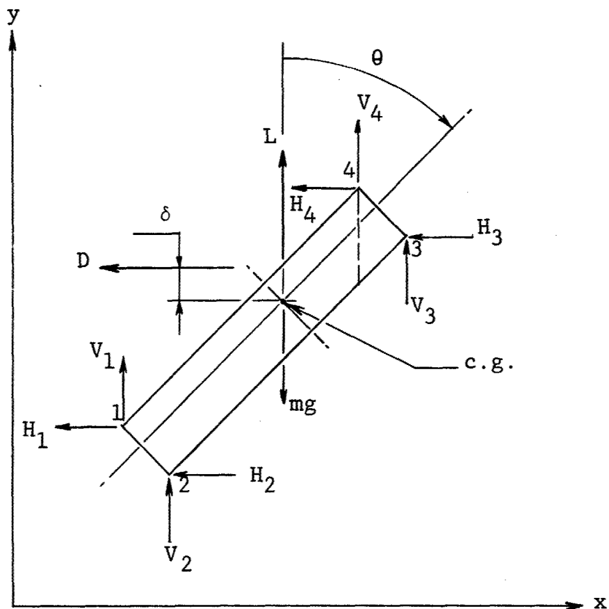
b) Lift, Drag and Contact Forces
