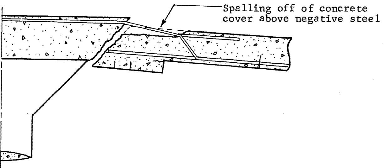
b) Shear Failure of Concrete at Incipient Collapse
