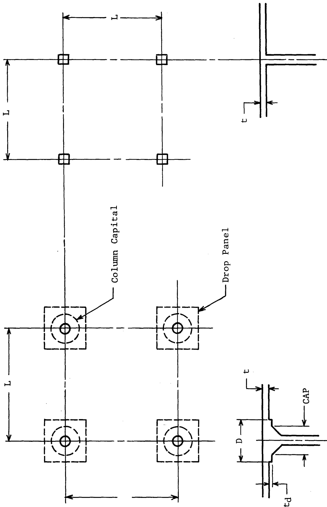
(b) Flat-Plate Floor
