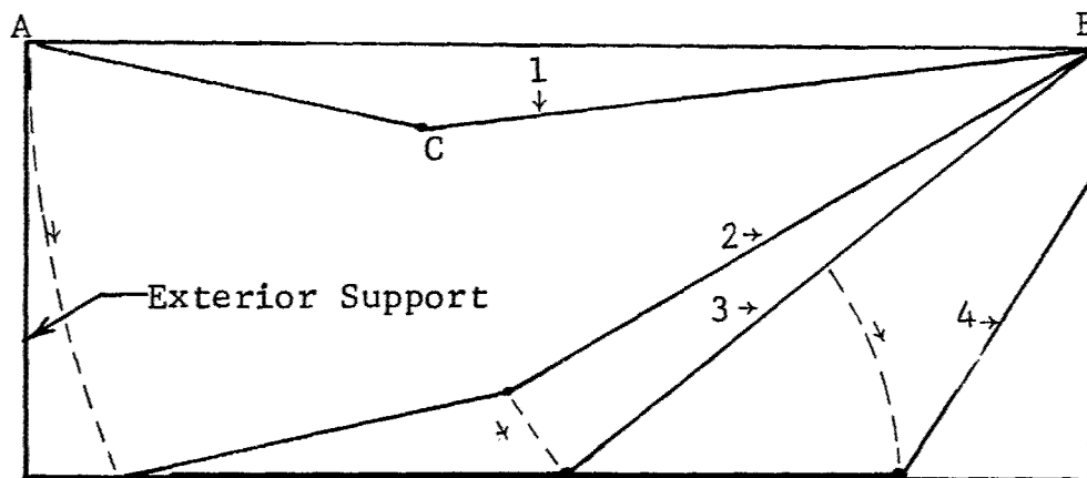
c) Collapse Mode for Two-Span Continuous Slab
