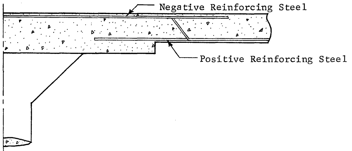
a) Initial Slab Configuration
