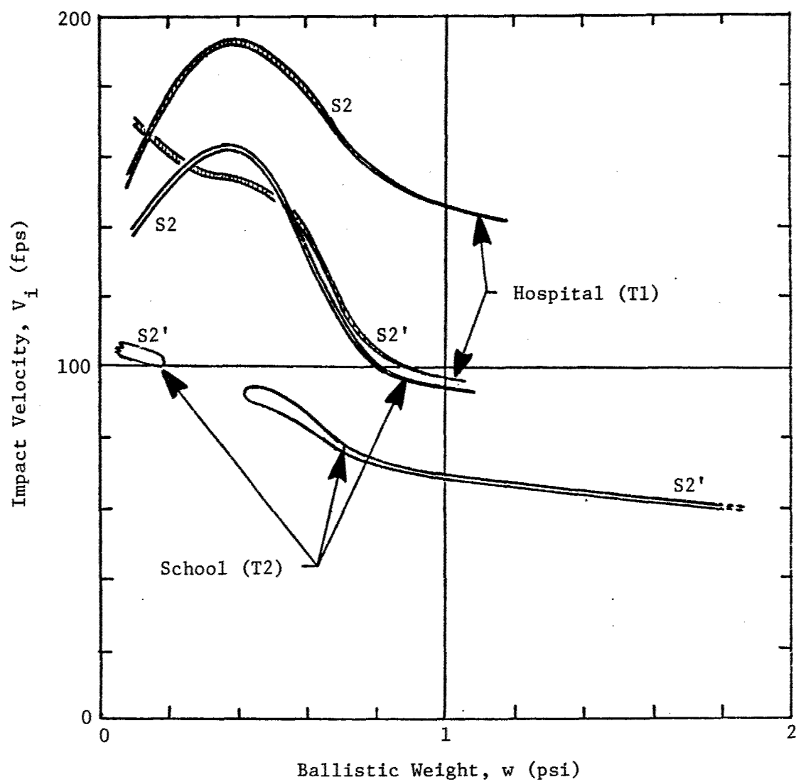
Figure 68 Impact Velocity Variations for Targets T1 and T2
