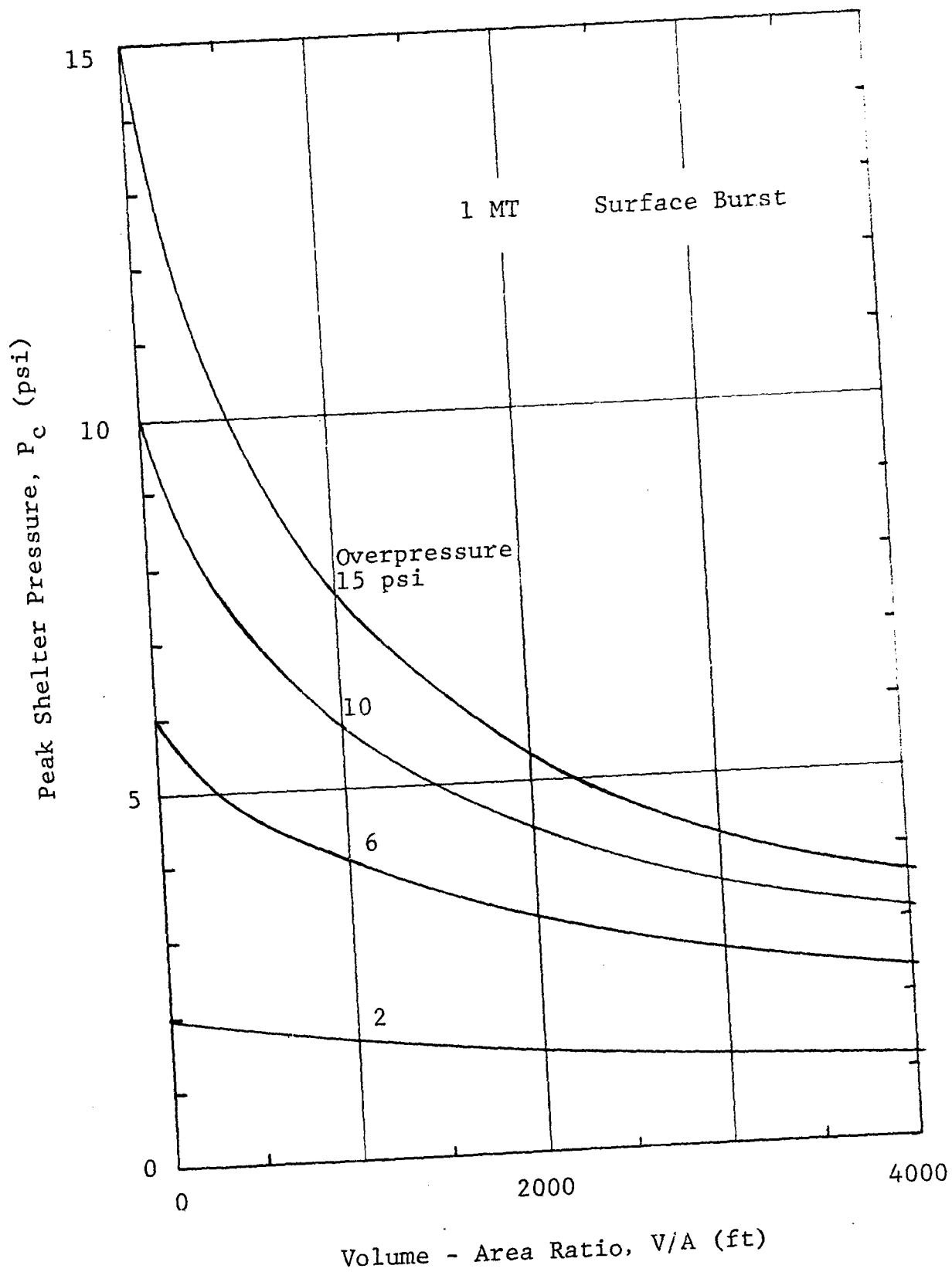
Figure 30 Peak Pressure Environment in Shelter
