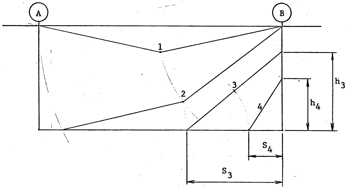
a) Unsymmetric Collapse Mode
