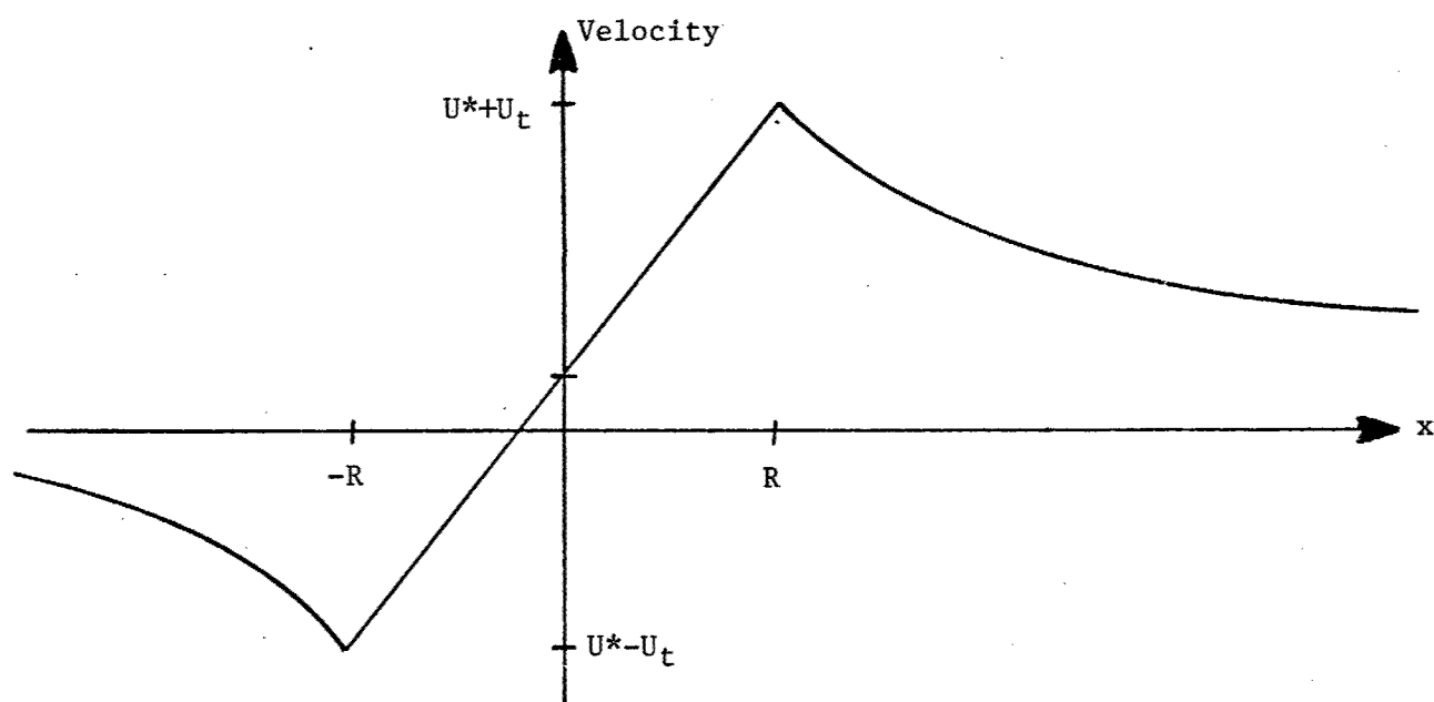
b) x-Axis Velocity Profile
