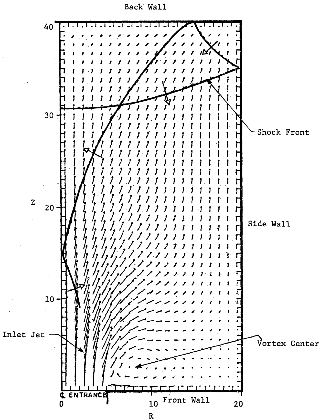
Figure 31 Velocity Diagram - Cycle 150
