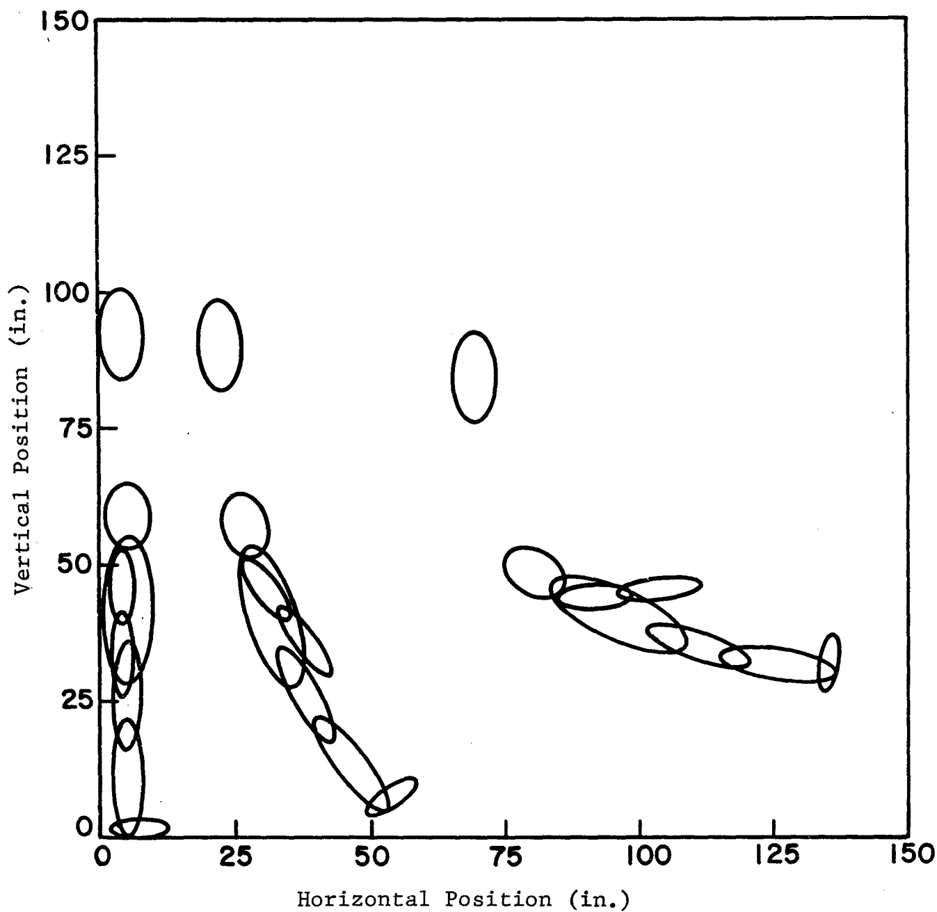
Figure 11 Blast Trajectory of Simulated Man
