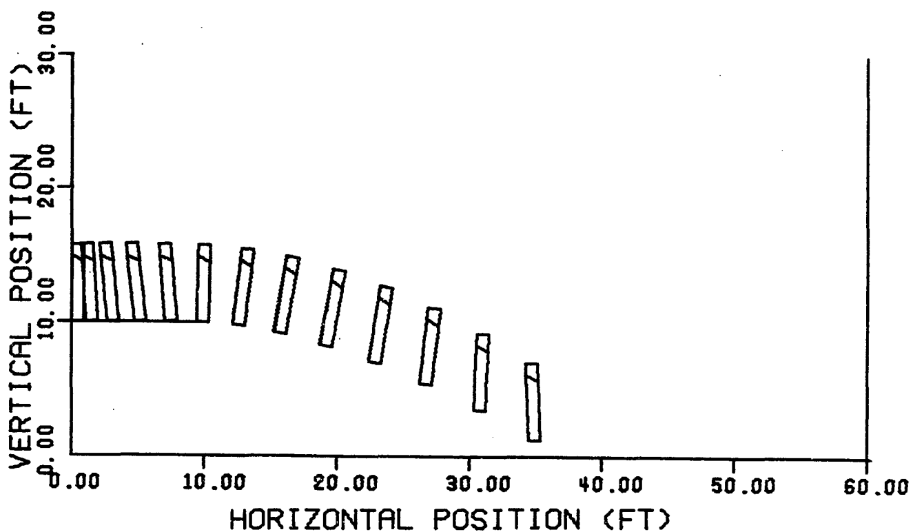
b) Free-Field Overpressure, 4 psi
