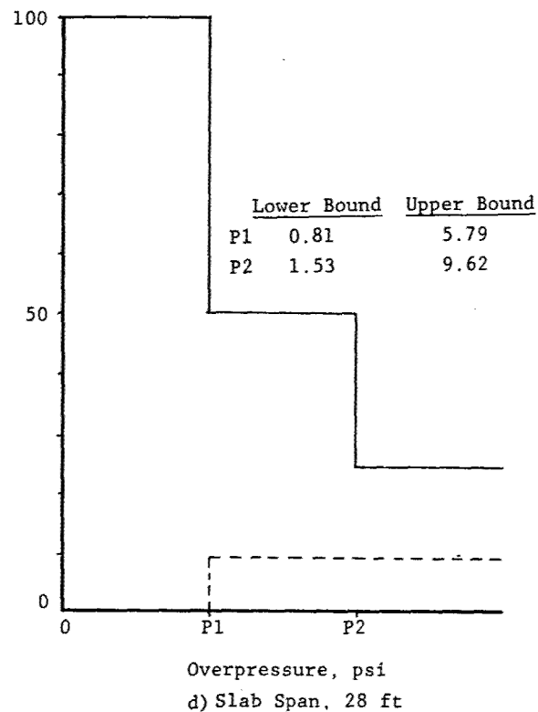
Figure 21 People Survivability Estimates for Basement Shelters With Two-Span Continuous Overhead Slabs
