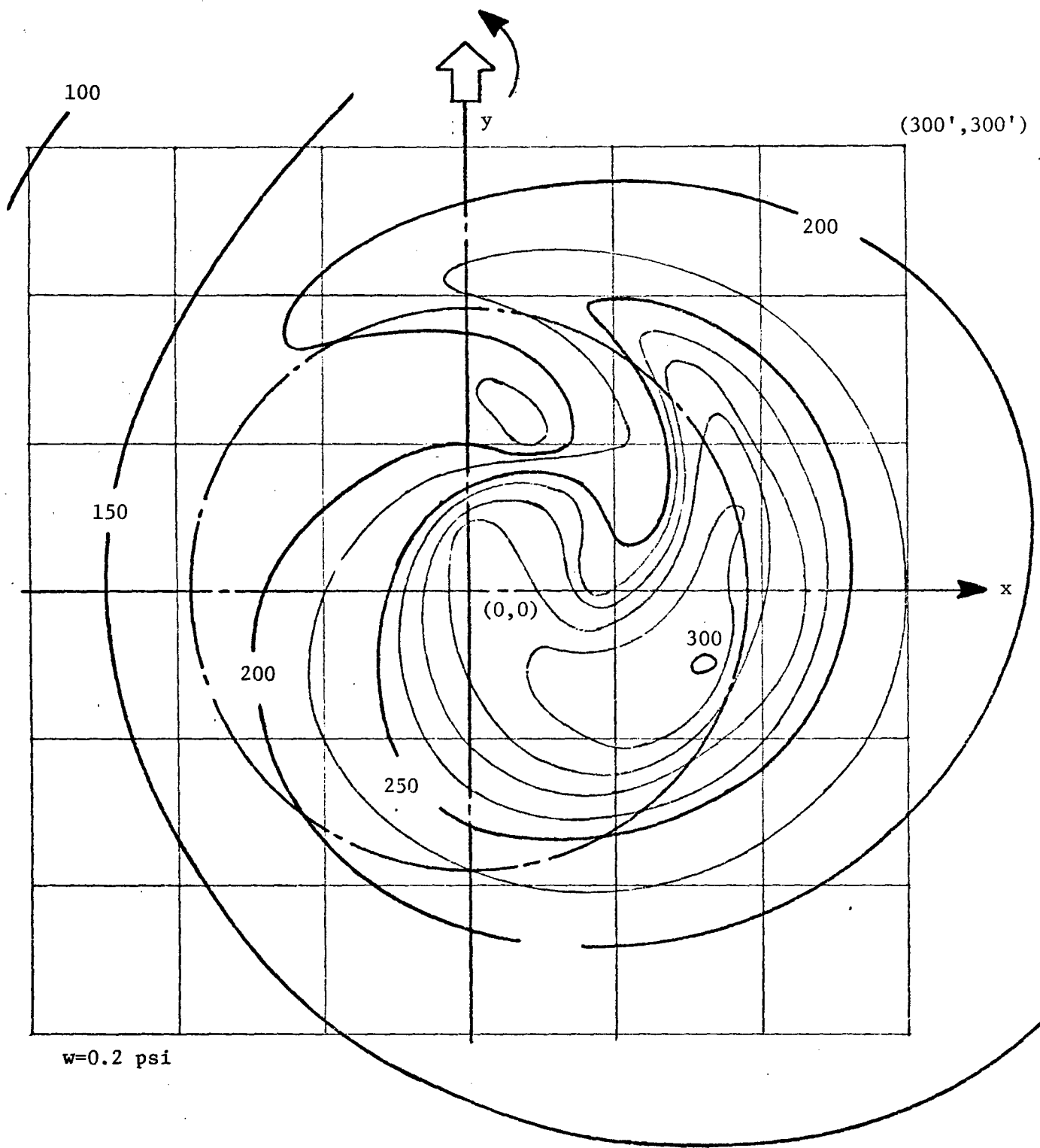
Figure 57 Influence of Release Point on Maximum Debris Velocity
