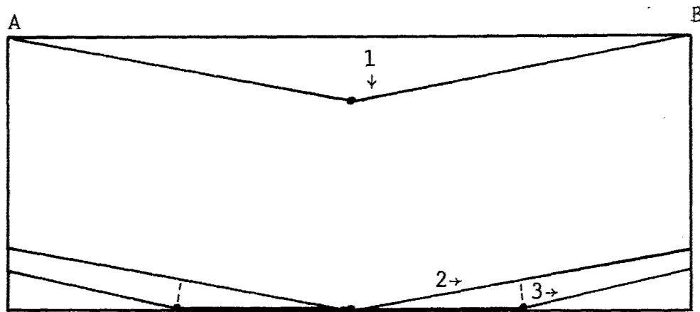
a) Symmetric Collapse Mode for Simply-Supported Slab
