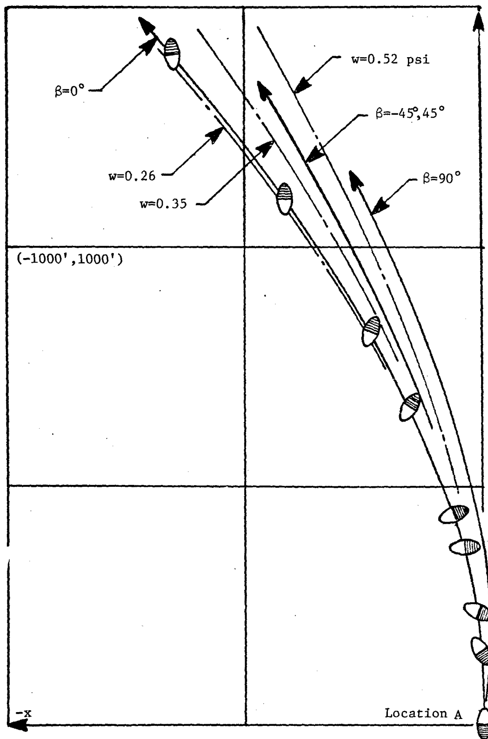
Figure 58 Trajectories of Rotating Debris - S = 0.5
