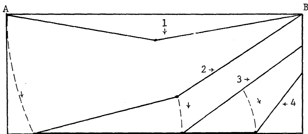
b) Unsymmetric Collapse Mode for Simply-Supported Slab
