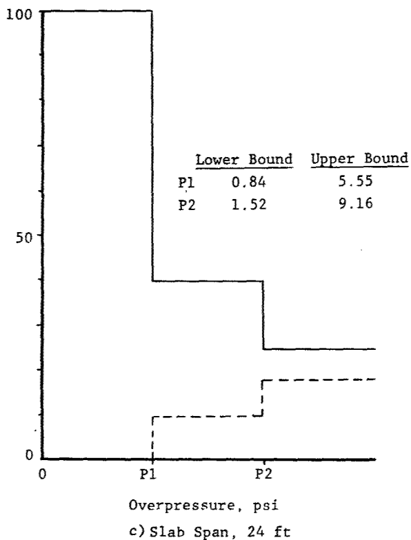
Figure 21 People Survivability Estimates for Basement Shelters With Two-Span Continuous Overhead Slabs
