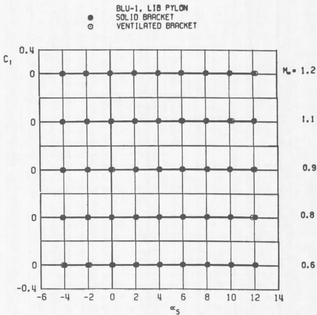
Figure 19. Effect on rolling-moment coefficient of a ventilated bracket supporting the BLU-1.
