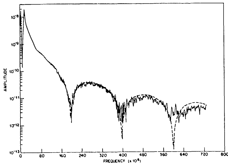
Figure 10. Analytic transform of Mimipulse (dotted line) and FLAT of digitized Mimipulse 2048 point interpolated array (solid line).
