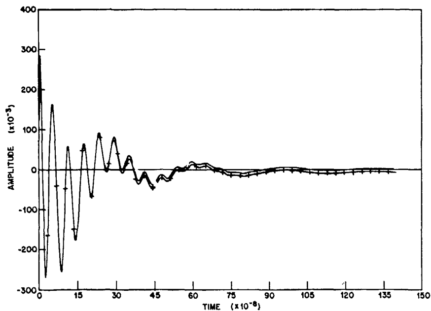
Figure 20. Mimipulse (solid line) and single aliased FFT of analytic transform of Mimipulse for 1024 points (crossed line).
