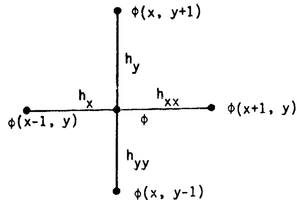
FIGURE B-2. IRREGULAR STAR IN TWO DIMENSIONAL CARTESIAN CO-ORDINATES
