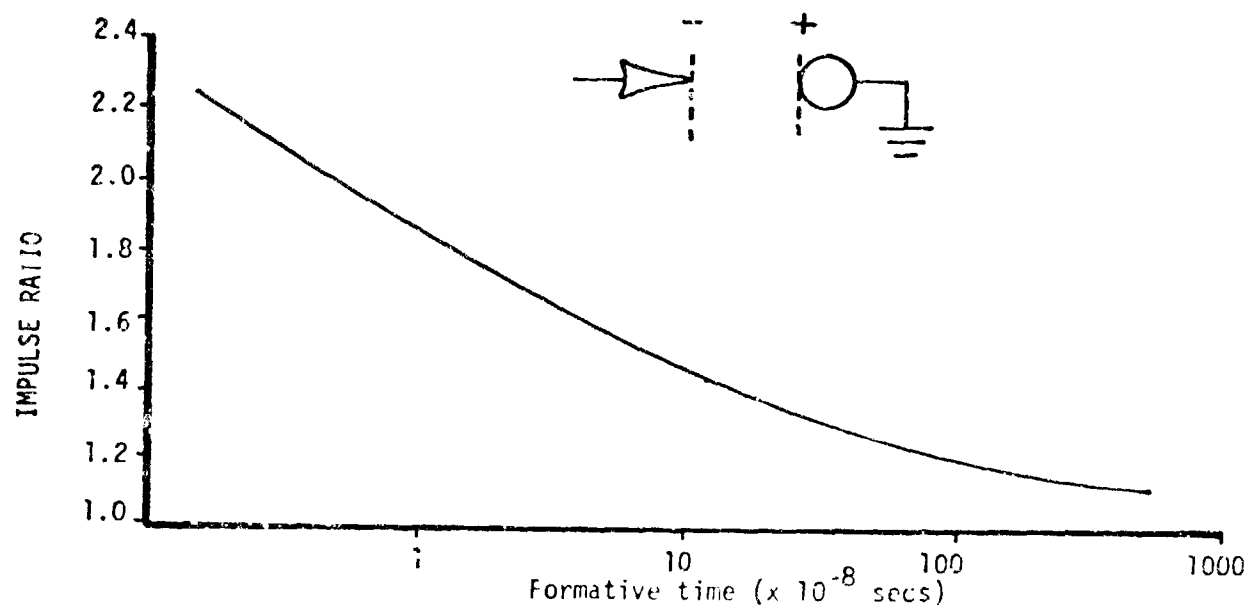
FIGURE 13. RELATION BETWEEN FORMATIVE TIME AND IMPULSE RATIO FOR VARIOUS GAP LENGTHS AND GAS PRESSURE IN A NEGATIVE POINT-SPHERE GAP IN AIR.
