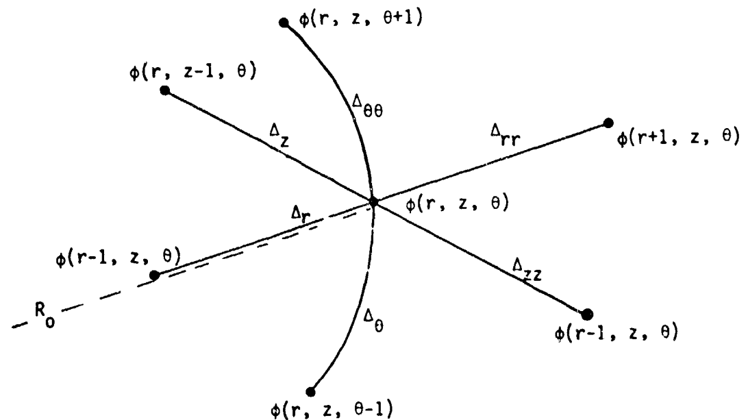
FIGURE B-4. IRREGULAR STAR IN CIRCULAR CYLINDRICAL CO-ORDINATES
