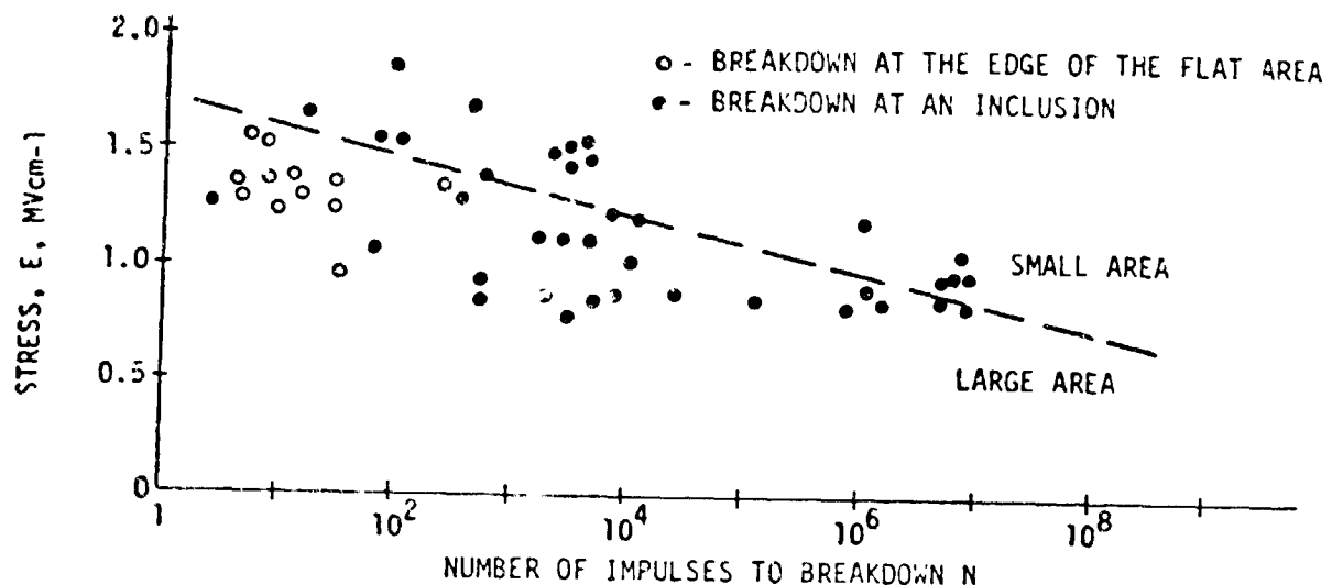
FIGURE 58. RELATION BETWEEN ELECTRICAL STRESS AND NUMBER OF IMPULSES REQUIRED TO PRODUCE BREAKDOWN WITH 1/50 MICROSECOND IMPULSES
