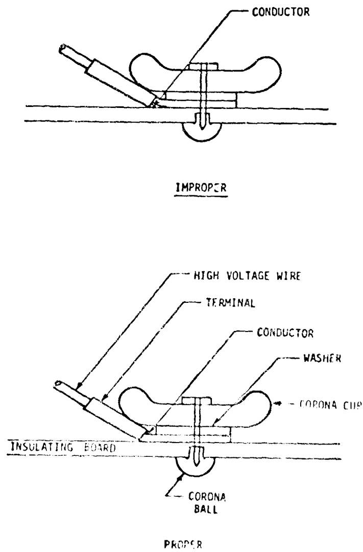
FIGURE 52. HIGH VOLTAGE TERMINALS
