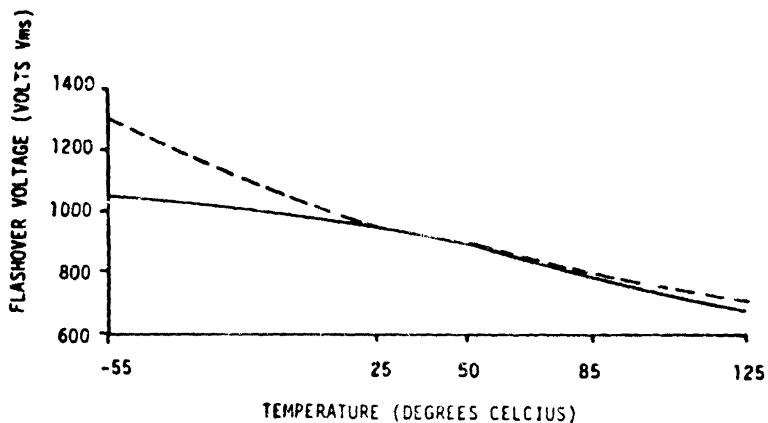
FIGURE 31. EFFECT OF TEMPERATURE ON 60 Hz FLASHOVER STRESS
