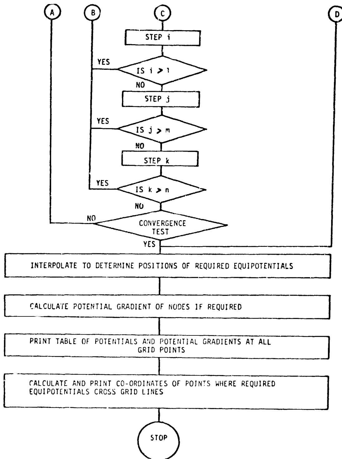
FIGURE B-5. COMPUTER PROGRAM FLOW CHART (Continued)
