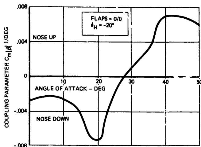
FIGURE 11. VARIATION IN PITCHING MOMENT DUE TO SIDESLIP WITH ANGLE OF ATTACK
