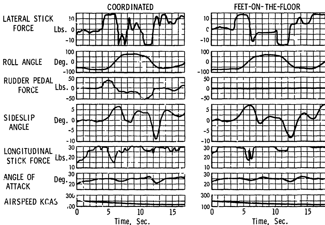
Figure 9 Roll Reversals
