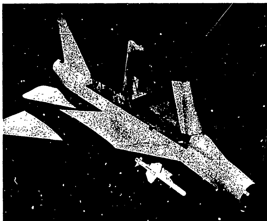
LIGHTNING MK 6 HELICOPTER DROP MODEL
