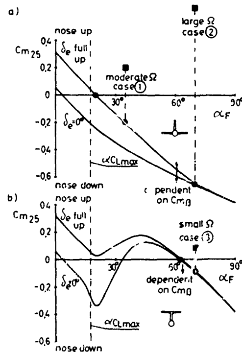
Figure 8: Balance of aerodynamic (⊗) and gyroscopic moments (⊠) about the Y axis for typical spins a) with conventional longitudinal characteristics "steep" with satisfactory yaw damping ① and "flat" with insufficient yaw damping ② (see fig. 9) b) flat with super-stall characteristics ③
