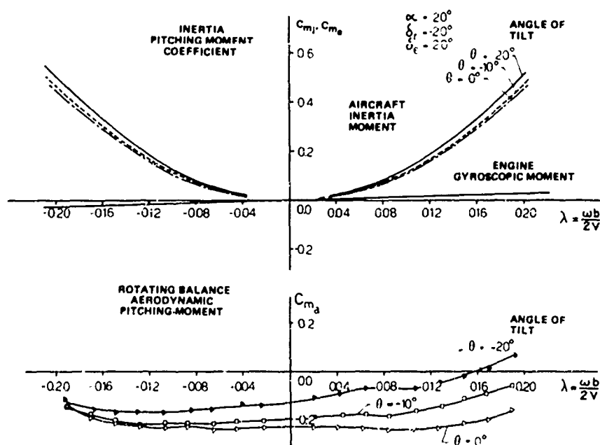
FIGURE 15. LONGITUDINAL (PITCHING) MOMENT COEFFICIENTS
