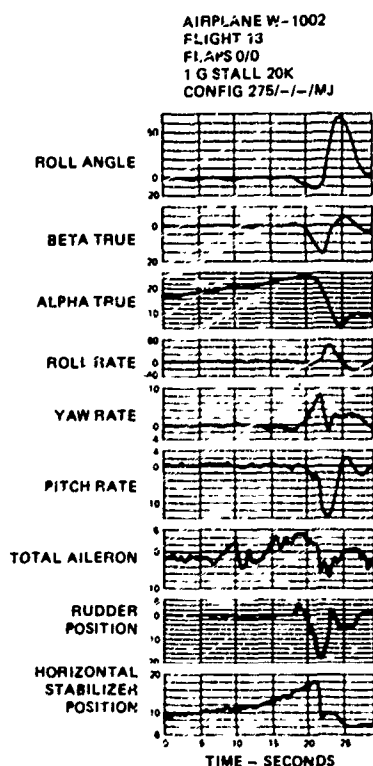
FIGURE 25. BASELINE CONFIGURATION
