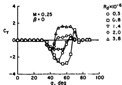
Fig. 16-7 Effect of Reynolds number on side-force curves for z/d = 3.5 pointed tangent ogive.
