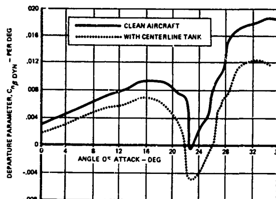
FIGURE 18. EFFECT OF CENTERLINE TANK ON F-5E DEPARTURE PARAMETER (MISSILES)
