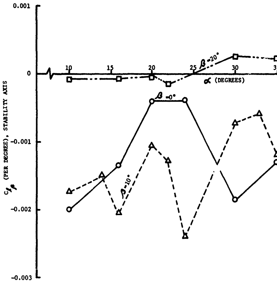
FIGURE 3 C_{l\beta}(\alpha) AT \beta = 0^\circ, 10^\circ, \text{ AND } 20^\circ
