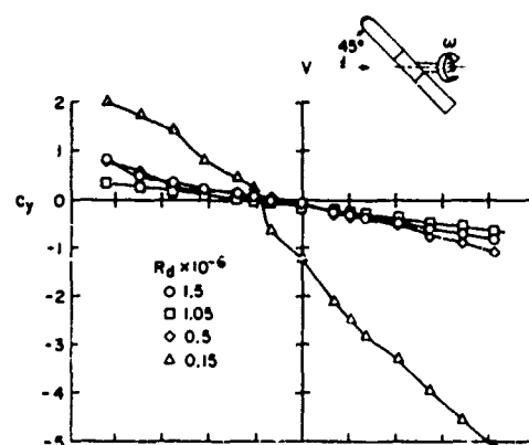
Fig. 16-13 Effect of Reynolds number and spin rate on side force for l/d = 3.5 pointed tangent ogive.
