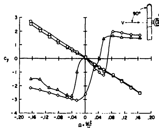
Fig. 16-16 Effect of Reynolds number and angle of attack on nose section side force in spin motion.
