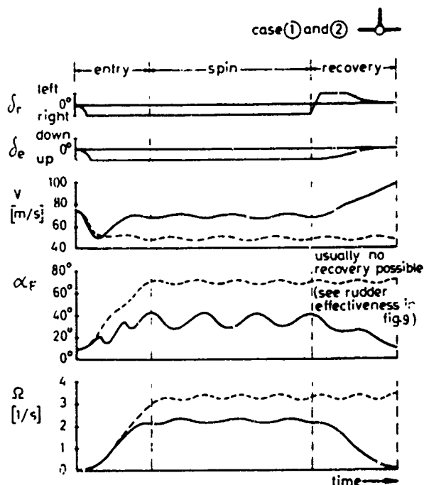
Figure 6: Development of spin with conventional longitudinal characteristics; \delta_a=0^\circ — "steep" with satisfactory yaw damping and --- "flat" with insufficient yaw damping beyond \alpha_{CL \max} (see fig.5)
