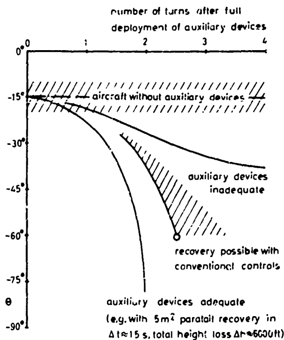
Figure 12: Development of spin recovery using auxiliary devices, for nose-down pitching moment; flat spin case (3) (for all initial control and flap deflections)
