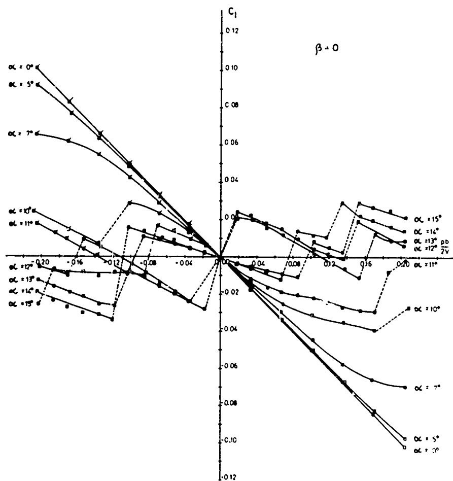
FIGURE 11. INFLUENCE OF STALL PROPAGATION ON ROLL DAMPING
