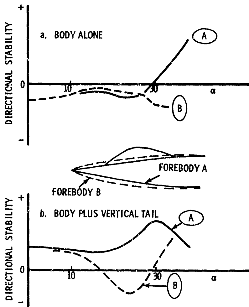
FIGURE 4- EFFECT OF FOREBODY (REF. 17)
