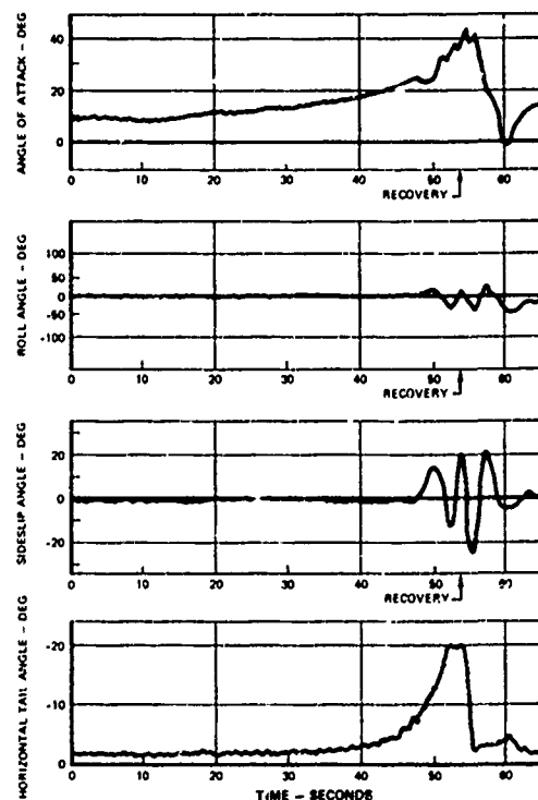
FIGURE 14. EXAMPLE OF SIDESLIP/ANGLE-OF-ATTACK COUPLING
