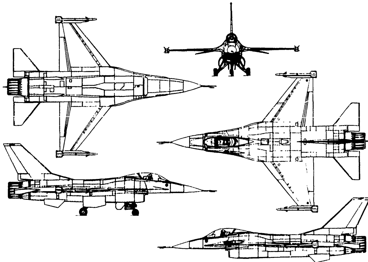
Figure 1 YF-16
