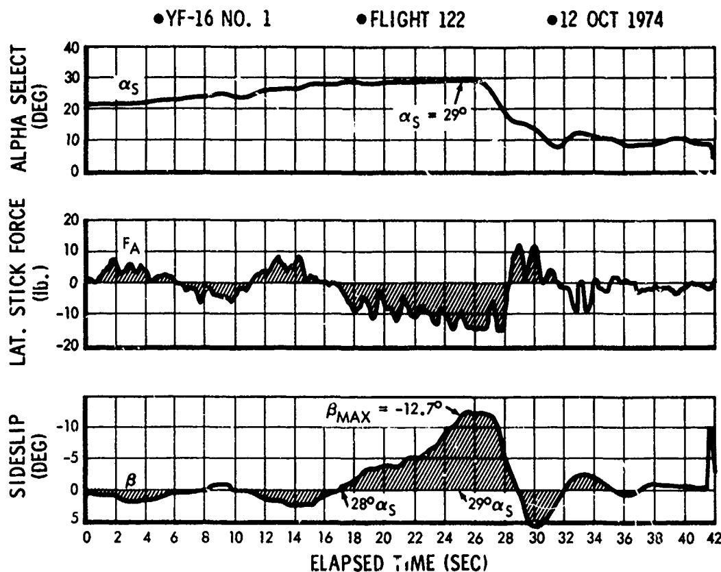
Figure 6 1g Deceleration
