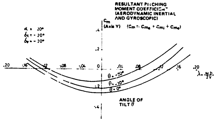
FIGURE 16. RESULTANT PITCHING MOMENT COEFFICIENT
