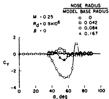
Fig. 16-9 Effect of nose bluntness on side force for z/d = 3.5 pointed tangent ogive.
