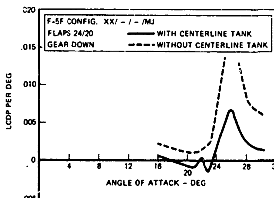
FIGURE 9. LATERAL CONTROL DEPARTURE PARAMETER VS ANGLE OF ATTACK, F-5F WITH MISSILES
