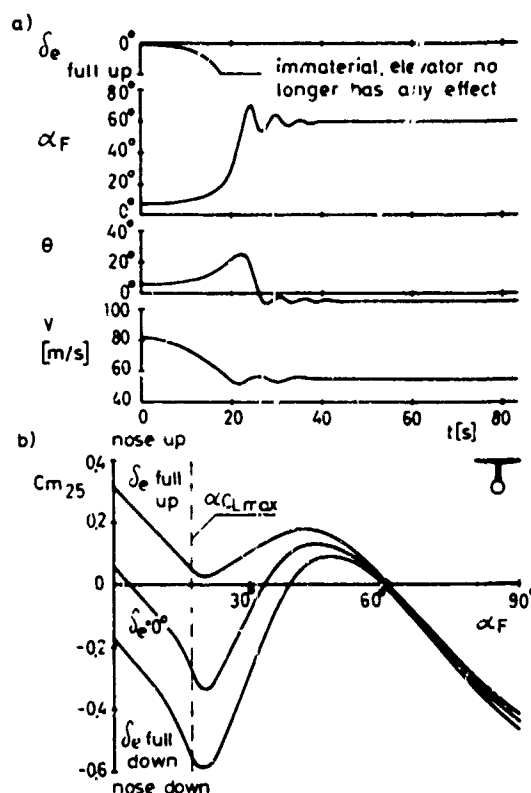
Figure 4: a) Development of a super-stall ( \delta_a, \delta_r, \beta=0^\circ ) and b) super-stall characteristics
