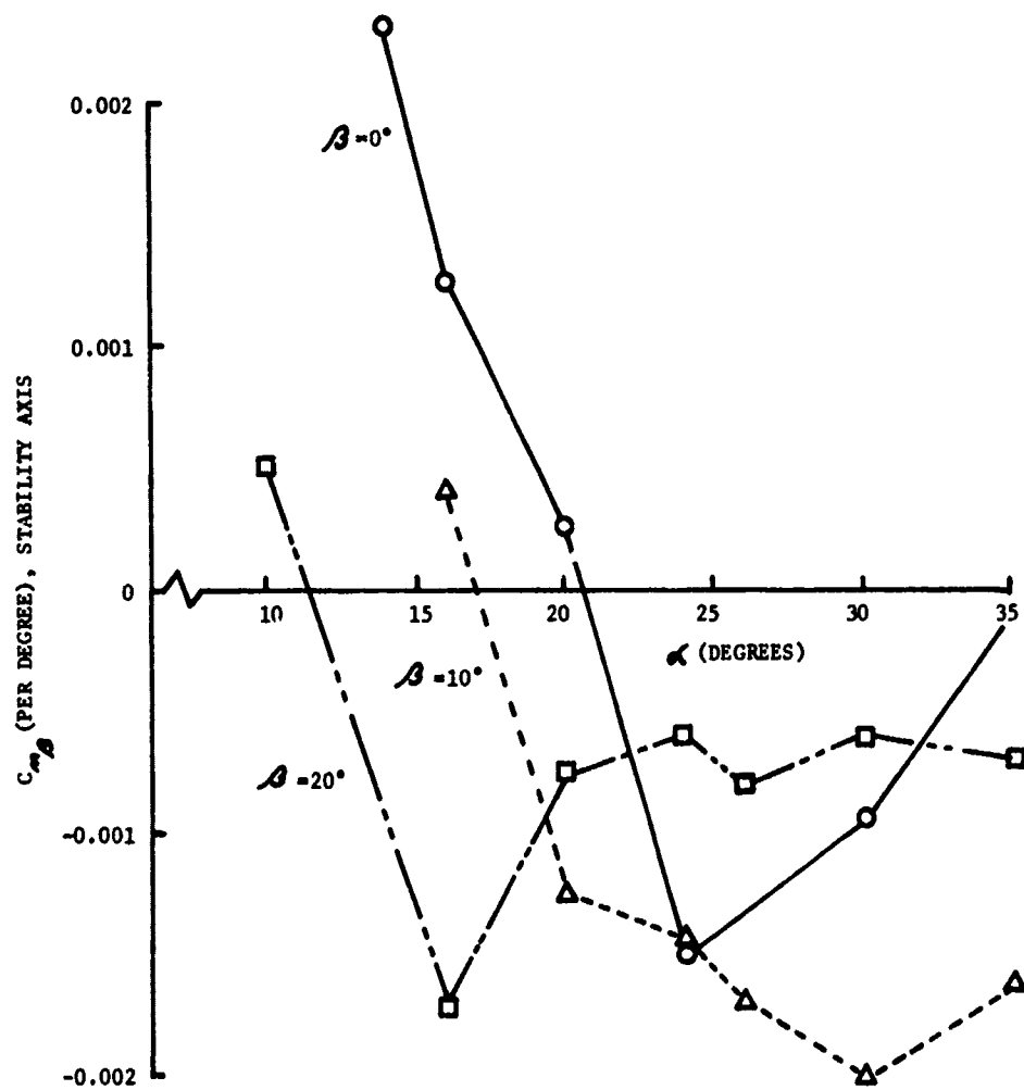
FIGURE 2 C_{m\alpha}(\alpha) AT \beta = 0^\circ, 10^\circ , AND 20^\circ
