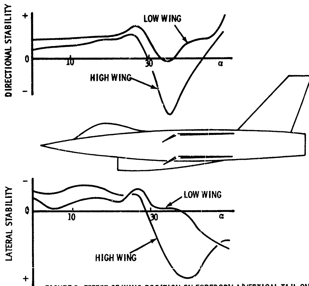
FIGURE 5- EFFECT OF WING POSITION ON FOREBODY A/VERTICAL TAIL ON AND VENTRAL INLET (REF. 17)
