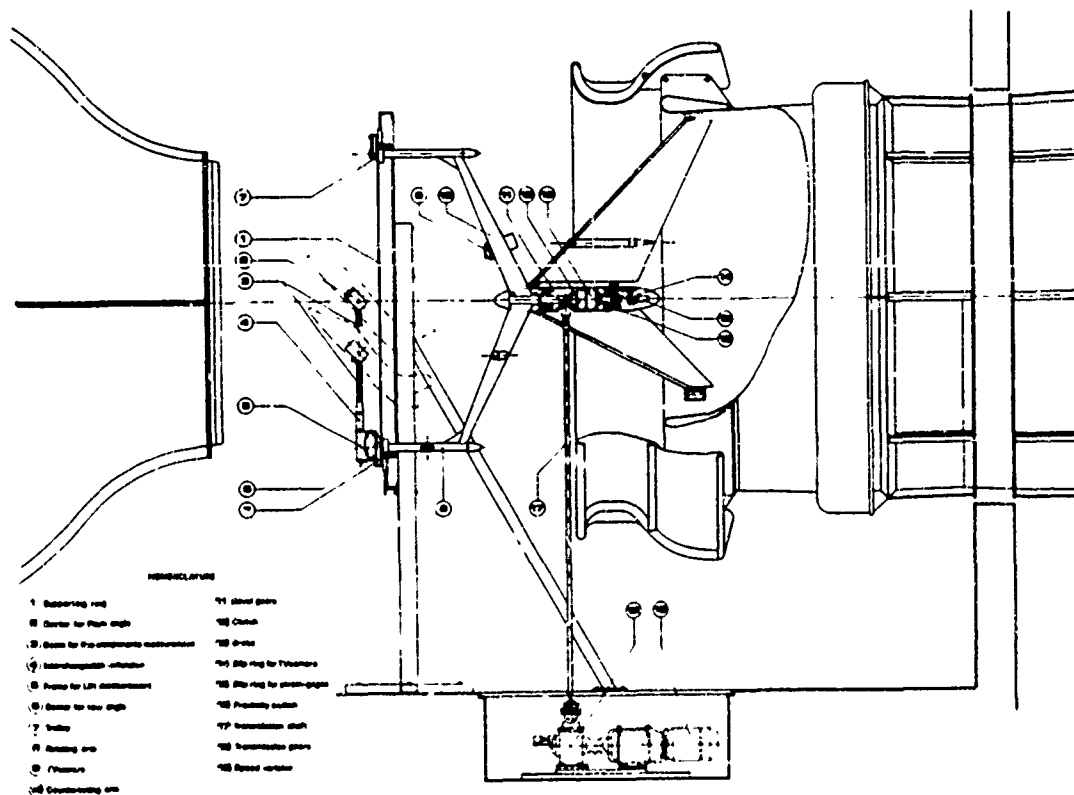
FIGURE 6. SIX-COMPONENTS BALANCE
