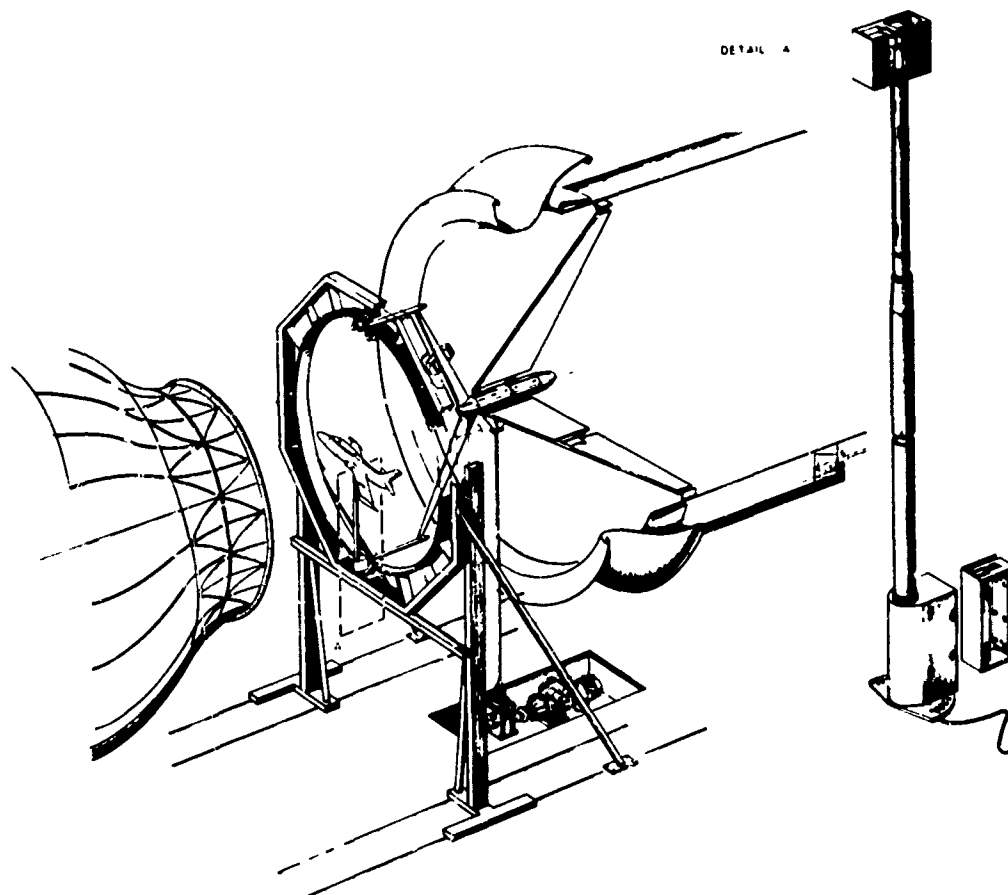
FIGURE 5. SIX-COMPONENTS BALANCE
