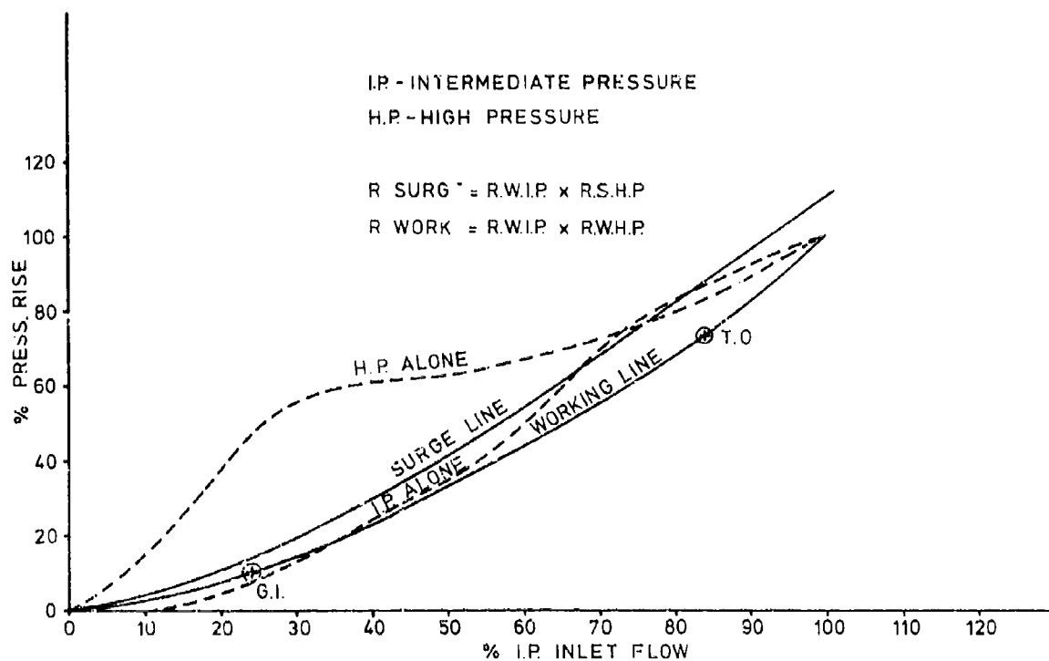
Fig.12B Performance of a twin spool multistage
