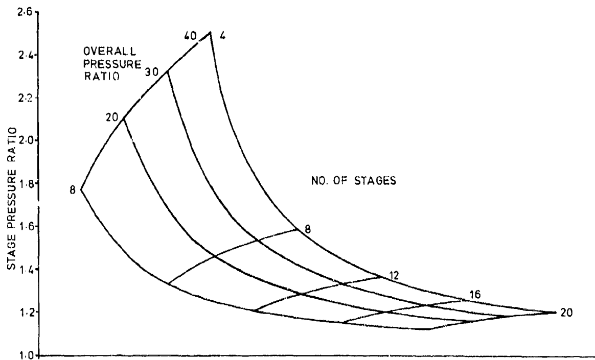
Fig. 15B Multistage performance potential
