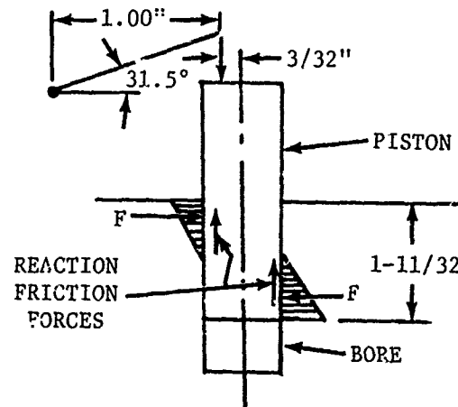
Figure A-1 Piston Loads
