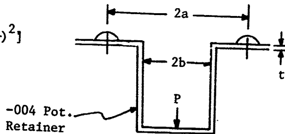
Figure A-11. Potentiometer Holder
