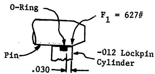
Figure A-7C. Pin Reaction
