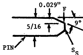
Figure A-7B. Pin Tip
