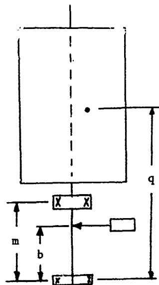
Figure A-12 Bearing Loads
