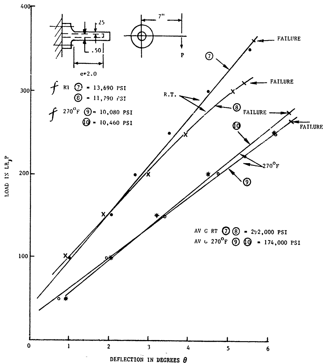
Figure 4. 5504 Polyimide Load Deflection Curve at R.T. and at 270°F in Torsion
