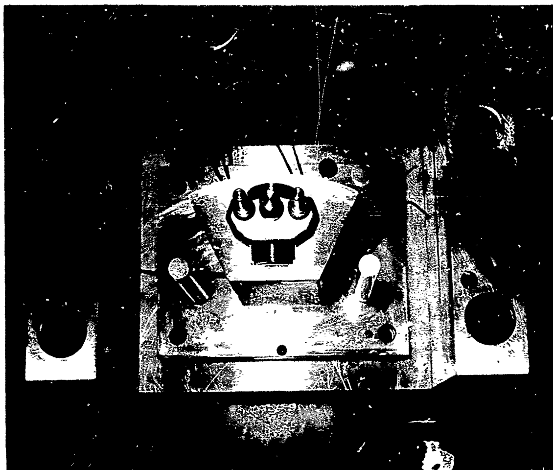
Figure 18. Punch
