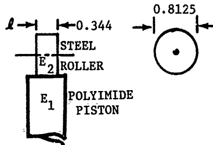
Figure A-5 Roller Forces
