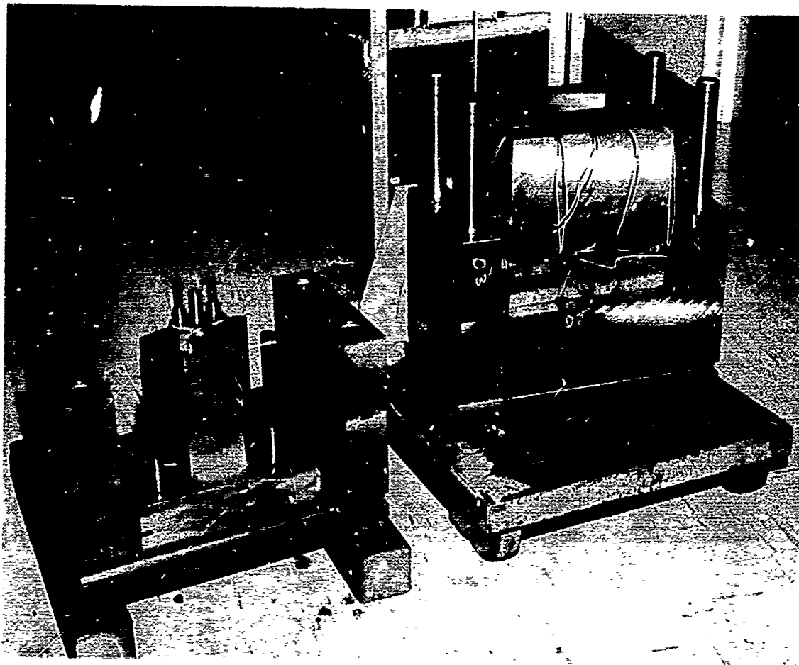
Figure 16. Mold Parts
