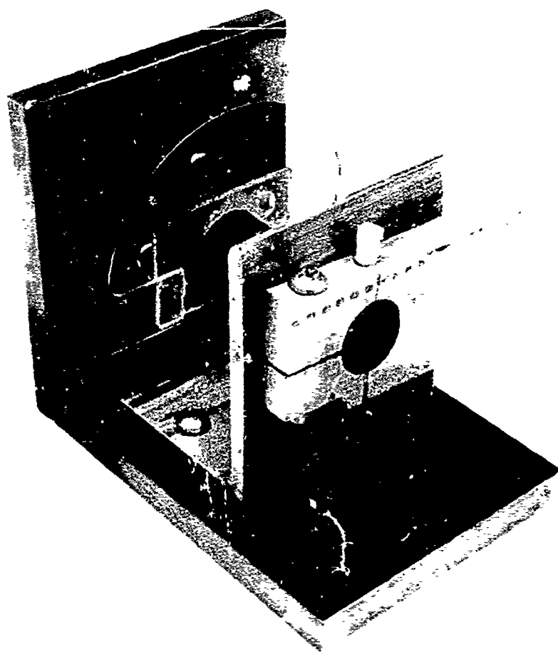
Figure 3. Torsion Test Fixture
