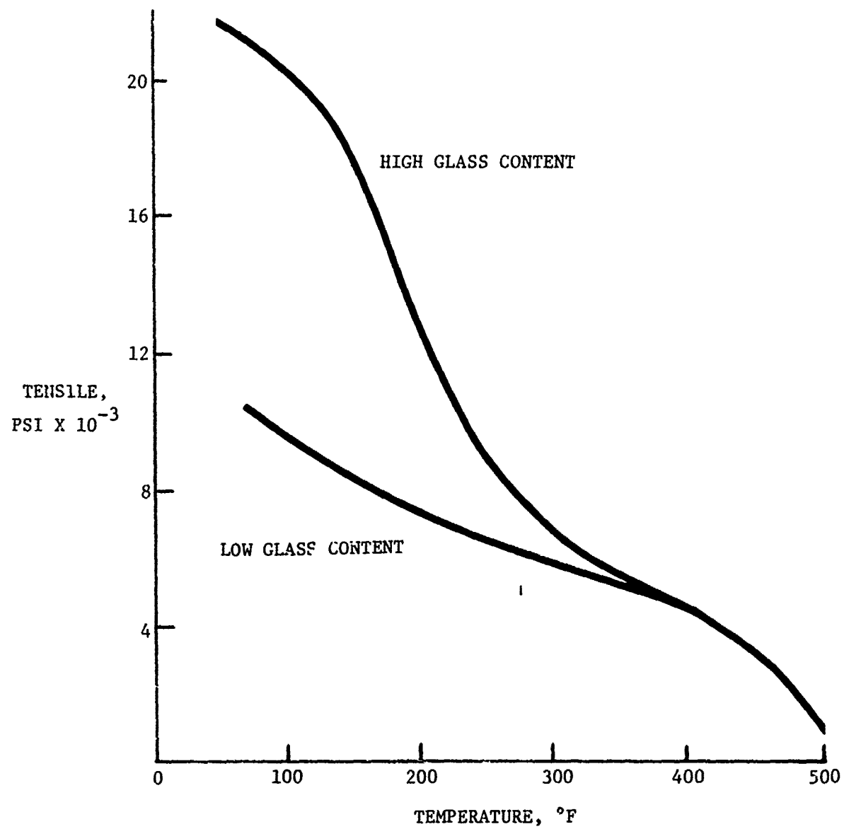
Figure 1. Tensile vs Temperature Polyphenylene Sulfide
