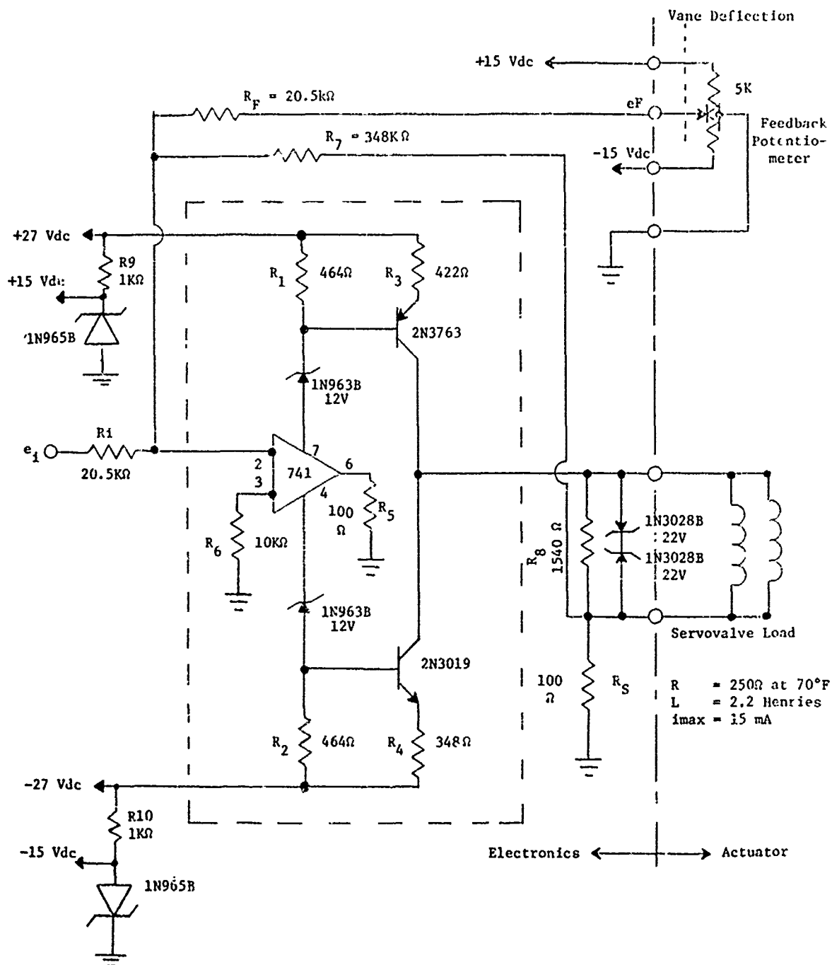
Figure 15. Electronics Schematic
