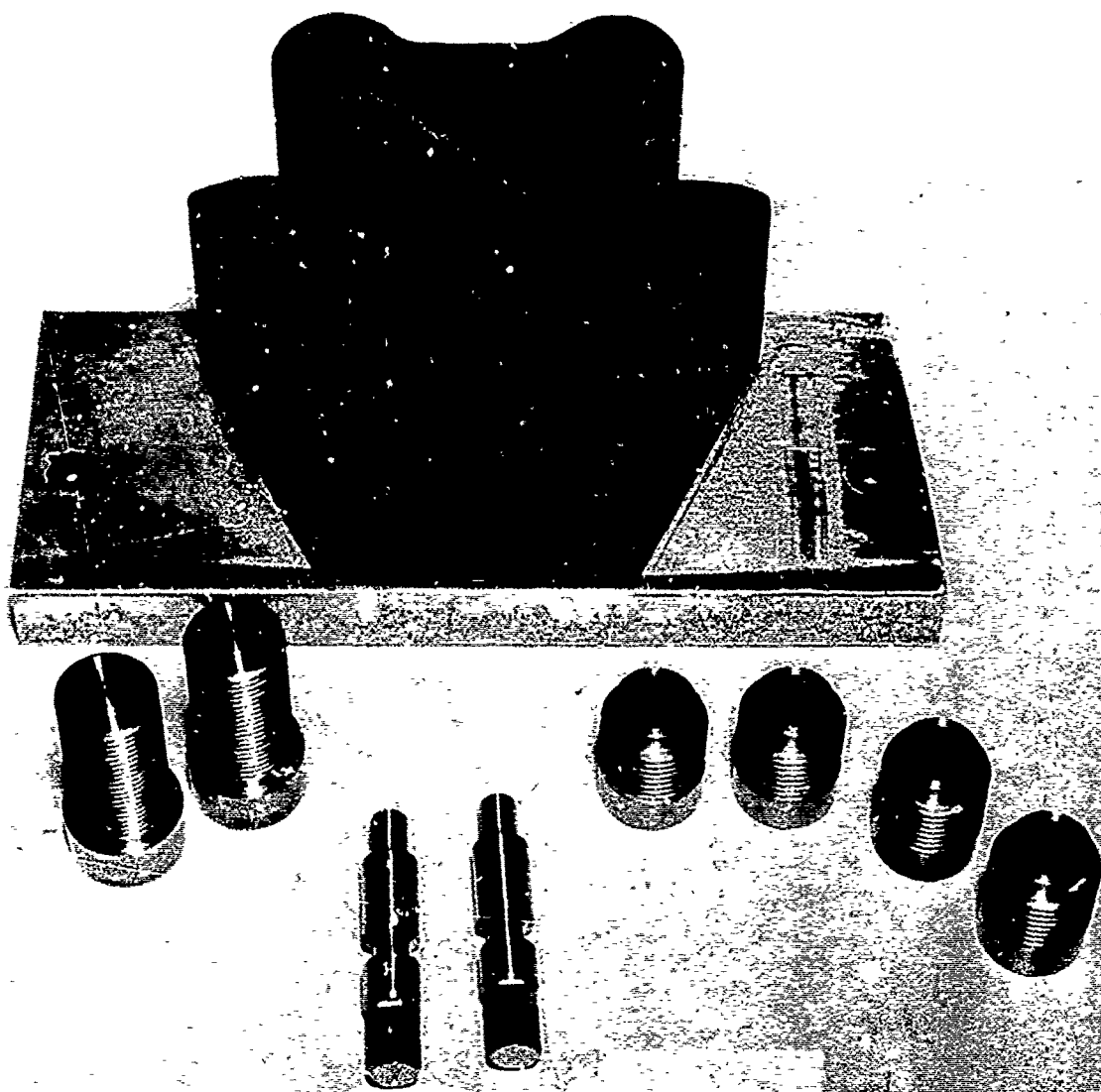
Figure 19. Mold Inserts and EDM Electrode
