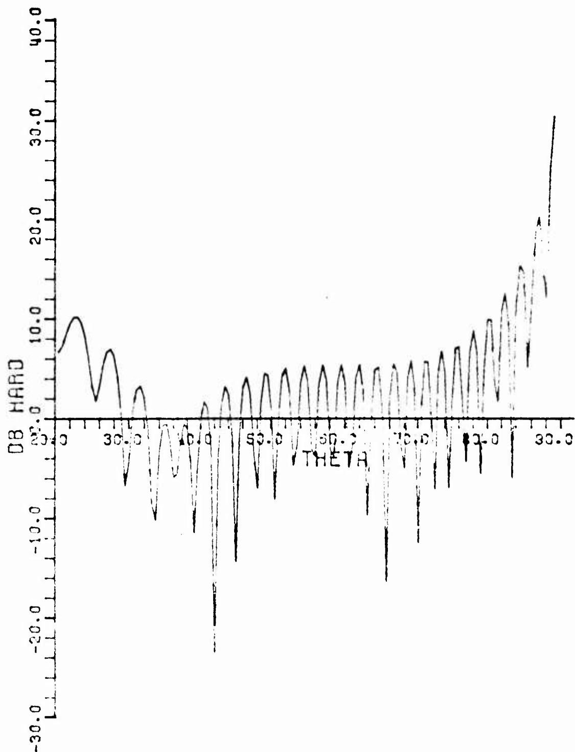
Fig. (31b). (G_h/\lambda^2) in dB vs \theta^i at f = 2 GHz, and \lambda = 1 m.
