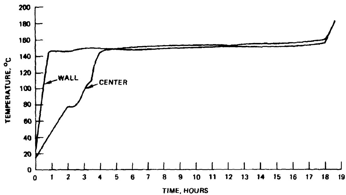
FIGURE 24. Thermocouple Data for Amatex-20K (With Ross AN/KN Prills) Tested at 150°C. (Sample 5 1/4-inch diameter by 8 inches long)
