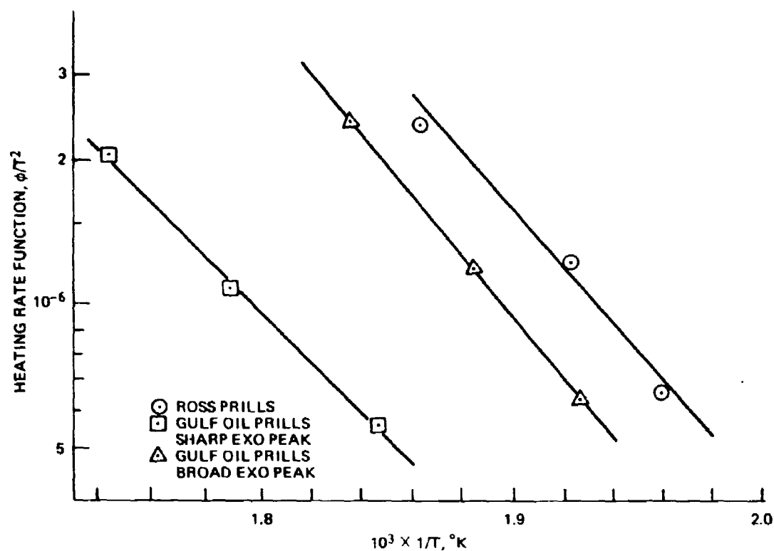
FIGURE 10. Plot of Heating Rate Function for Amatex-20K.
