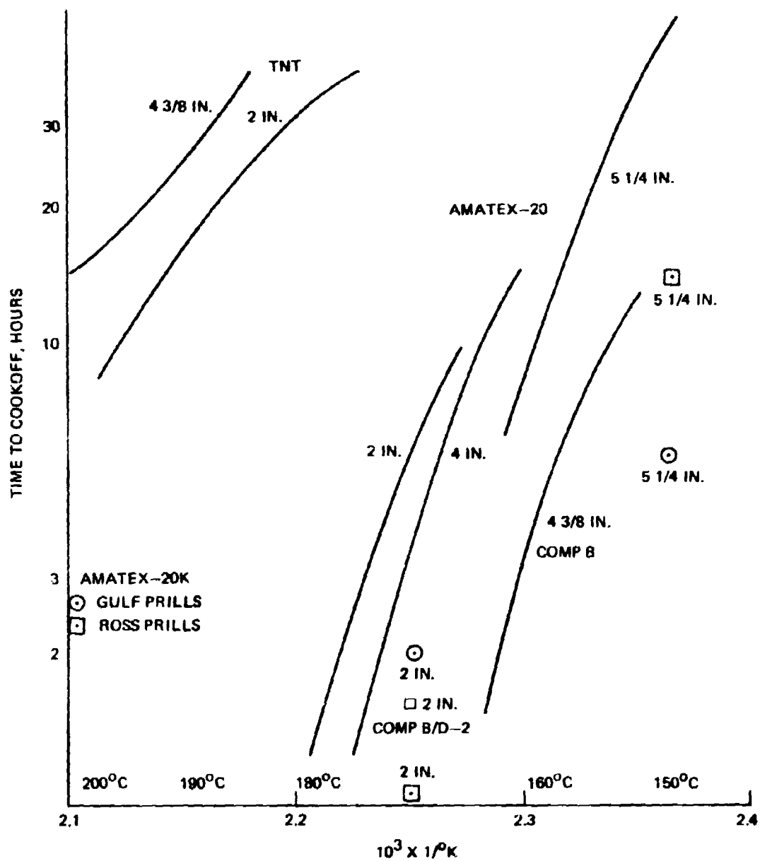
FIGURE 26. Comparison of AmateX-20K with TNT, AmateX-20, Composition B and Composition B/D-2.
