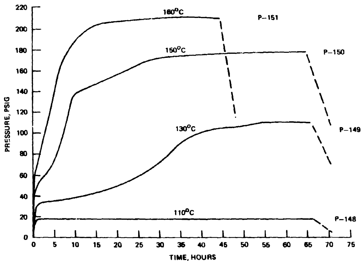
FIGURE 16. Thermal Decomposition of Amatex-20K (With Gulf AN/KN Prills).
