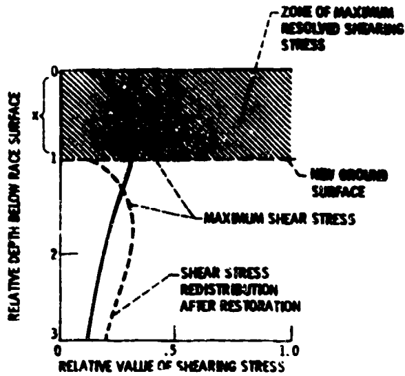
Figure 6. - Relative value of shearing stress as a function of depth below rolling-element surface.
