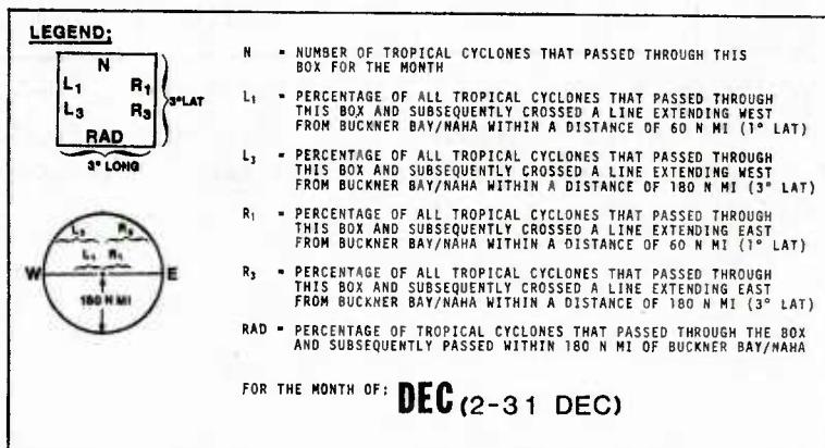
Figure 17. Statistical summary of tropical cyclones for the month of December (based on data from the years 1947-1973).
