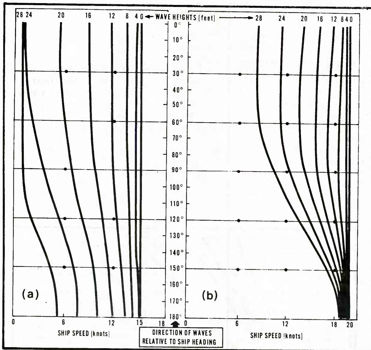
Figure E-2. Expected ship speed as a function of wave height and wave direction relative to ship's heading for (a) a ship making 15 kt and (b) a ship making 20 kt (from Nagle, 1972).
