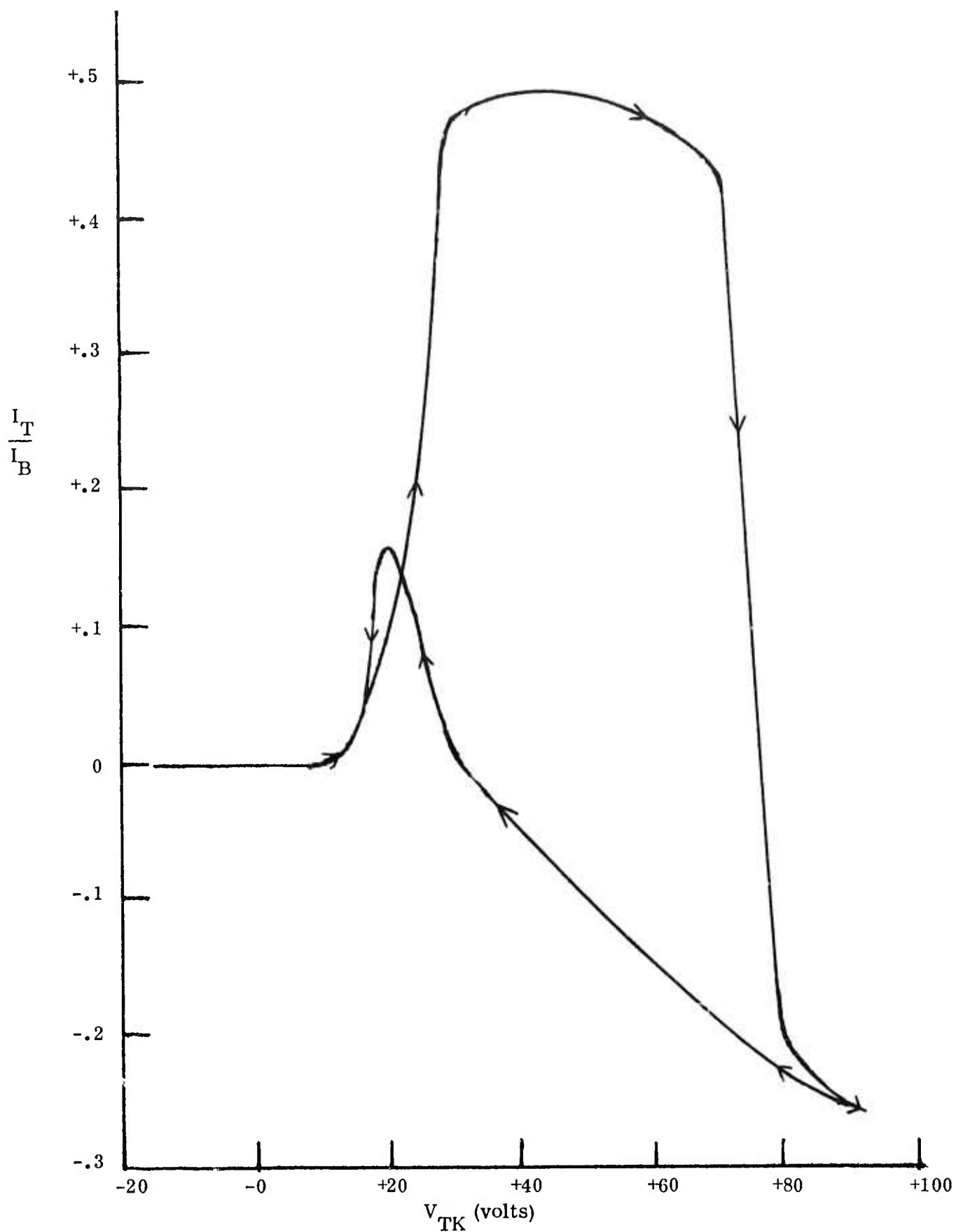
Figure 19. Normalized Target Current vs. V_{TK} (Unscanned, T = 300^\circ\text{K} )
