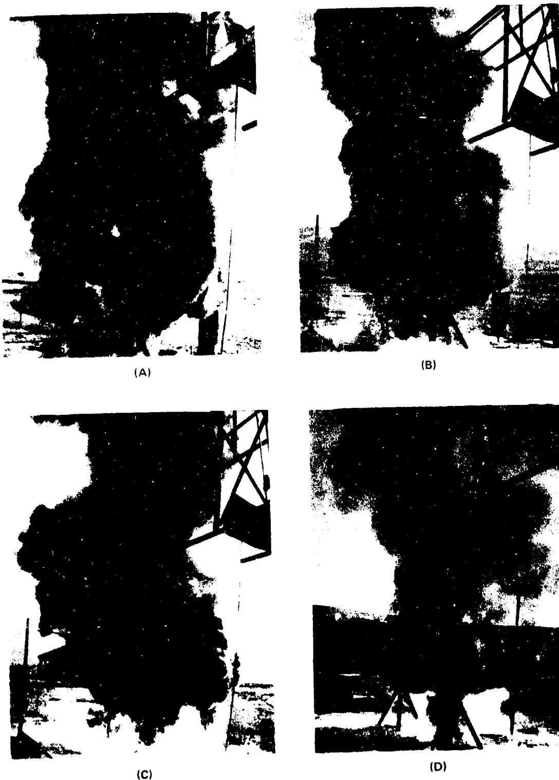
FIG. 3.5 EXTINGUISHMENT OF JP6 FIRE UNDER SIMULATED AIRCRAFT WING, i.e. TYPE 3 OBSTRUCTION TEST 26 (A) FIRE JUST BEFORE ONSET OF SUPPRESSION, (B) FIRE PERIPHERY EXTINGUISHED (C) ONLY SHADOWED AREA BURNING (D) JUST BEFORE COMPLETE EXTINGUISHMENT.
