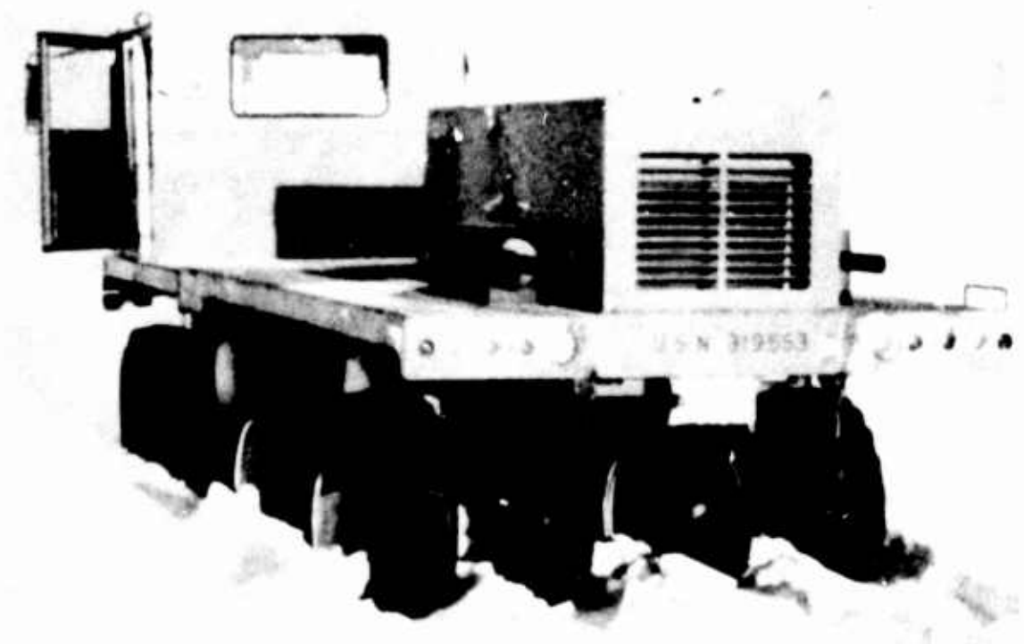
Figure 14. Testing LGPV-16 in 1974 over undisturbed snow on the Ross Ice Shelf, McMurdo, Antarctica
