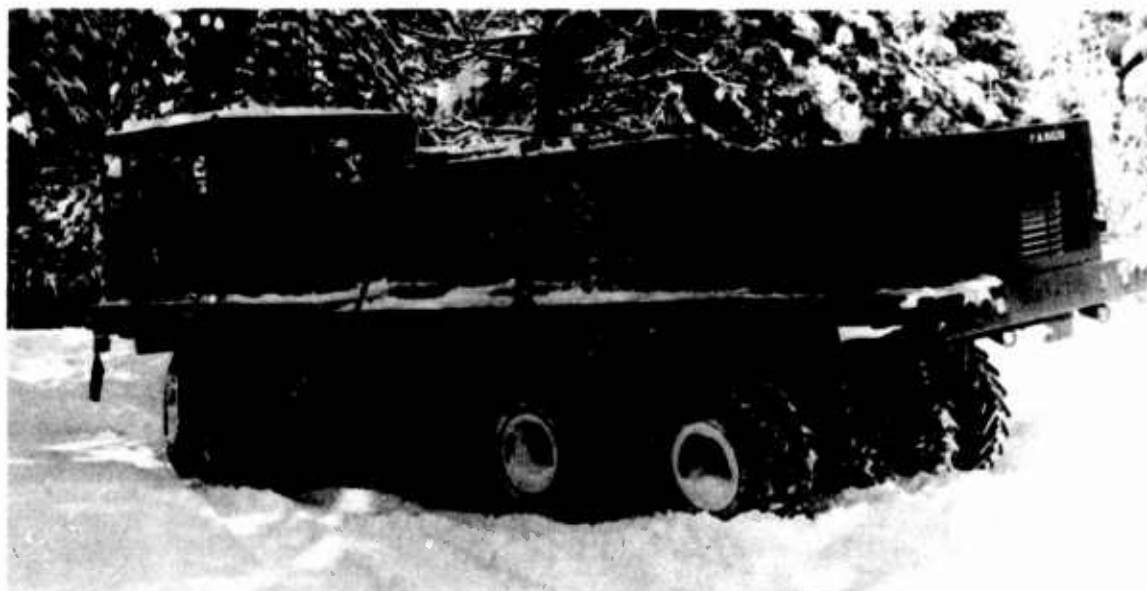
Figure 13. Vehicle operating on forest-covered hilly terrain at Truckee test site.
