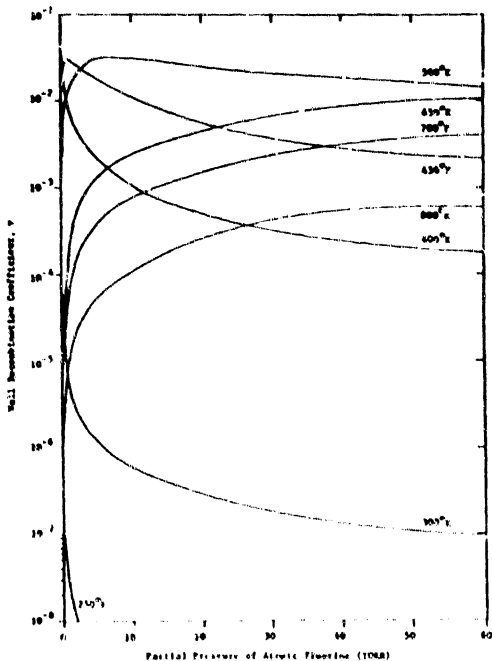
Figure D.2. Fluorine Recombination Coefficient vs. Partial Pressure of Atomic Fluorine for 90% Argon Diluent and 10% Fluorine Dissociation
