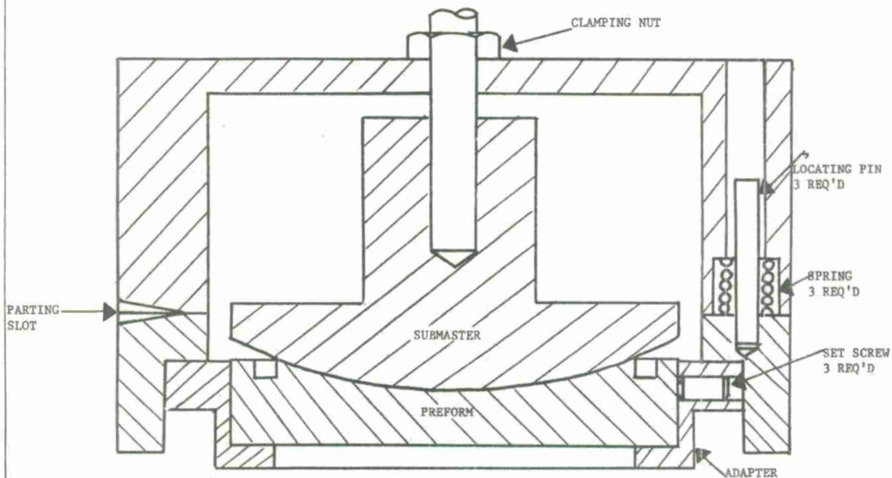
B. SUBMASTER REPLICA &amp; PREFORM REPLICA
