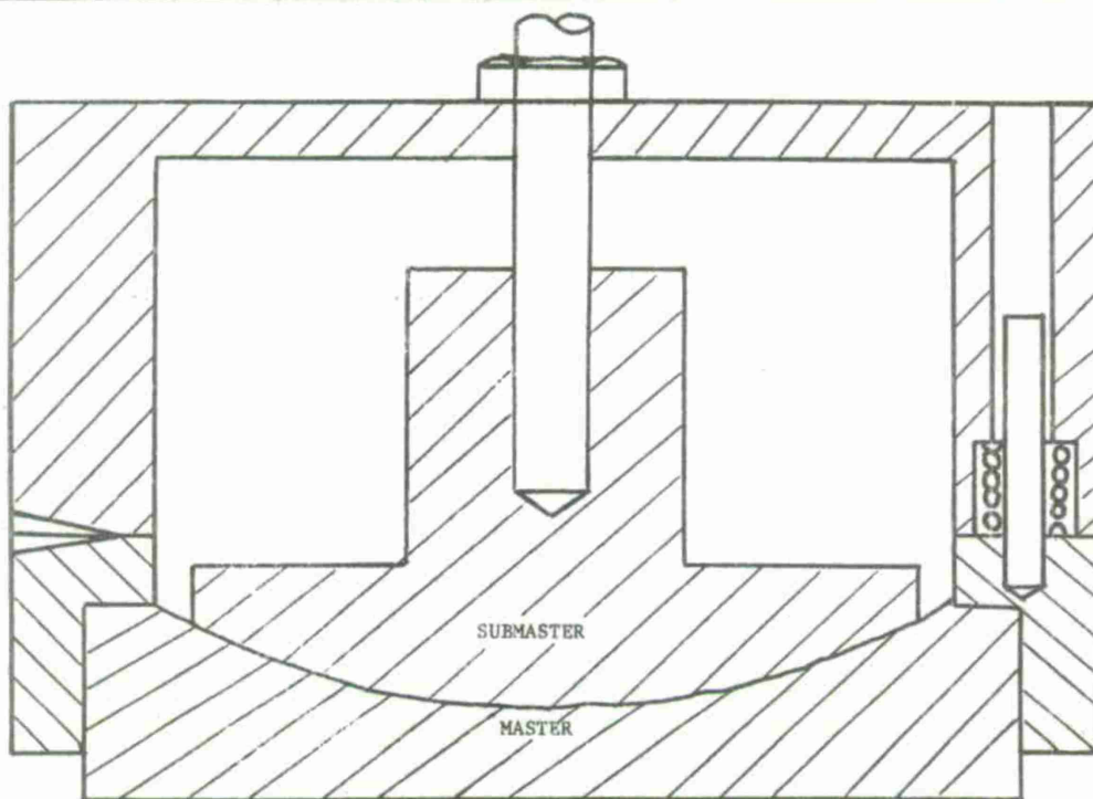
A. MASTER &amp; SUBMASTER REPLICA
