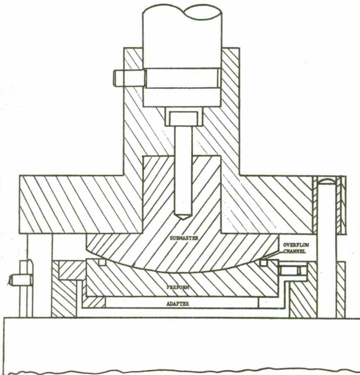
SUBMASTER REPLICA &amp; PREFORM REPLICA
