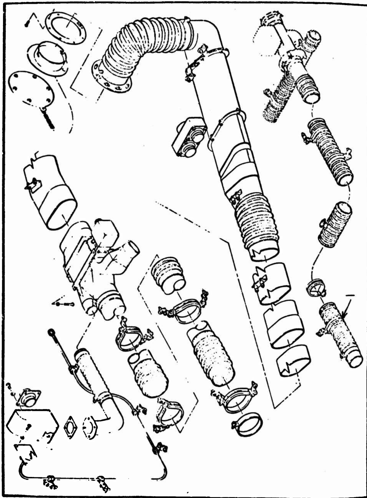
Figure 184 Distribution Illustration, Hot Air Right-Hand Section (UH-1D)
