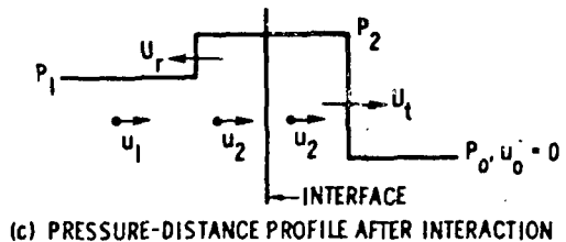
Fig 4 Transmission of a plane shock wave into a material of higher impedance
