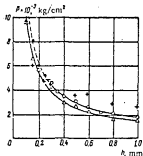
Fig 10. Average pressures P_{ult} and P_{ex} vs charge thickness for PETN ( \circ ) and Trinitrophenol ( \triangle ) Points marked + refer to Dina
