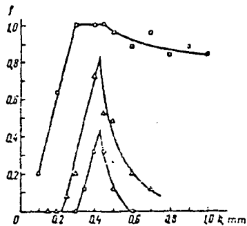
Fig 13. Explosion frequency vs charge thickness in the case of HMX for various impact energies
