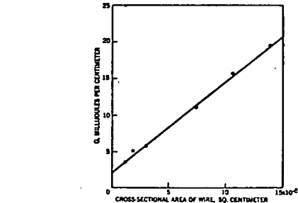
Fig 2. Relation between cross-sectional area of wire and G=A/l ( l =wire length) (Ref 3)
