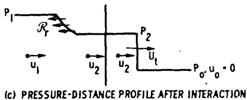
Fig 3 Transmission of a plane shock wave into a material of lower impedance
