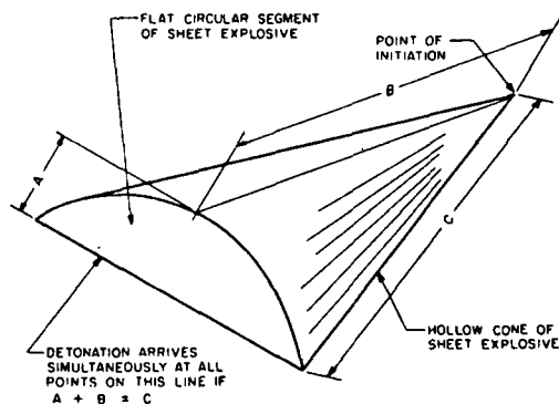
Line Wave Generator of Warped Sheet of Explosive
