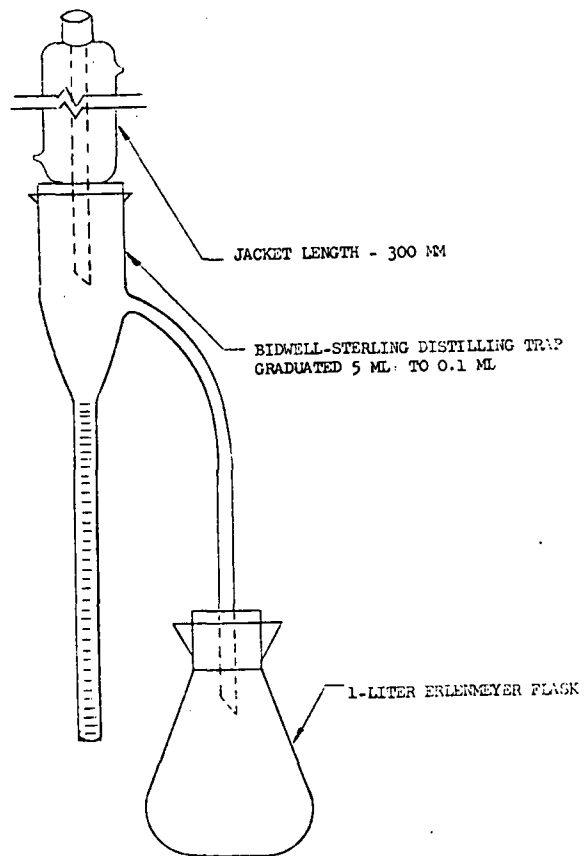
FIGURE 1 Moisture content apparatus
