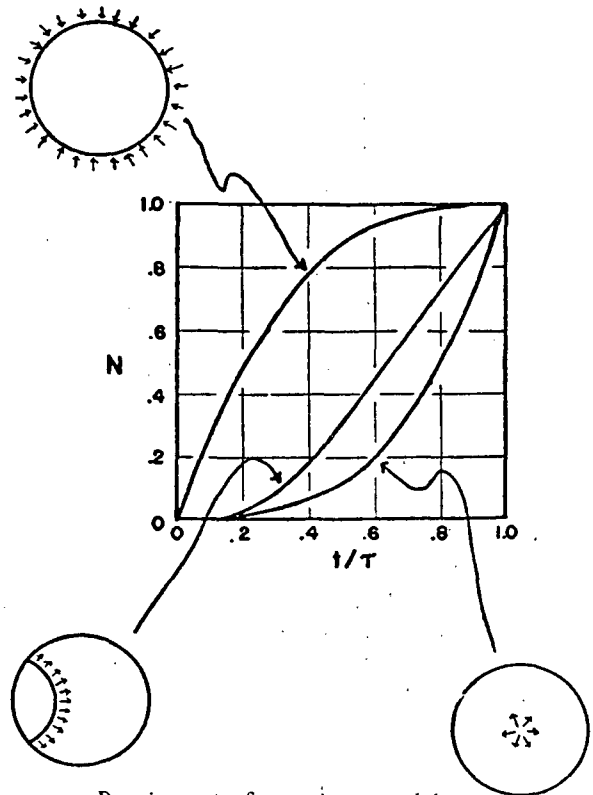
Burning rate for various models
