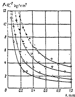
Fig 9. Average pressures upon fracture ( P_{ult} —solid curves) and upon explosion ( P_{ex} —dashed curves) vs charge thickness of HMX ( \circ ), RDX ( \nabla ), Tetryl ( \triangle ) and TNT ( \square )
