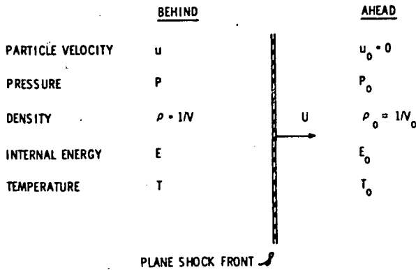
Fig 1 Steady plane shock front propagating into undisturbed materials in laboratory coordinates
