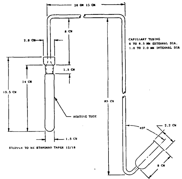
FIGURE 2 Apparatus for 100°C vacuum stability test
