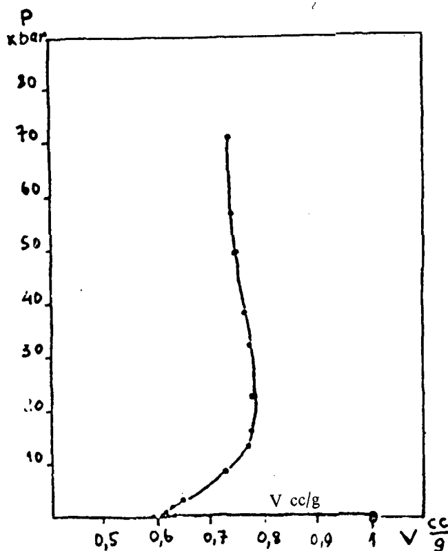
Fig 7 P-V Hugoniot for 1 g/cc TNT
