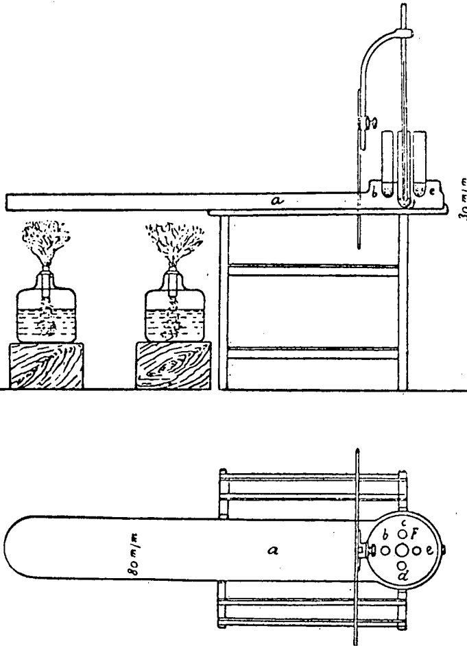
Fig 83. Apparatus for Determining the Temperature of Ignition
