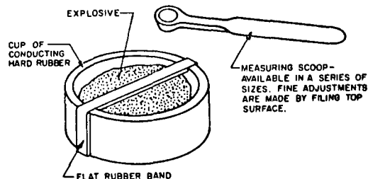
Fig 1 Scoop Loading
