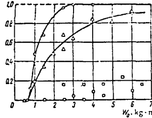
Fig 12. Explosion frequency vs impact energy for Tetryl ( \square ) and RDX ( \triangle ) for charges 0.4mm thick and for HMX ( \circ ) charges 0.5mm thick
