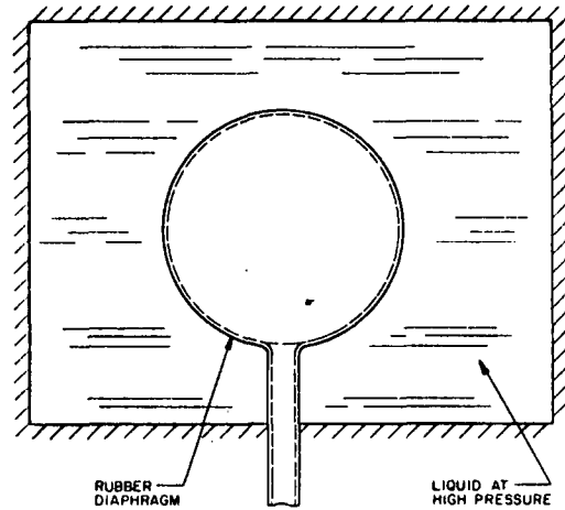
Fig 8 Isostatic Press Principle
