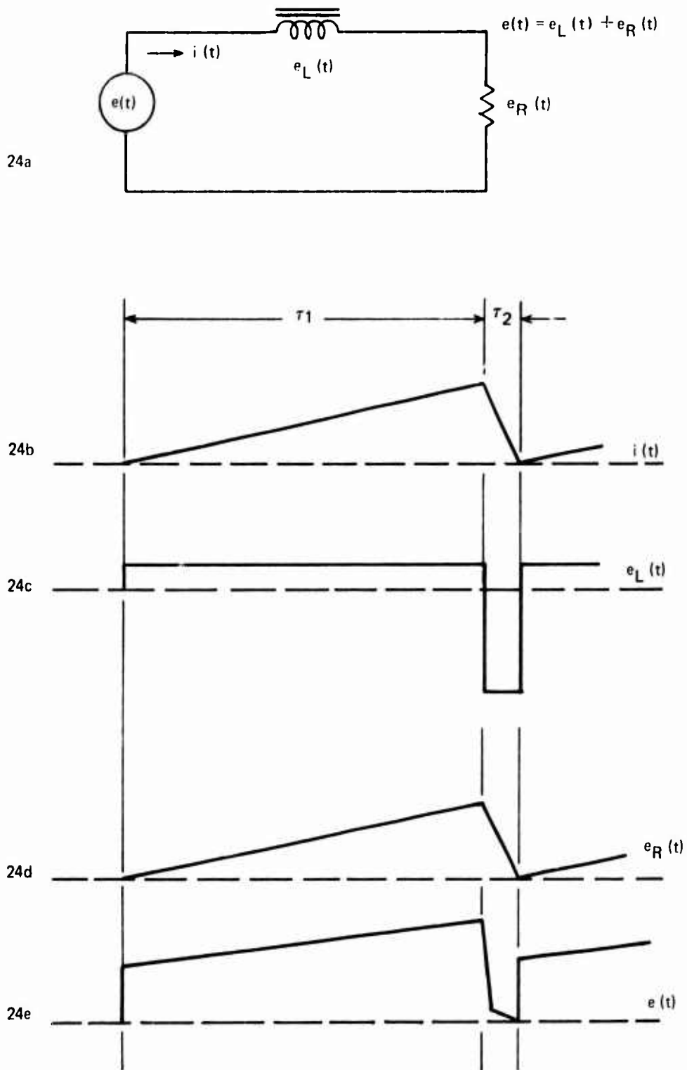
Figure 24. LR Circuit
