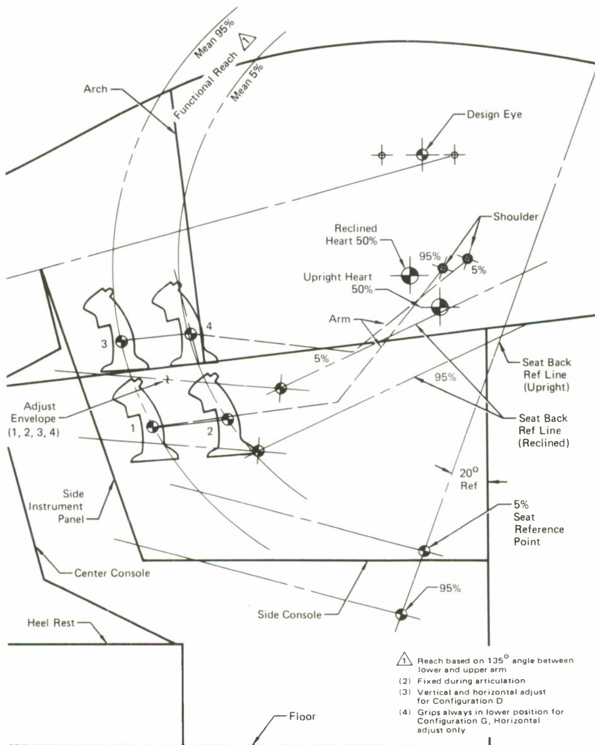
FIGURE 12 INSTRUMENT PANEL MOUNTED CONTROLLERS Configuration D
