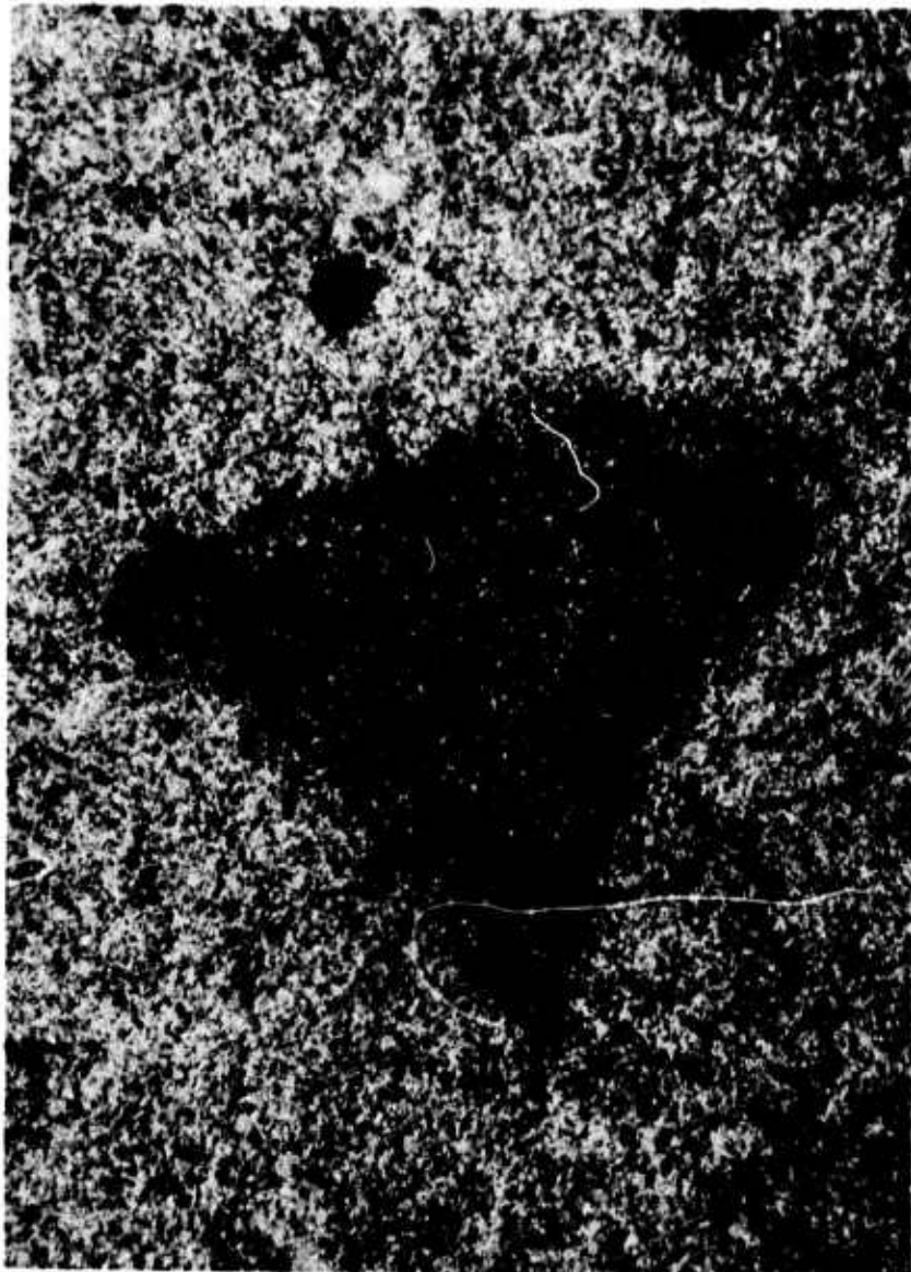
Fig. 23 Microstructure of a dense, solid region in sintered \beta -SiC containing 0.8% C and 0.6% B chemically etched in 10 parts KOH + 1 part KNO 3 at 650°C for 30 seconds.
