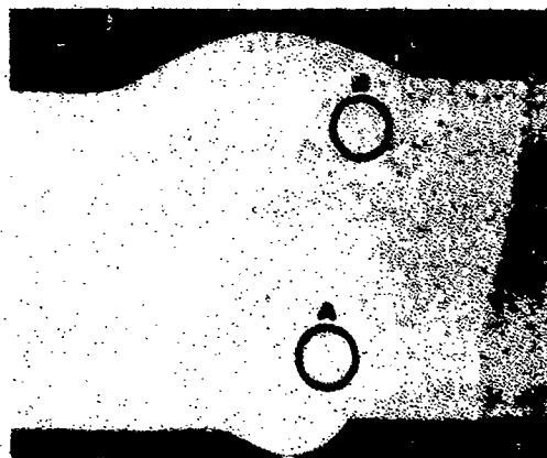
Figure 17. The Profile of Weld 4PAW-FM-3. Area A Identifies Location Where Very Fine Porosity Was Detected in Weld 4PAW-FM-2 (Figure 18). Area B Identifies Location Where Porosity Was Detected in 4PAW-FM-3 (Figure 19) (10X MAG)
