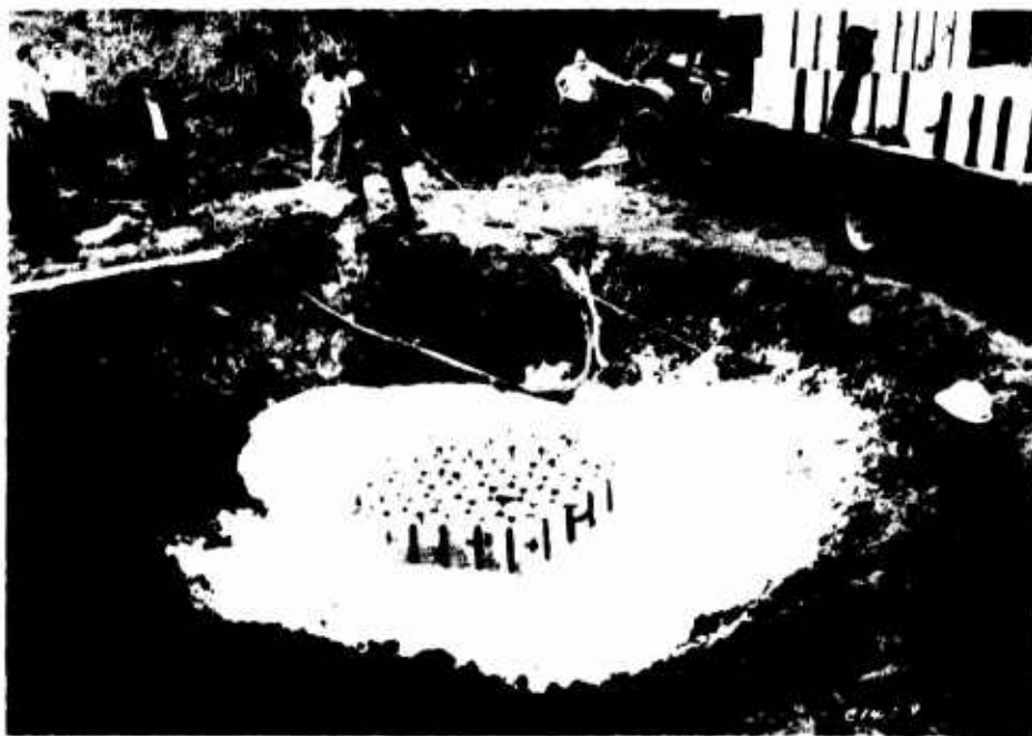
Figure 5.16 Placement of cellular concrete around bottom module.
