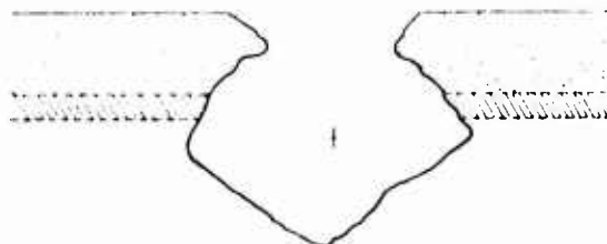
TYPE 5 - CAMOUFLET WITH SPALL CRATER
