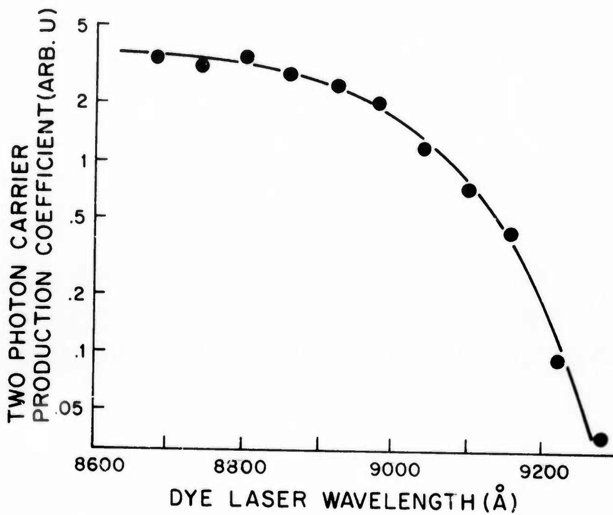
Figure 2. Two photon carrier production coefficient vs. wavelength for ZnSe.
