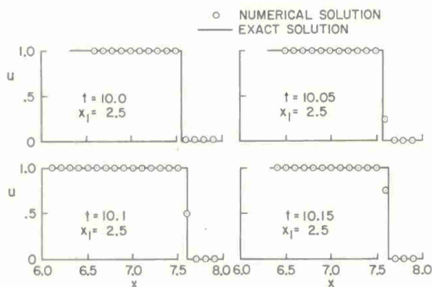
Fig. 2 Solution of Burger's equation (modified method, CFL = 0.1).
