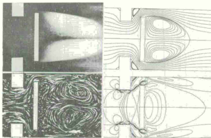
Fig. 23 Flow pattern in idealised heart valve. Computed lines of constant stream function and shearing stress distribution were provided by T. J. Mueller.
