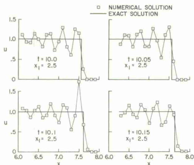
Fig. 1 Solution of Burger's equation (basic method, CFL = 0.1).
