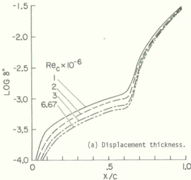
Fig. 11 Thickness parameters on 18-percent circular arc ( M_\infty = 0.775 ).
