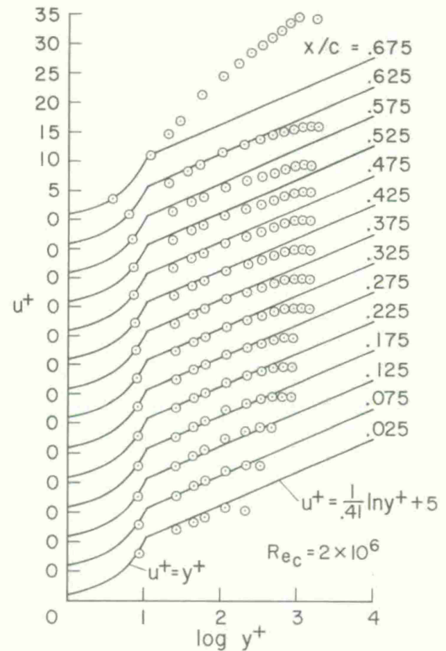
Fig. 12 Velocity profiles ahead of shock.
