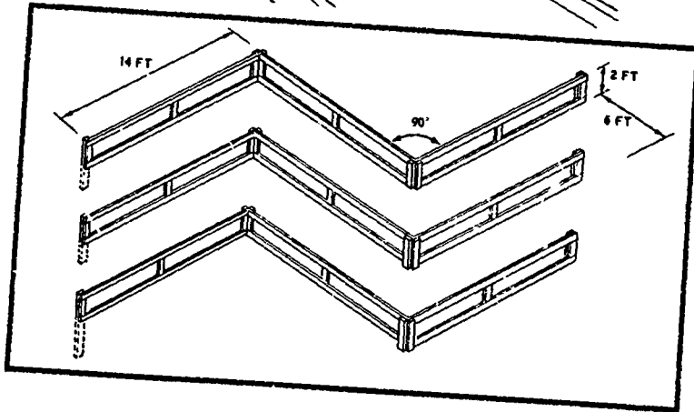
Fig. 24A. 90° passways.
