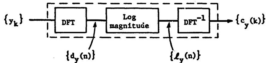
Fig. 2. Computation of the Real Cepstrum.
