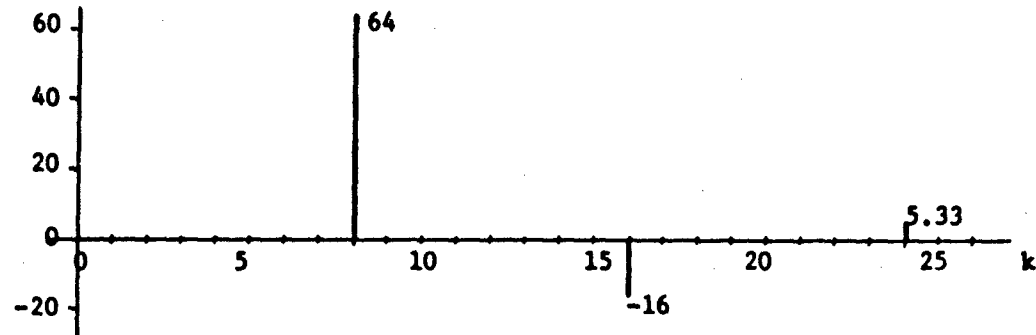
Fig. 1. Portion of Discrete Multipath Cepstrum, for N = 256 , r = 8 , \alpha = 0.5
