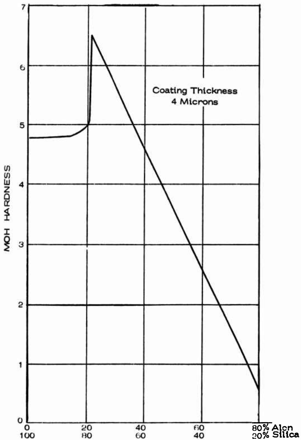
Figure 2. Moh Hardness vs. % Silica/% Alon on Glass.
