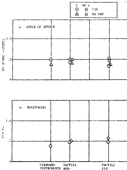
Figure 4-8. AOA Error and Monitoring Performance Average of 4 subjects.
