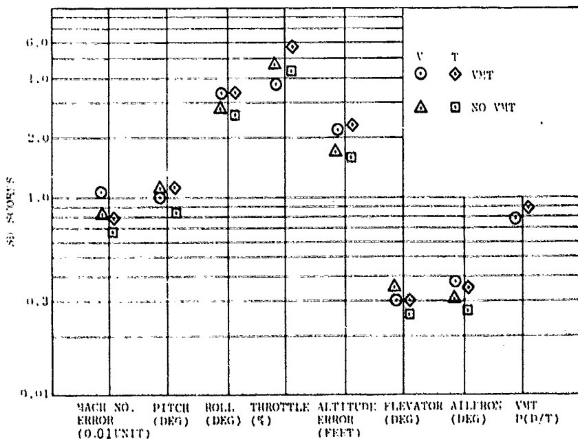
Figure 4-2. Performance Scores for Straight and Level Flight. (Average of six subjects).
