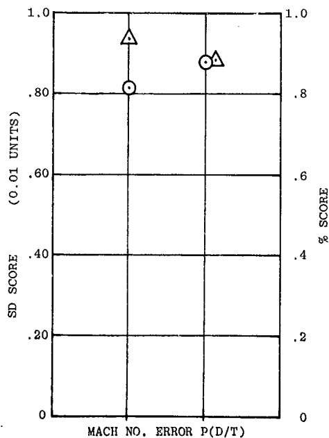
Figure 4-6. Comparison of Vibrotactors and Electrotactors Straight and Level, Average of 6 Subjects.
