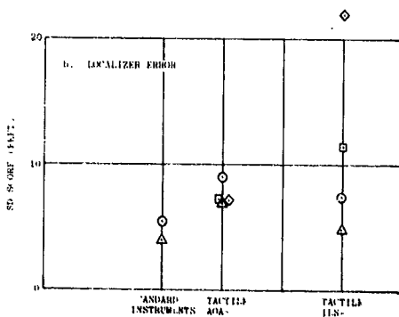
Figure 4.7. Effects of Display and VMT on Path Performance, Average of 4 subjects.
