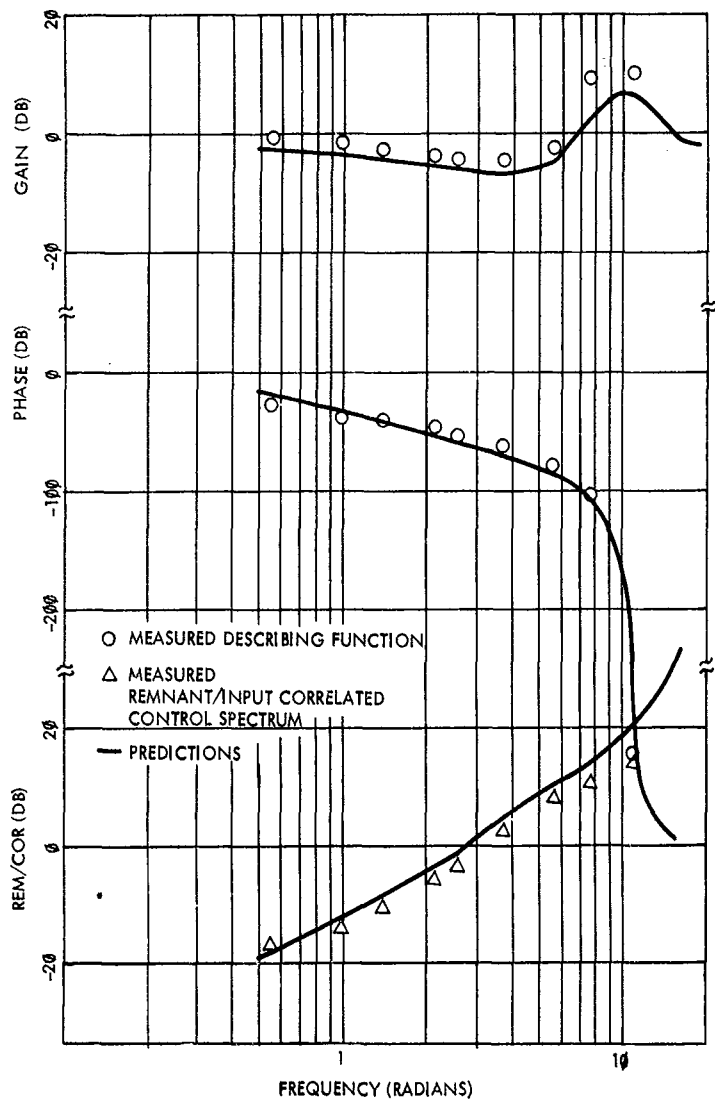
FIGURE 3-8. FREQUENCY-DOMAIN MEASURES FOR TACTILE TRACKING, 1-AXIS PITCH WITH LARGER INPUT (AVERAGE OF 4 SUBJECTS).
