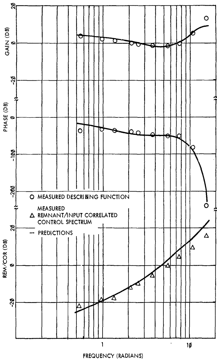
FIGURE 3-7. FREQUENCY-DOMAIN MEASURES FOR VISUAL TRACKING, 1-AXIS PITCH (AVERAGE OF 4 SUBJECTS).
