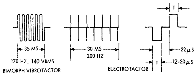
(a) TACTOR STIMULUS SIGNALS
