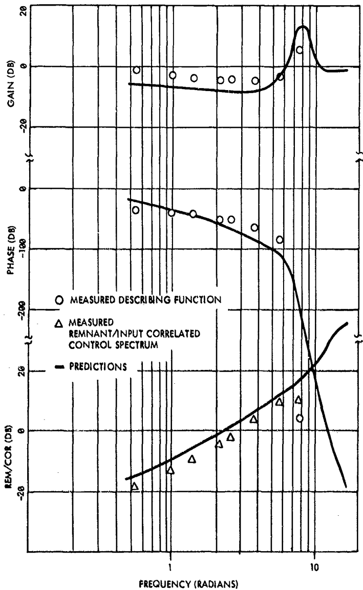
FIGURE 3-10. FREQUENCY-DOMAIN MEASURES FOR TACTILE TRACKING, 1-AXIS PITCH WITH SMALLER INPUT (AVERAGE OF 4 SUBJECTS).
