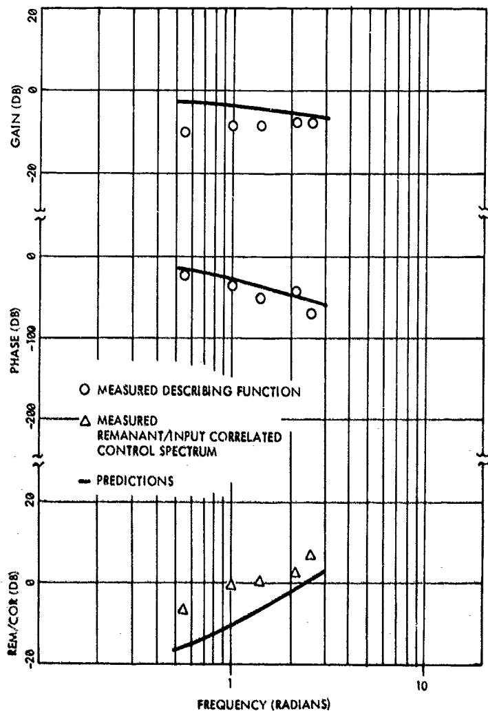
FIGURE 3-12. FREQUENCY-DOMAIN MEASURES FOR TACTILE TRACKING, 2-AXIS PITCH WITH LARGER INPUT (AVERAGE OF 4 SUBJECTS).
