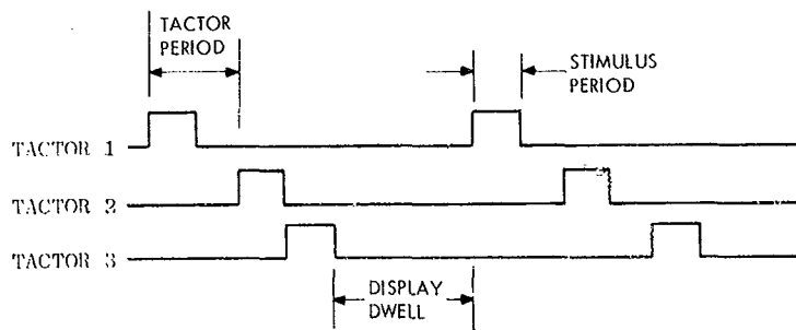
(b) TACTILE DISPLAY PERIODS
