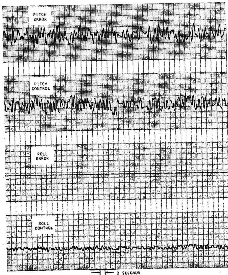
Figure 3-3 Time Histories of Error and Control Signals. Subject JK; Task = Pitch Relative Input Amplitude = 0.50
