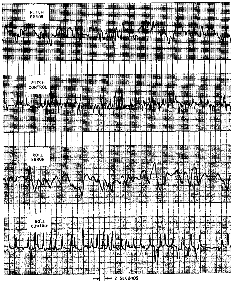
Figure 3-2 Time Histories of Error and Control Signals. Subject RF; Task = Pitch+Roll Relative Input Amplitude = 0.25
