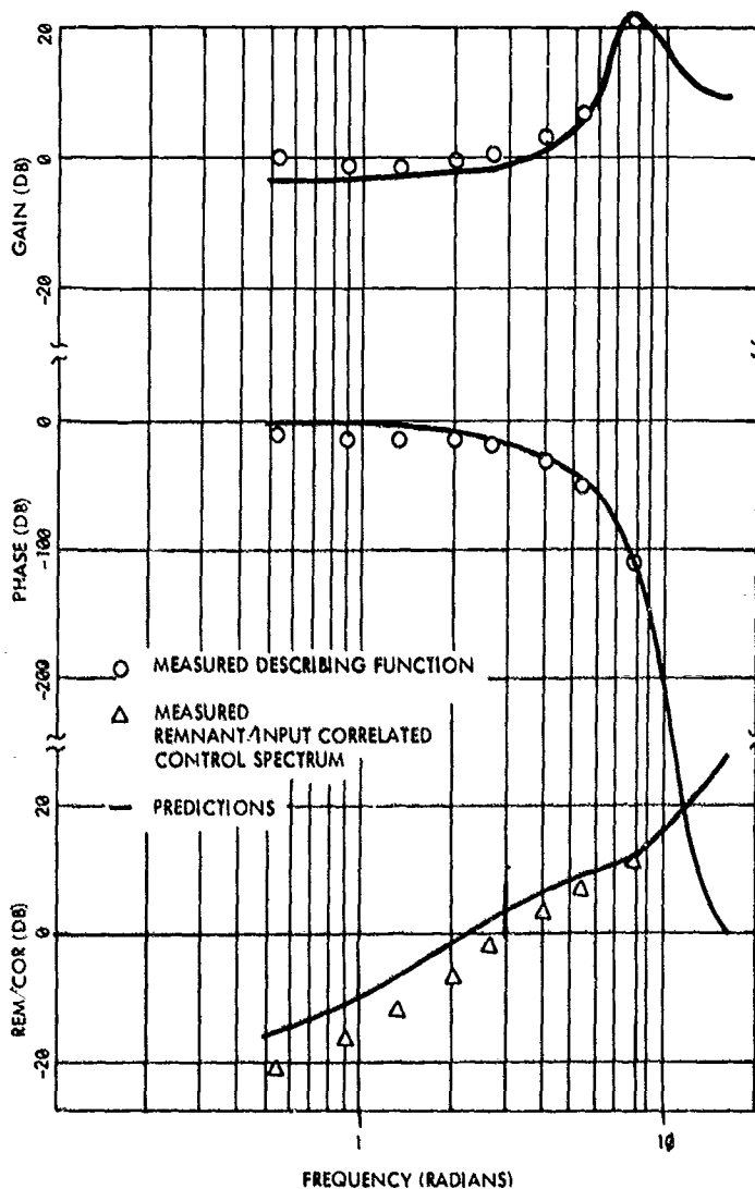
FIGURE 3-11. FREQUENCY-DOMAIN MEASURES FOR TACTILE TRACKING, 1-AXIS ROLL WITH LARGER INPUT (AVERAGE OF 4 SUBJECTS).
