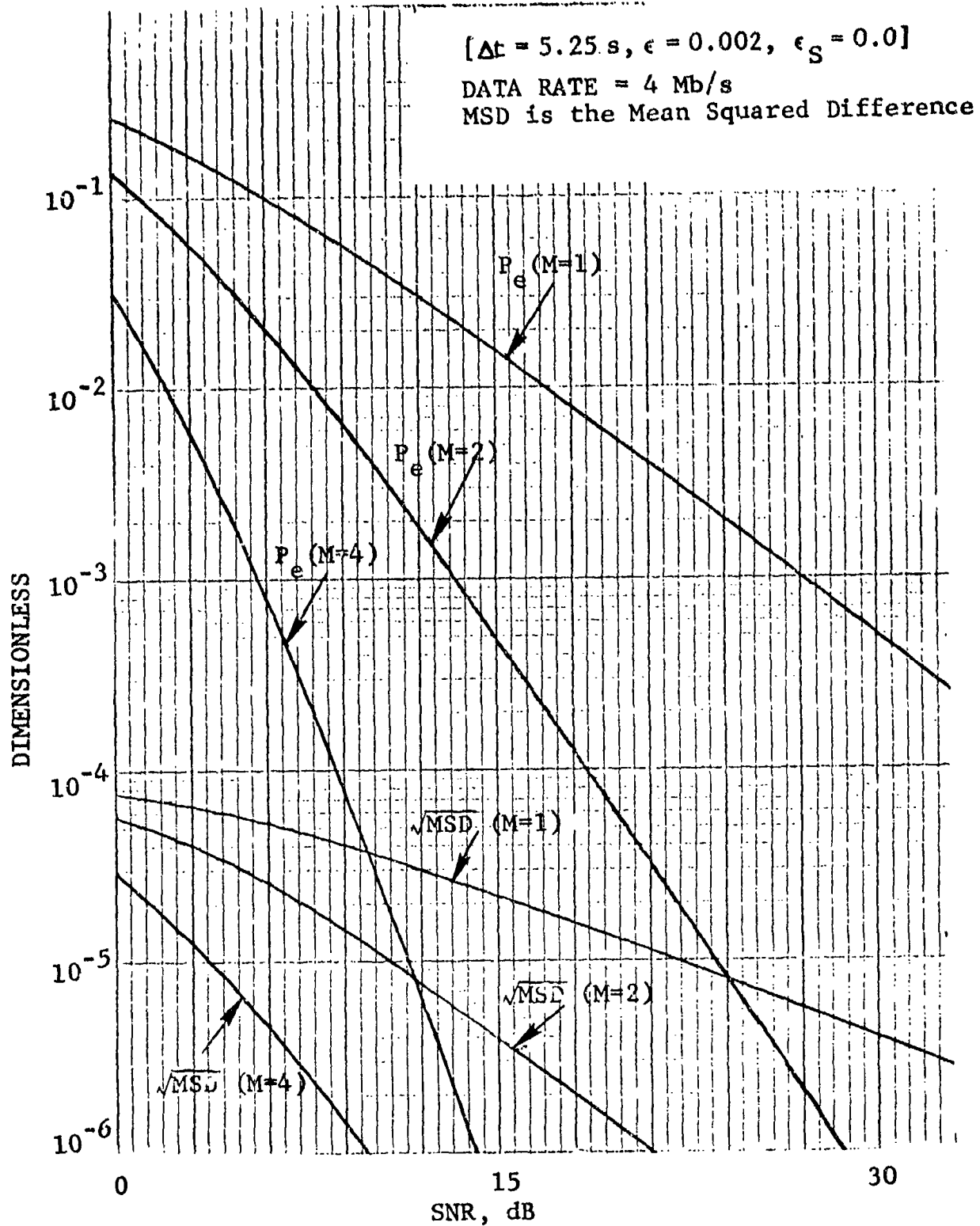
Figure 5.10 Performance of Error Burst Estimator for LOS Channel (15-second Estimation Time)
