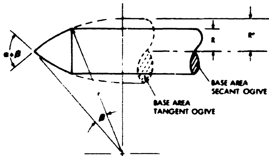
FIG. 5 OGIVE GEOMETRY
