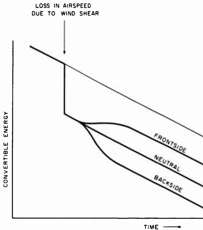
FIG 4 EFFECT OF LOSS IN AIRSPEED DUE TO WIND SHEAR ON 'CONVERTIBLE' ENERGY DISSIPATION RATE IF PITCH ATTITUDE REMAINS CONSTANT
