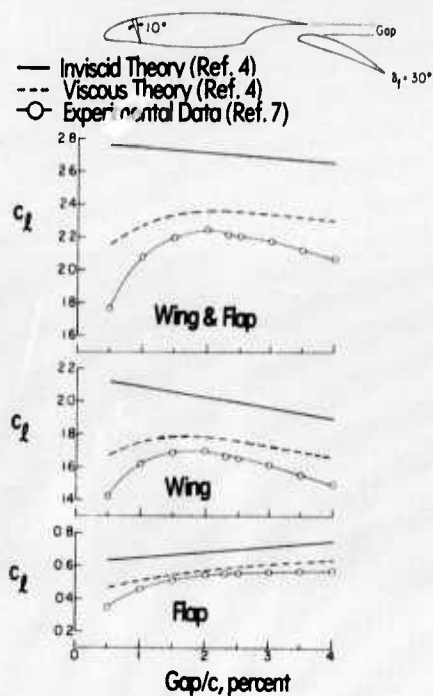
Figure 5. - Gap optimization results from 10^\circ -drooped nose airfoil with slotted flap.
