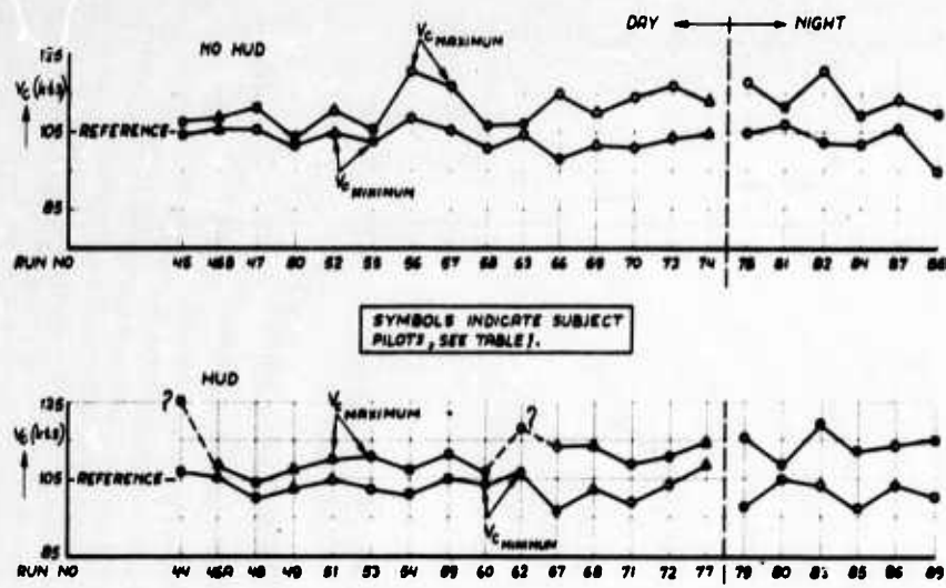
FIG. 7: MAXIMUM AND MINIMUM CALIBRATED AIR SPEED ( V_c ) DURING NO-HUD- AND HUD- APPROACHES.
