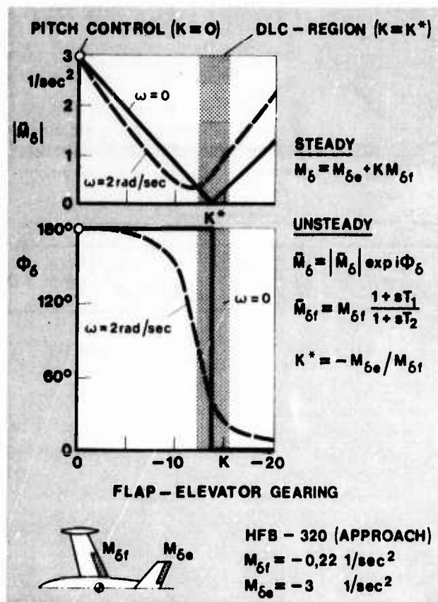
Fig. 7 Effect of unsteady aerodynamics on control derivative M_\delta
