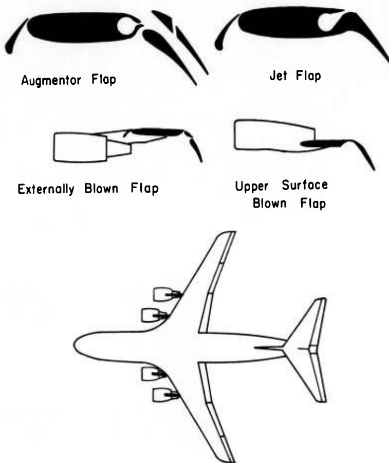
Figure 13. - Propulsive-lift-flap concepts.
