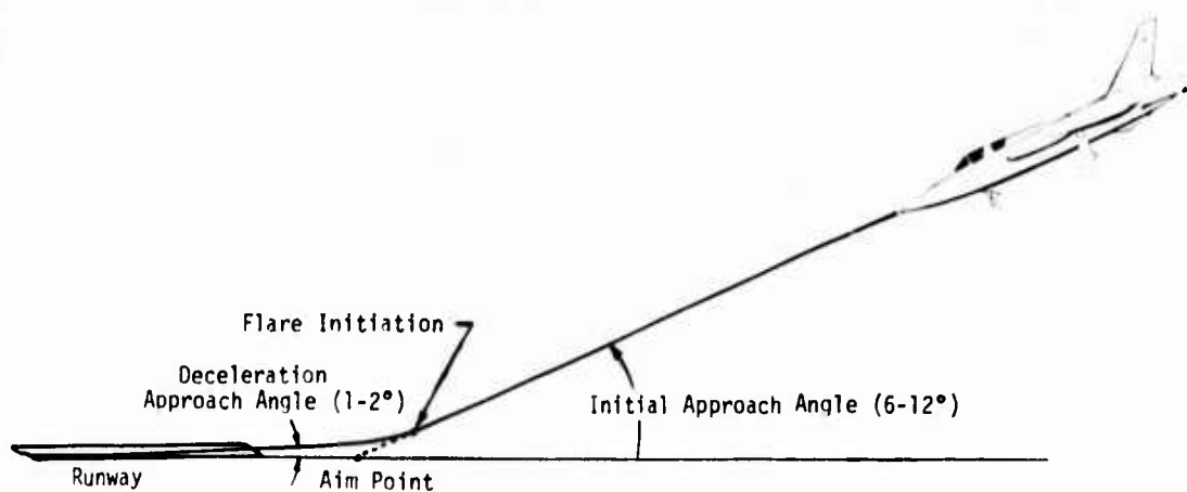
Figure 4. Low Power Approach Technique
