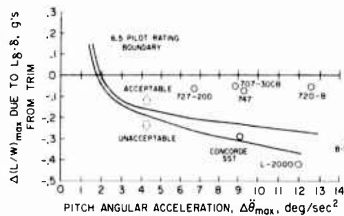
Fig. 12 Pitch control power criteria, \Delta\theta_{\max} (from trim).
