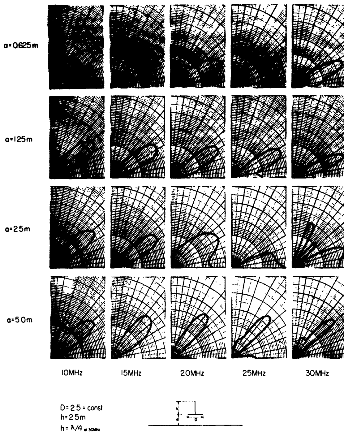
Fig. 4. 12. Radiation patterns |E_\theta|^2 for various ground plane locations (a) with D = 2.50\text{m}
