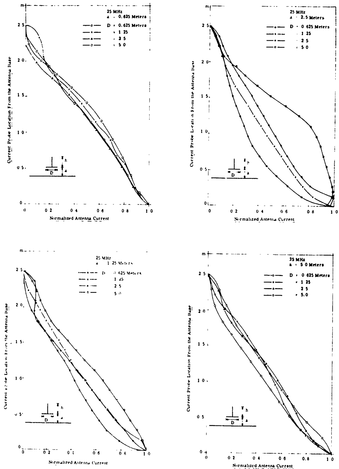
Fig. 3. 16. Current distribution on a monopole antenna with a ground plane of various diameters at a given location with respect to an infinite ground at 25 MHz
