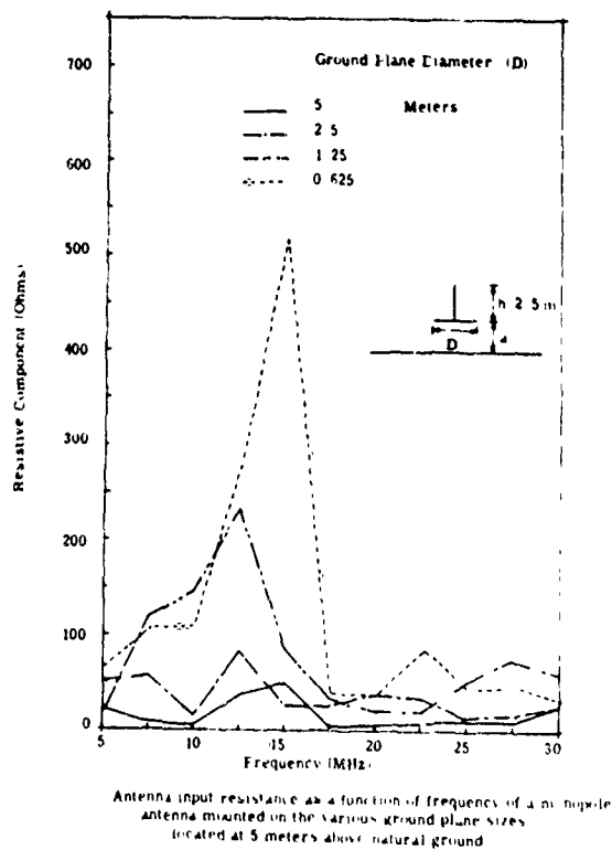
Fig. 2.12. Input impedance versus frequency
