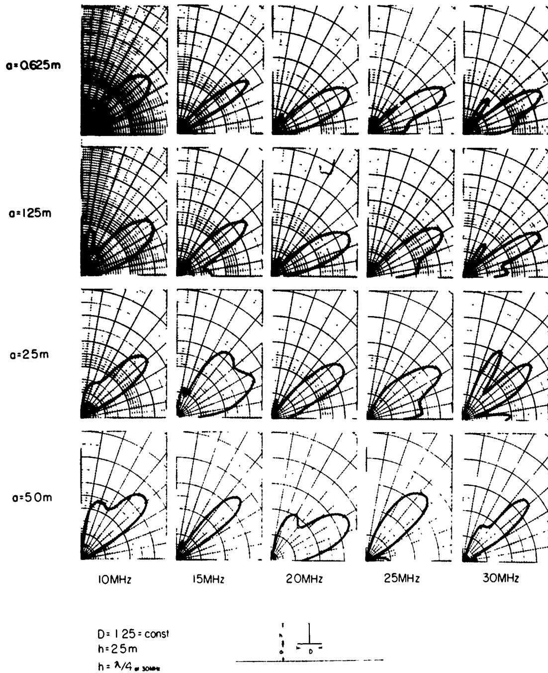
Fig.4. 11. Radiation patterns |E_\rho|^2 for various ground plane locations (a) with D = 1.25\text{m}
