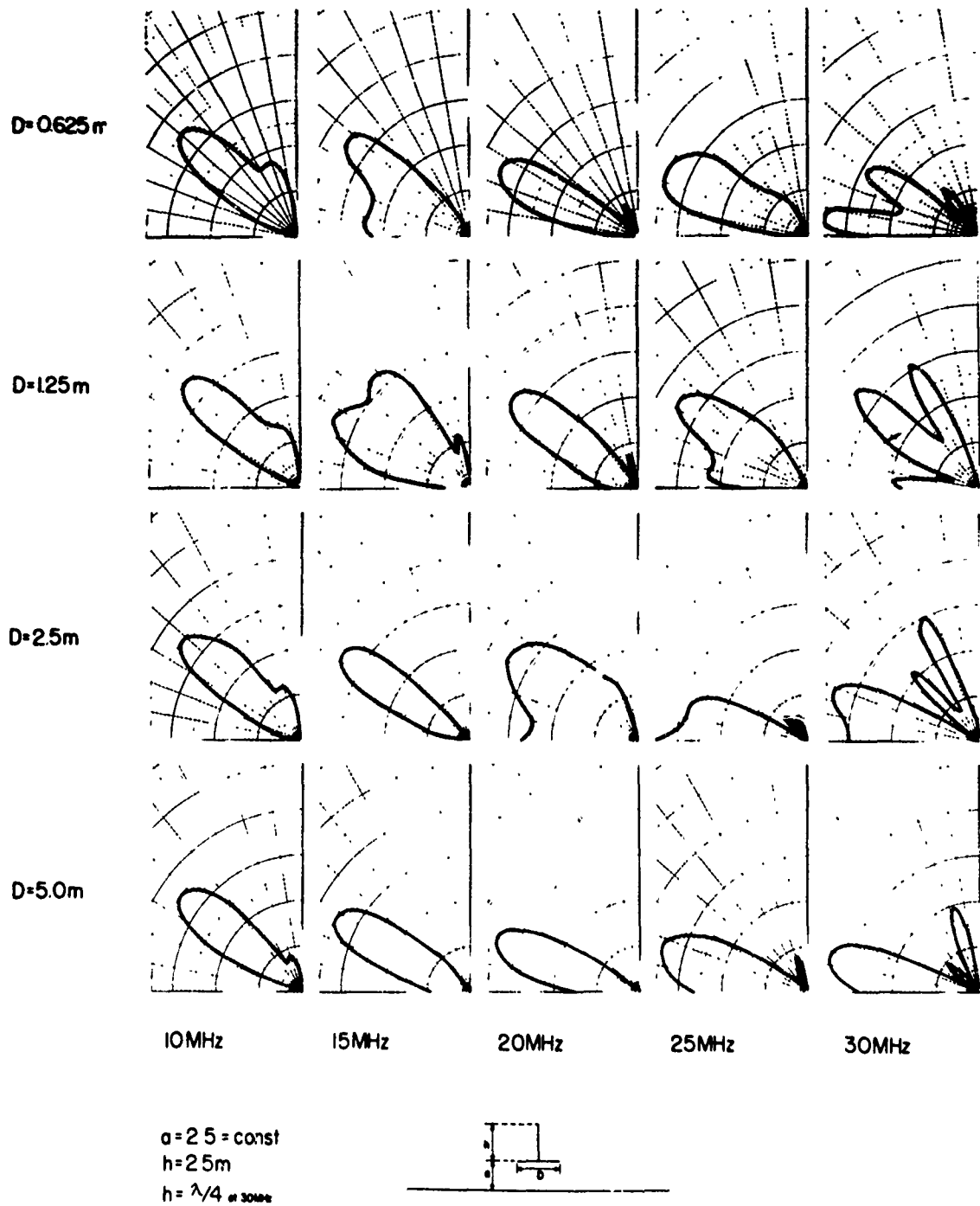
Fig. 4. 8. Radiation patterns |E_\theta|^2 for various ground plane diameters ( D ) with a = 2.5\text{m} .
