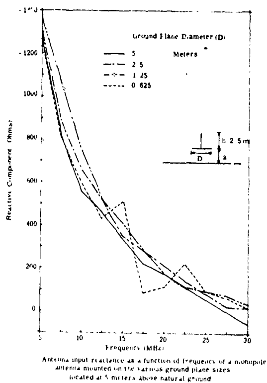
Fig. 2.12. Input impedance versus frequency
