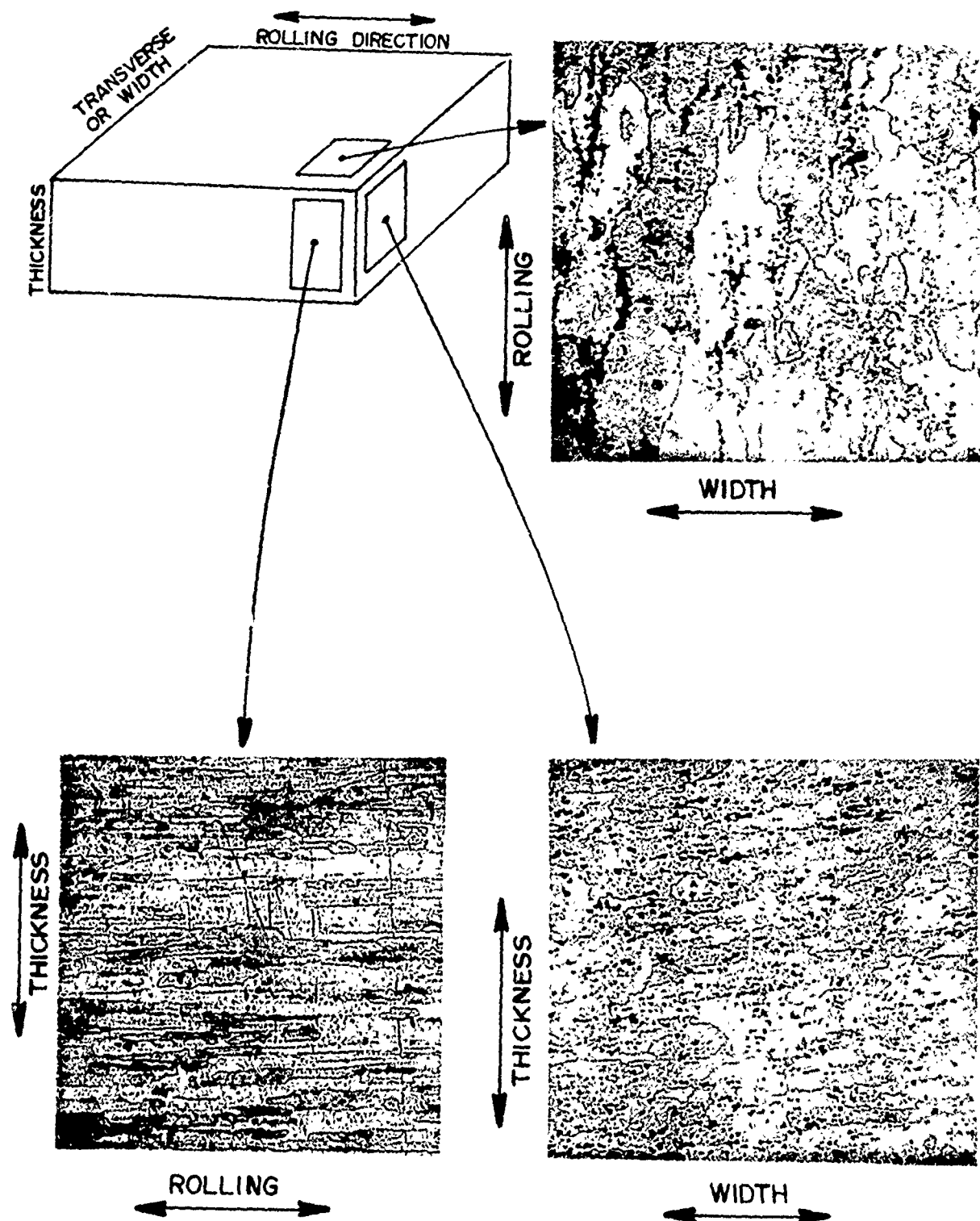
Figure 1. Photomicrographs of 2014-T651 Aluminum Plate
