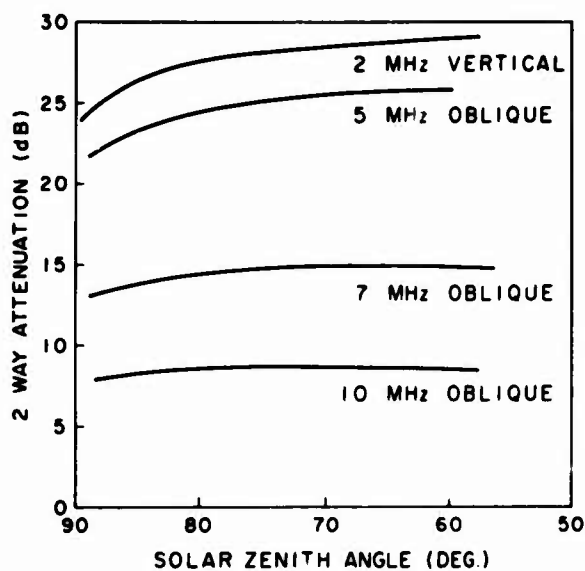
Figure 6. Attenuation as a Function of Solar Zenith Angle and Frequency for Vertical Incidence (at 2 MHz) and for Oblique Incidence on the RECAP-Alert Path
