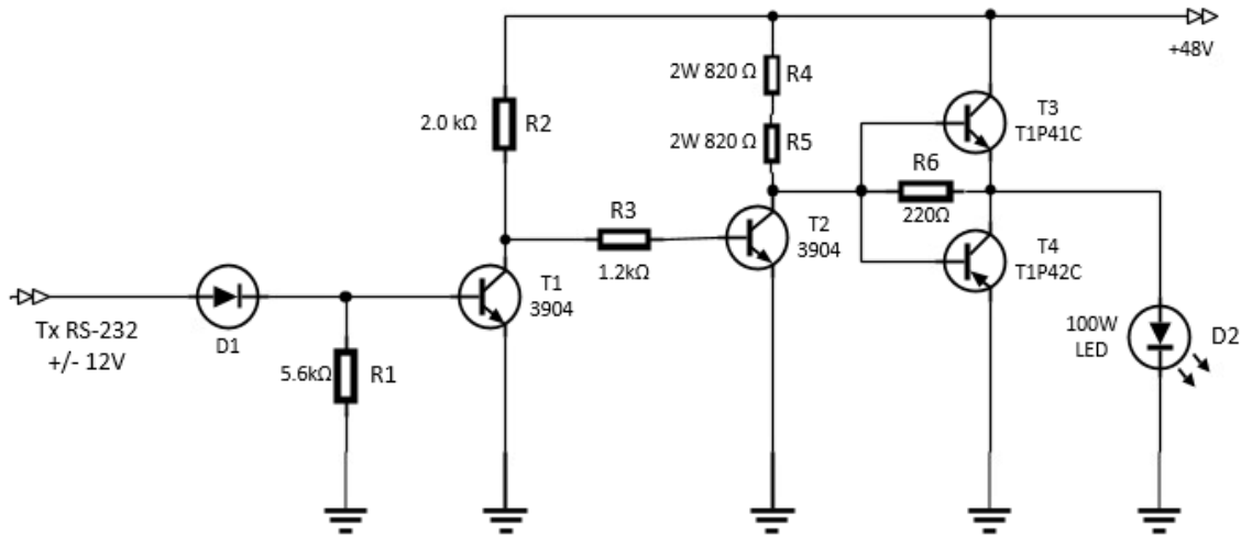
Figure 21. 100-Watt LED Transmitter Prototype Schematic
