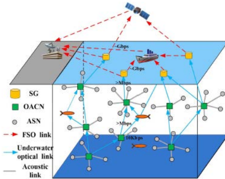
Figure 2. Potential Integrated Network Using Optical and Acoustic Communication. Source: Xing et al. (2018).
