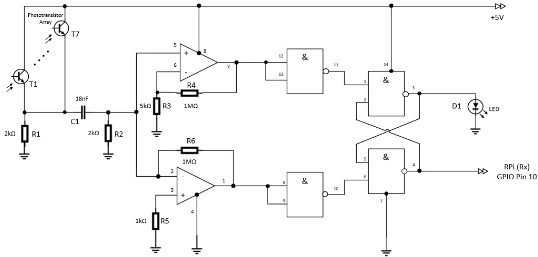
Figure 22. Phototransistor Array Receiver Prototype Schematic
