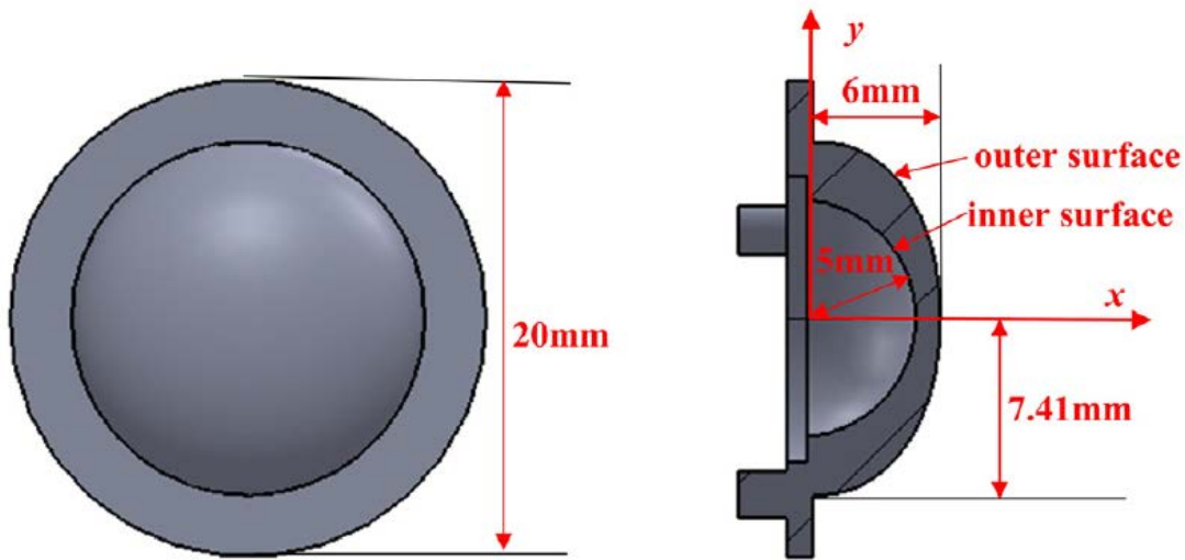
Figure 12. Quasi-omnidirectional Transmitter. Source: Han et al. (2018).
