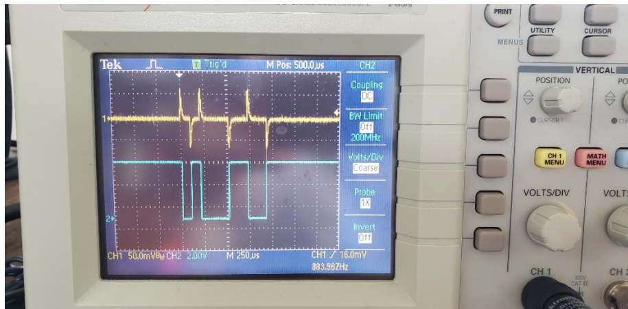
Figure 23. 9600 Baud Rate
