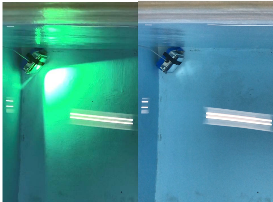
Figure 29. VLC Transmitter Operating in Clear Water
