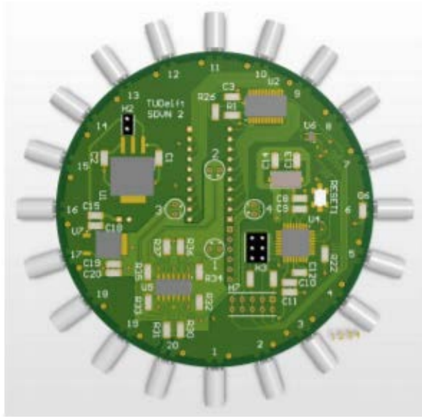
Figure 14. VLC Transmitter with 20 LEDs in Array. Source: Klaver and Zuniga (2015).
