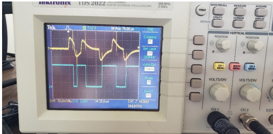
Figure 24. 57600 Baud Rate
