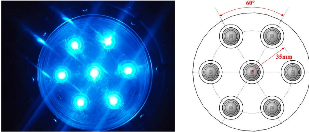
Figure 13. Arrangement of Blue LED Array. Source: Han et al. (2018)
