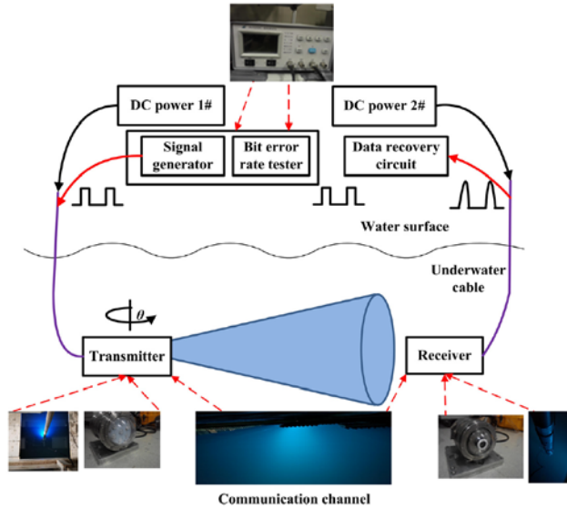
Figure 15. Experiment Design with Transmitter and Receiver Submerged. Source: Han et al. (2018)
