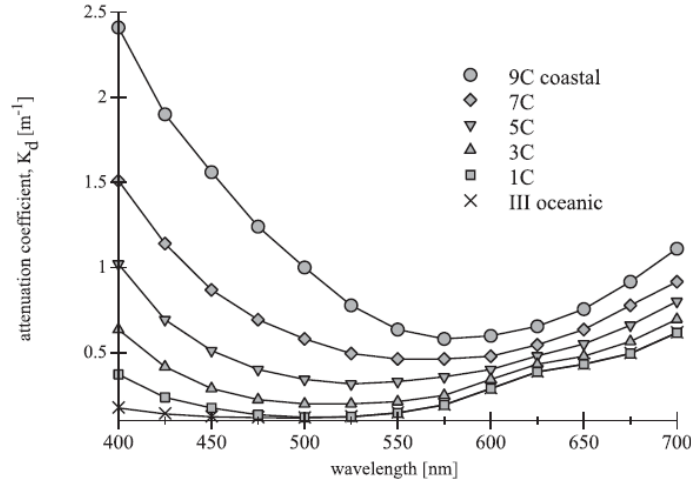
Figure 10. Plot of Attenuation Coefficients for Jerlov Water Types vs. Visible Light Wavelengths. Source: Sticklus et al. (2019).
