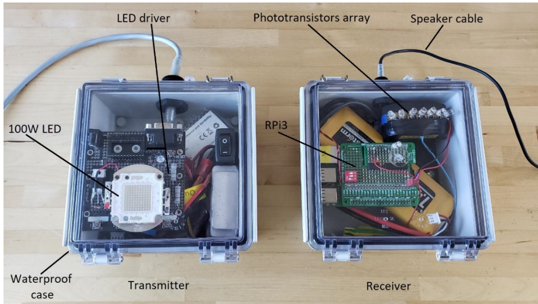
Figure 28. Waterproofed VLC Transmitter and Receiver Systems
