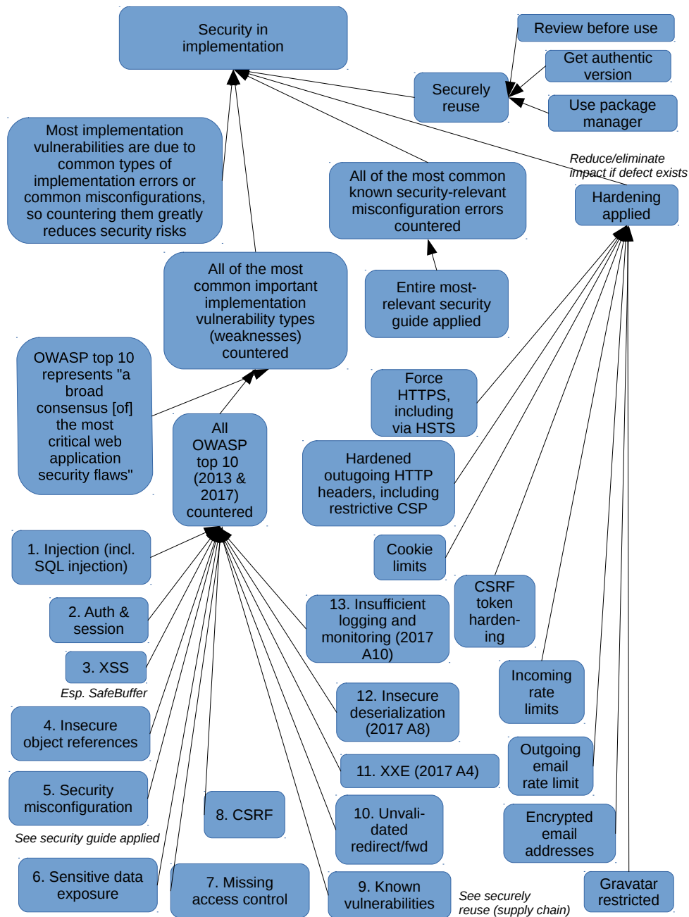
Figure 10. Application: Implementation
