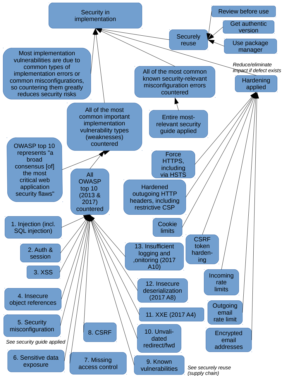
Figure 3. Implementation—Web Application
