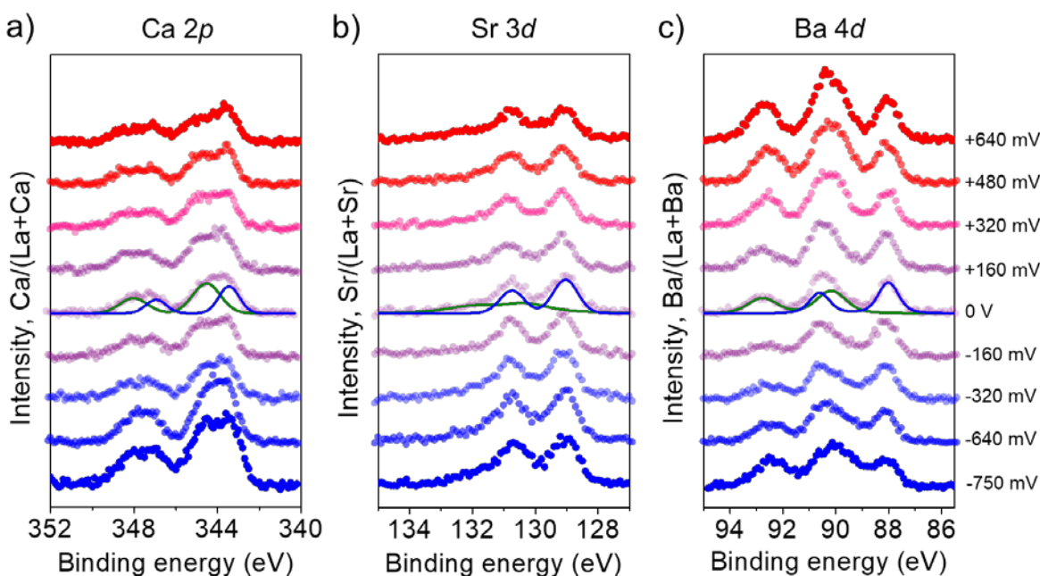
Figure 1-4. X-ray photoelectron spectra taken for Ca 2p, Sr 3d, and Ba 4d illustrating the extent of dopant segregation at the surface as a function of applied potential at 770°C in 1 atm O 2 for 1 h for a) La 0.8 Ca 0.2 MnO 3 , b) La 0.8 Sr 0.2 MnO 3 , and c) La 0.8 Ba 0.2 MnO 3 . The 0 mV spectrum in each core-level is deconvoluted into the emission arising from the surface (green) and lattice (blue) binding environments.
