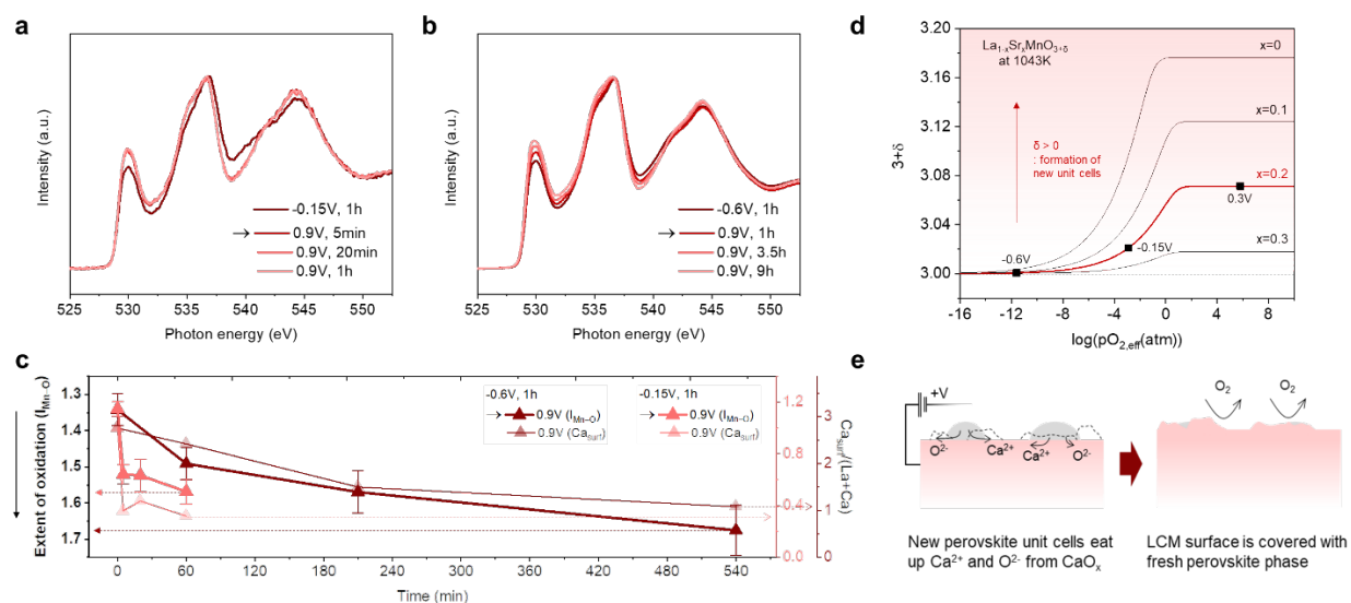
Figure 4-7. Oxygen-excess non-stoichiometry of LCM coupled with a formation of new fresh unit cell reactivates its surface. a , Total-electron-yield O K-edge XAS spectra measured on LCM thin films after annealing under -0.15V, followed by annealing under 0.9V for 5min, 20min, and 1h. b , Another set of samples were annealed under -0.6V, followed by annealing under 0.9V for 1h, 3.5h, and 9h. c , The area of Mn 3d-O 2p peaks in each O K-edge XAS spectra is integrated and plotted with respect to the time we applied anodic polarization (please read the thick y-axis at the left side). Deep pink triangles indicate the samples initially annealed at -0.15V for 1h and deep brown triangles represent those annealed at -0.6V for 1h. For comparison, the amount of \text{Ca}_{\text{surf}} is plotted together with light colors (please read the thin y-axis at the right side). d , Oxygen-excess non-stoichiometry of \text{La}_{1-x}\text{Sr}_x\text{MnO}_{3+\delta} ( x=0, 0.1, 0.2 , and 0.3 ) with respect to effective \text{pO}_2 (replotted from a previous work by Mizusaki et al. 82 ). The curve that coincides with the composition of our LCM is colored in red and the anodic polarization values we used are converted to the corresponding \text{pO}_{2,\text{eff}} according to Nernst equation (marked as squares). e , Schematics describing the mechanism of activation process on LCM under anodic polarization.
