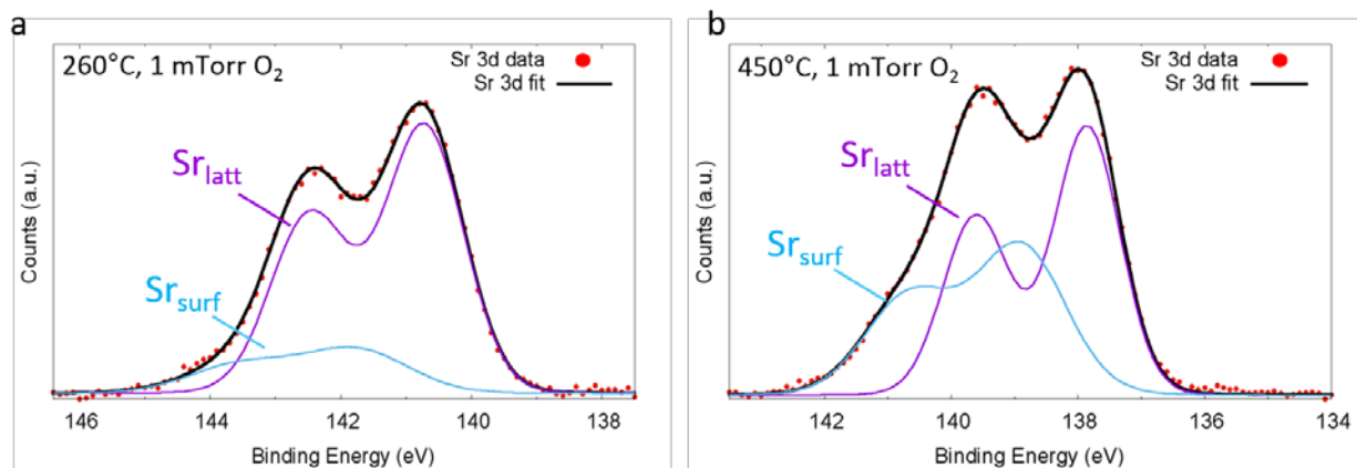
Figure 2-1. Sr 3d spectra of La 0.8 Sr 0.2 MnO 3 /YSZ acquired in-situ in 1mTorr O 2 at 260°C (a) and 450°C (b). The deconvolution shows two species, Sr in the La 0.8 Sr 0.2 MnO 3 lattice (Sr latt , purple) and the segregating SrO x species (Sr surf , cyan). At 450°C a substantial increase in Sr surf is observed, corresponding to surface segregation of Sr.
