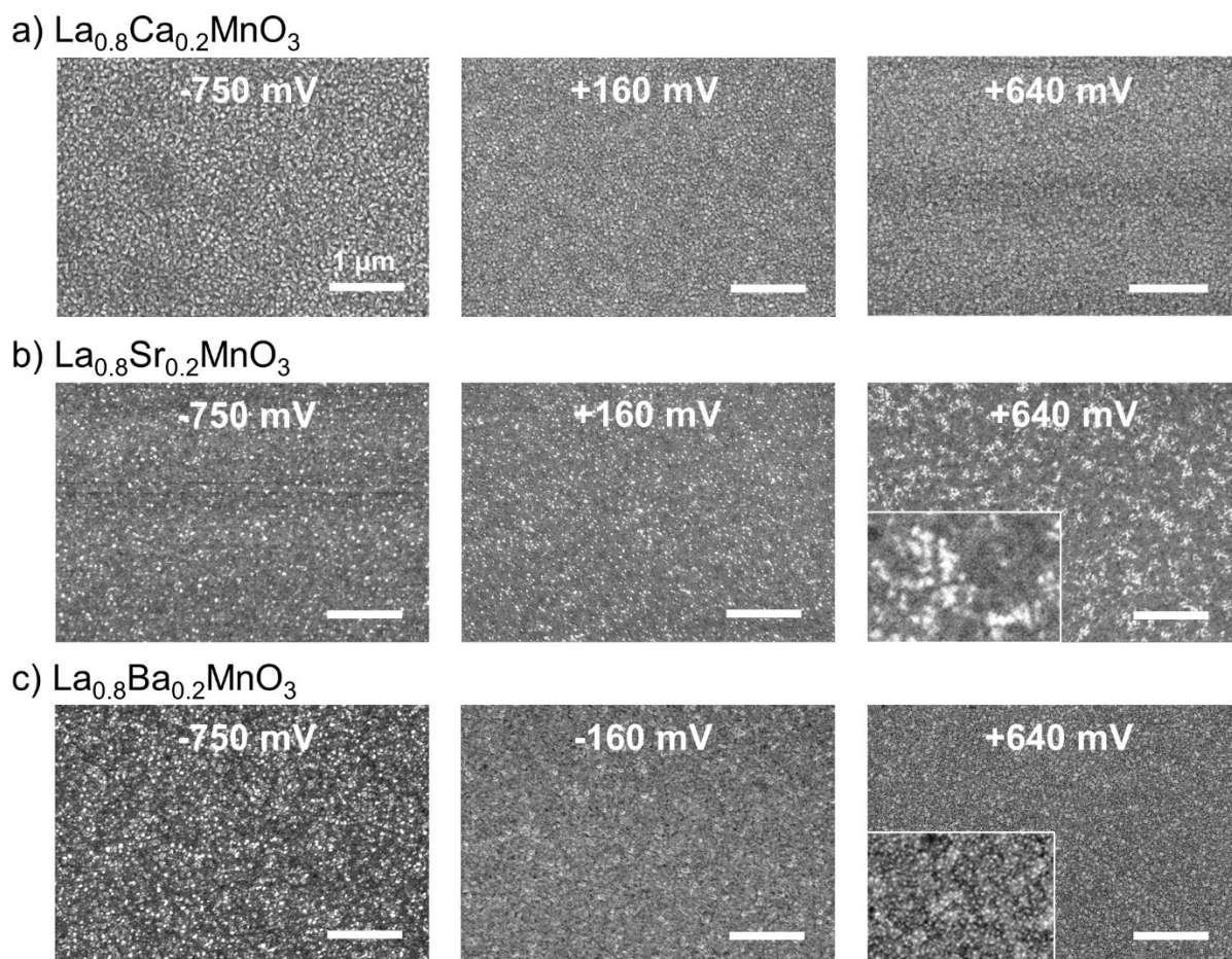
Figure 1-6. SEM images of the \text{La}_{0.8}\text{Ca}_{0.2}\text{MnO}_3 , \text{La}_{0.8}\text{Sr}_{0.2}\text{MnO}_3 , and \text{La}_{0.8}\text{Ba}_{0.2}\text{MnO}_3 surfaces after annealing at 770^\circ\text{C} in 1 atm \text{O}_2 under polarization, acquired at different locations corresponding to the indicated bias voltages. a) \text{La}_{0.8}\text{Ca}_{0.2}\text{MnO}_3 at -750 mV, +160 mV, and +640 mV, b) \text{La}_{0.8}\text{Sr}_{0.2}\text{MnO}_3 at -750 mV, +160 mV, and +640 mV, and c) \text{La}_{0.8}\text{Ba}_{0.2}\text{MnO}_3 at -750 mV, -160 mV, and +640 mV. The magnification of all the images is 25k with a scale bar indicating 1\ \mu\text{m} . Insets in \text{La}_{0.8}\text{Sr}_{0.2}\text{MnO}_3 and \text{La}_{0.8}\text{Ba}_{0.2}\text{MnO}_3 at +640 mV are 4-times further magnified images for a clearer view of small particles on their surface.
