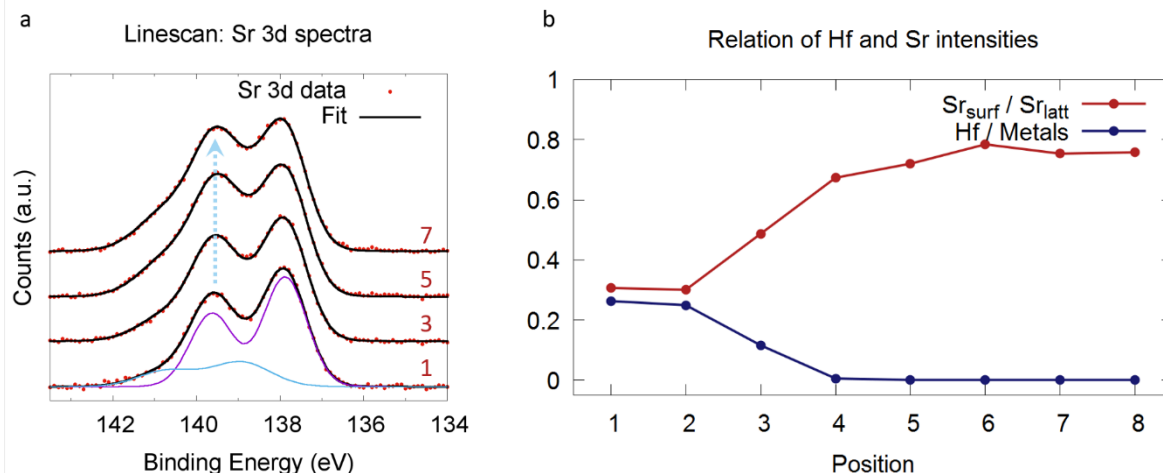
Figure 2-3. Line scan across the \text{La}_{0.8}\text{Sr}_{0.2}\text{MnO}_3 thin film at 450^\circ\text{C} in 1.3 \times 10^{-3} mbar \text{O}_2 . (a) Sr 3d spectra in four positions in different locations moving from the Hf-doped side (1) via a transition zone with low Hf content (3) to the undoped region (5, 7). Segregation increases with decreasing Hf content. (b) Relation of Hf content and \text{Sr}_{\text{surf}}/\text{Sr}_{\text{latt}} ratio in 8 points along a linear path across the sample. \text{Sr}_{\text{surf}}/\text{Sr}_{\text{latt}} shows a direct, inverse dependence on the Hf content.
