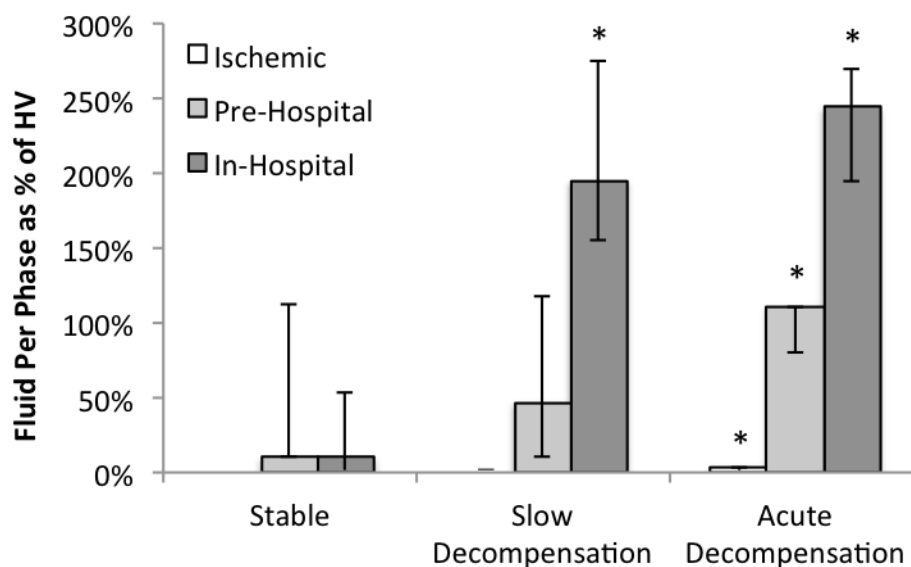
Figure 3 Fluid volume required in each phase of the experiment (Ischemia, Pre-Hospital, and In-Hospital) for each decompensation category. Data expressed as median \pm interquartile range.
