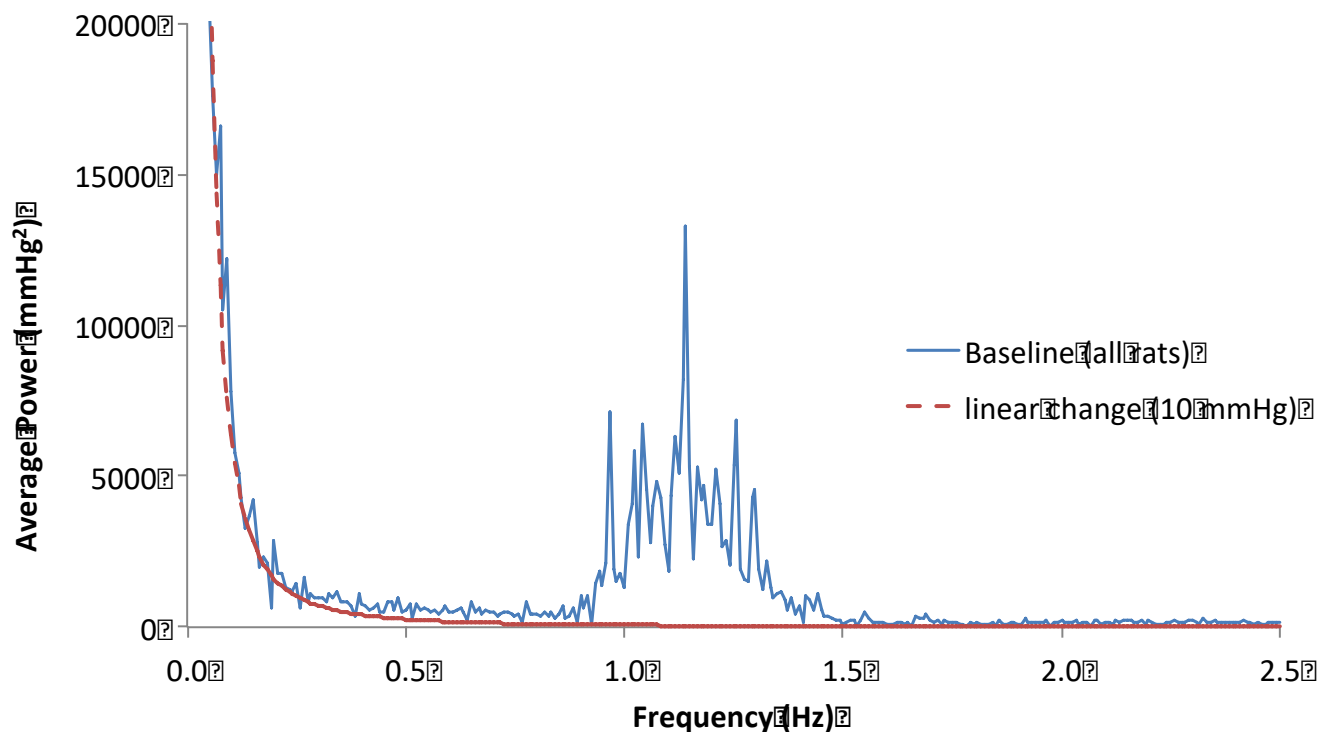
Supplemental Figure 1 Mean power spectrum for mean arterial blood pressure of all subjects at baseline compared to the power spectrum of a line with slope 5 mmHg/min (i.e. a 10-mmHg difference between starting and ending pressure in a 2 min period). The Fast-Fourier Transfer assumption of repeating data causes an artifact in data segments that end at a different value than they begin, resulting in high power at the low frequency range, as demonstrated by the power spectrum for the line segment. The absence of peaks in the low frequency range suggests that Mayer waves (reported to appear around 0.4 Hz) were either suppressed or shifted into very low or high frequency ranges.
