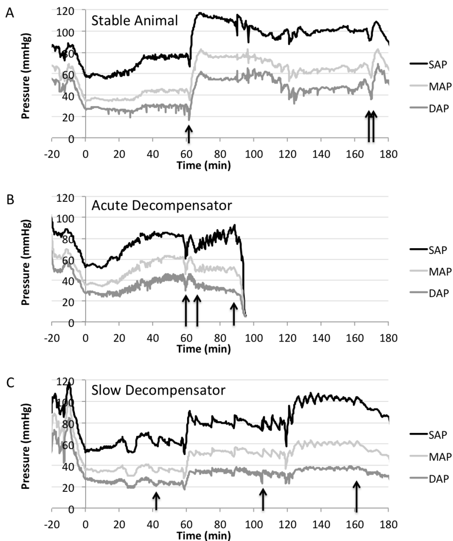
Figure 4 Typical blood pressure traces from each decompensation category. (A) Stable animal, OA-sat BSA group. No fluid needed after treatment bolus (first arrow) in pre-hospital period and only a small amount required in In-hospital period. In the final 20 minutes, a pressure drop triggered fluid administration (second arrow), but it likely was not needed, as pressure continued to rise even after fluids were stopped (third arrow). (B) Acute decompensator, Plasmalyte group. After blood sample, bolus, and initial resuscitation at 60 min (first arrow), pressure begins to fall. Once the MAP hits ~49 mmHg (second arrow), Plasmalyte is given until MAP reaches ~53 mmHg. The process is repeated as needed, giving the MAP its jagged appearance. DAP decreases, balanced by increasing
