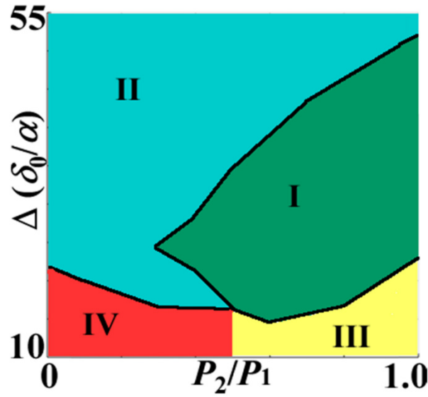
Fig. 15. Stability boundaries for TOD and \delta_{12} = 1 : in Region I the pulse position is stable, in Region II the pulse rotates because the detuning is too high, in Region III the single pulse solution goes back to a chaotic multipulse state, and in Region IV the pulse disappears, and the system transitions to a low-power CW solution.
