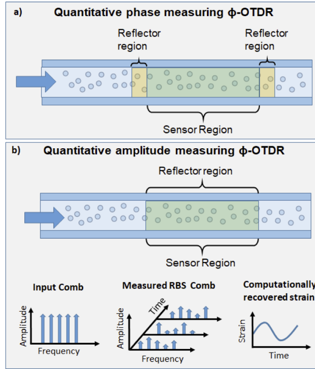
Fig. 1. (a) In a quantitative phase-measuring \phi -OTDR system, strain in the sensor region is proportional to the relative phase between light back-scattered from two reflector regions. (b) In the quantitative amplitude measuring \phi -OTDR system presented in this work, the reflector region and the sensor region are the same. The input pulse consists of multiple frequency components and the amplitude of each frequency component is measured over time. The strain experienced in the sensor region is then computationally recovered from the evolution of the measured RBS comb.
