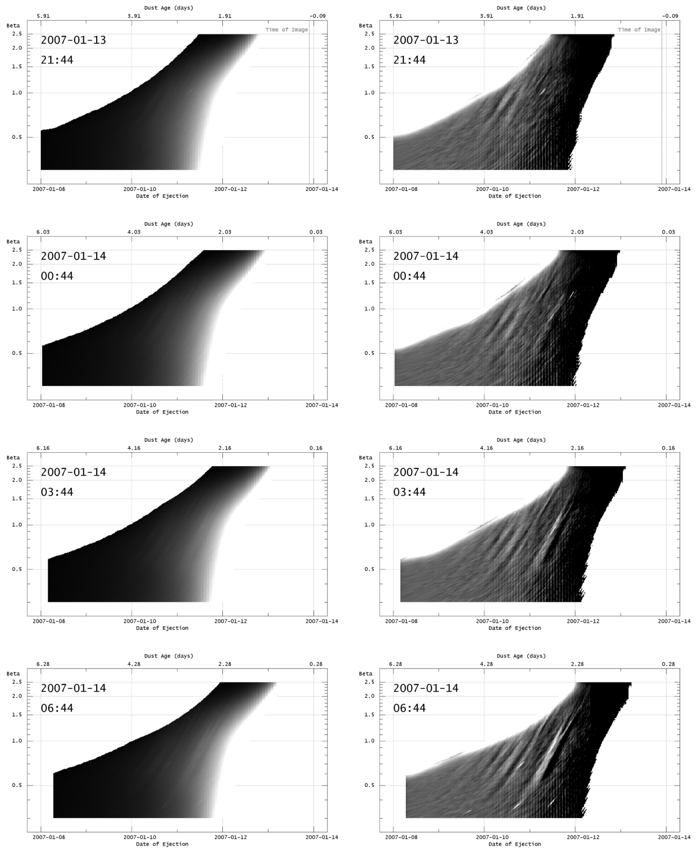
Fig. 12. A sequence of four pairs of temporal maps of the younger dust tail as seen in the SOHO LASCO C3 Blue filter datasets. The left images are temporal maps of the raw data, and the right images are the same temporal maps enhanced to show the structure. Across a 9 h period, structures form from dust released on the 11th January.
