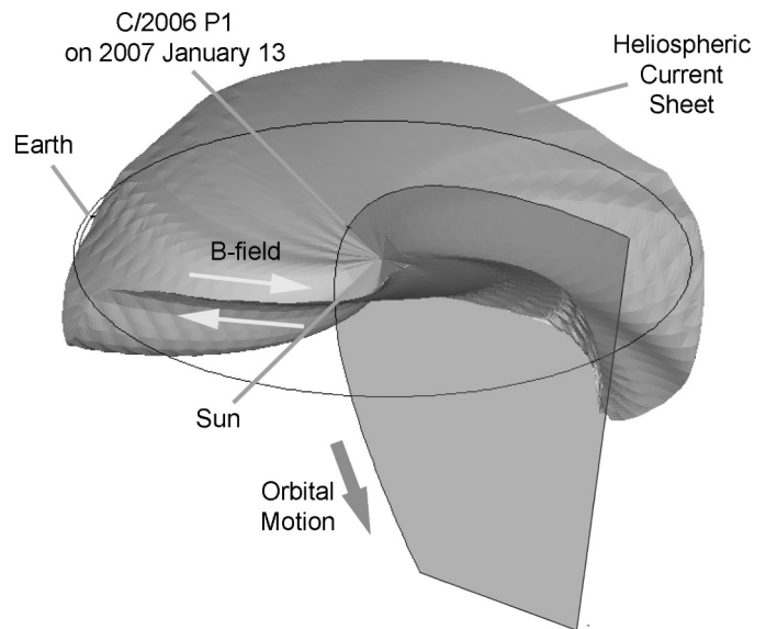
Fig. 19. The relative positions of Comet McNaught's orbit and the heliospheric current sheet, HCS, as estimated from the CORHEL model. Yellow arrows denote the general direction of the heliospheric magnetic field to the north and south of the HCS. Earth's orbit at 1 AU from the Sun is shown as a circle. The HCS, comet nucleus, and planet's positions are shown for 2007 January 13. (For interpretation of the references to colour in this figure legend, the reader is referred to the web version of this article.)
