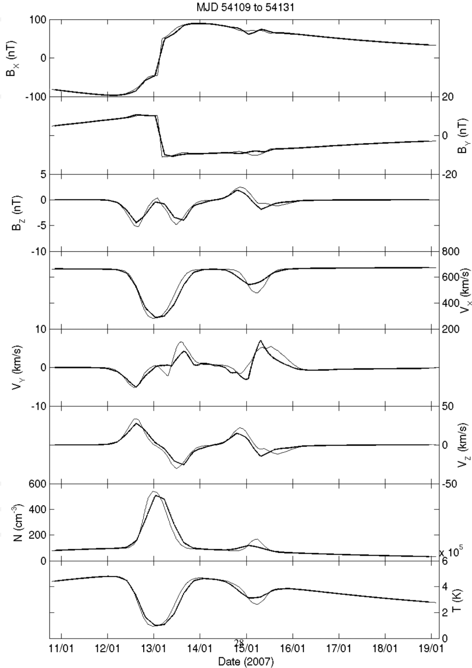
Fig. 18. Solar wind conditions at the nucleus of McNaught estimated using the CORHEL model, extracted along the path of McNaught in Fig. 17 , plotted against date in the format month/day. From top to bottom, the panels show the three components of the heliospheric magnetic field in the Radial-Tangential-Normal coordinate system; three components of the solar wind speed in the same system, the solar wind particle number density, and finally the plasma temperature. The black and grey lines correspond to the two solar magnetogram datasets used.
