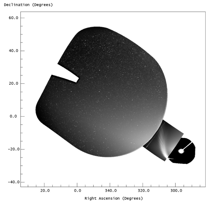
Fig. 6. The view of the comet as seen from STEREO and SOHO on 2007 January 15 at 12:00 UT. The SOHO LASCO C3 field of view is the region at lower right centred on the Sun. STEREO SECCHI HI1-A is the tilted square image containing the bulk of the comet's dust tail. The STEREO SECCHI HI2-A image is the leftmost panel, containing the outermost fringes of the dust tail, with the zodiacal light also apparent.
