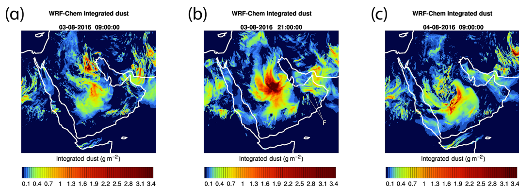
Figure 3. WRF–Chem-simulated vertically integrated dust ( \text{g m}^{-2} ) on the following: (a) 3 August 2016, 09:00 UTC, (b) 21:00 UTC, and (c) 4 August at 09:00 UTC leading up to the 4 August observations of missing dust shown in Fig. 1. The feature “F” in panel (b) denotes pooling of dust along a southerly surge of air near the surface, responding to the low-pressure system in the SG.
