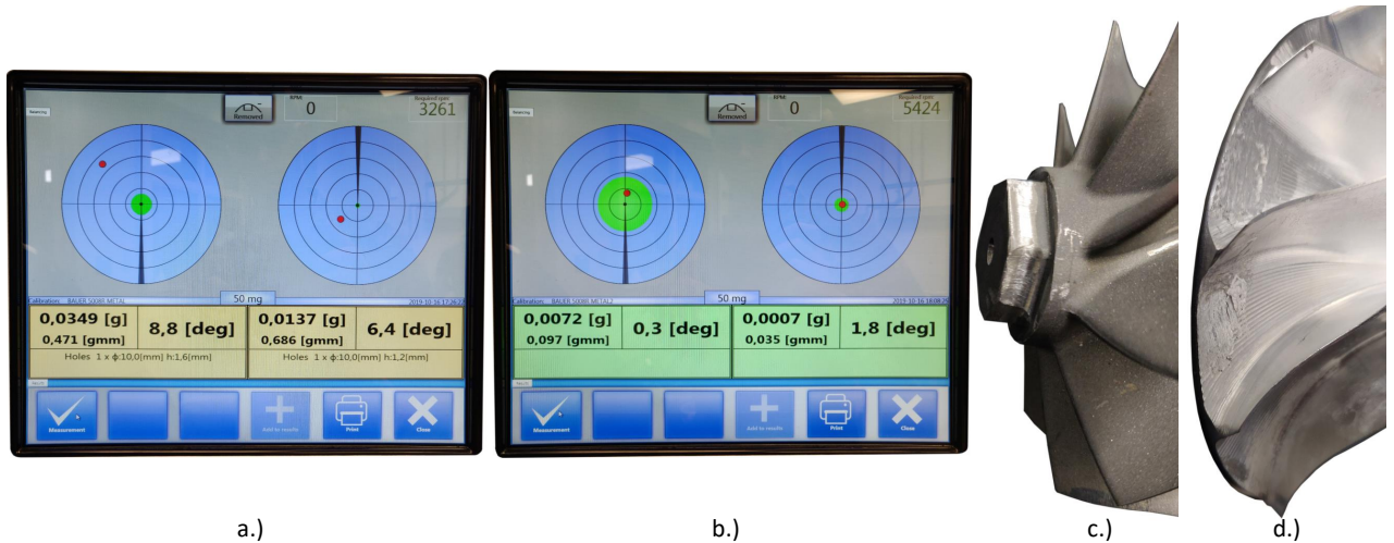
Figure 62. Balancing Test Stand Results. a.) Unbalanced Results. b.) Balanced Results. c.) Balanced Turbine. d.) Balanced Compressor.
