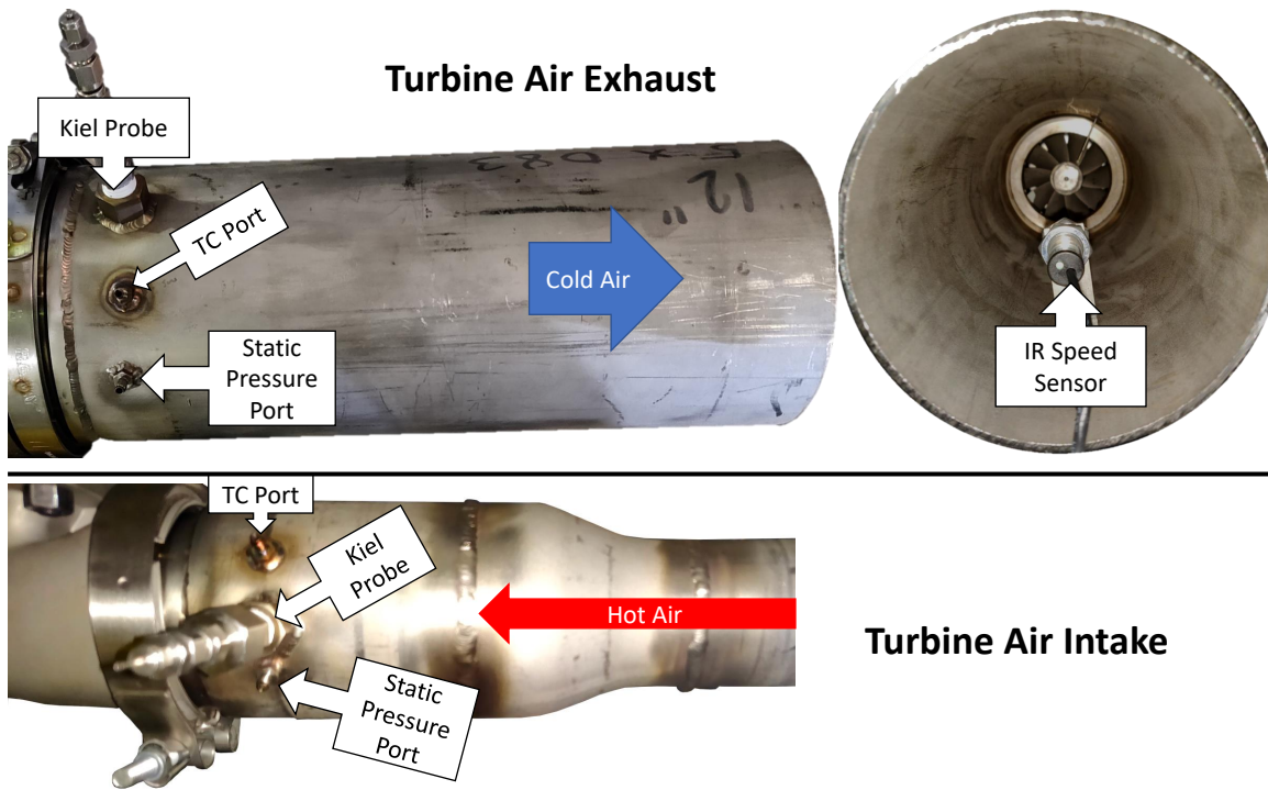
Figure 54. Test Stand Turbine Air Exhaust, Exhaust from Back, and Intake
