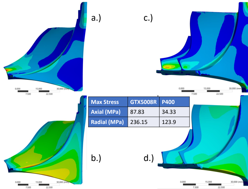
Figure 87. FEA Axial Stresses and Radial Stresses in GTX5008R and P400 Compressor. a.) GTX5008R Axial Stress, 98,000 RPM. b.) GTX5008R Radial Stress, 98,000 RPM. c.) P400 Axial Stress, 50,000 RPM. d.) P400 Radial Stress, 50,000 RPM
