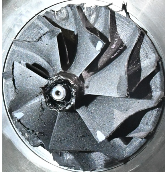
Figure 123. Compressor Failure, P400 Onyx-Carbon Fiber
