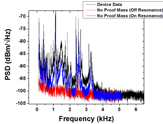
Figure 4. Plot showing low-frequency noise for various combinations of acceleration signal and laser noise.
