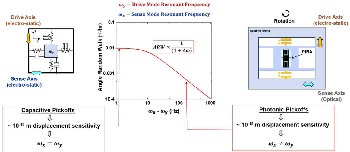
Figure 10. Illustration showing improved performance using optical vs. capacitive pickoffs in MEMS gyro.
