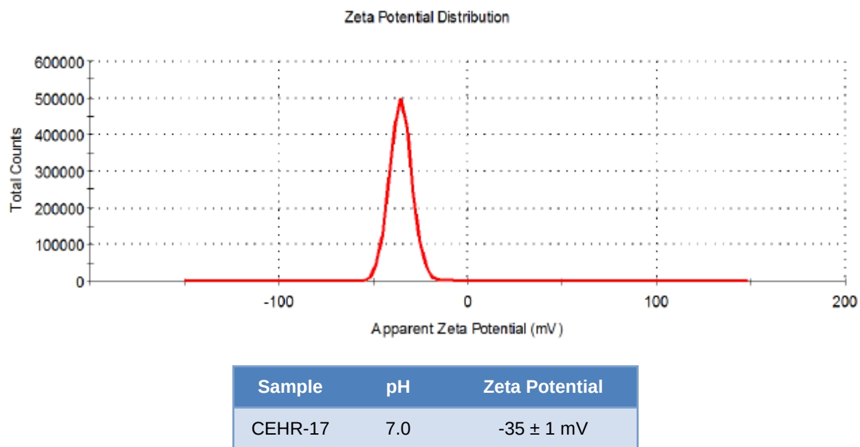
Figure V-13. The averaged zeta potential distributions for CEHR-17 diluted 10,000-fold in deionized water.
