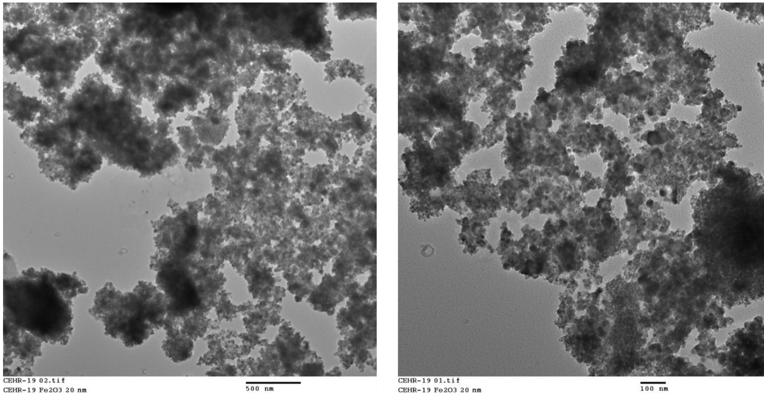
Figure VI-2. Representative TEM Images of CEHR-19. Two representative images are shown for CEHR-19, showing the severity of particle agglomeration within the sample. This sample could not be sized.
