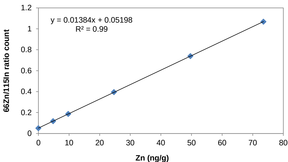
Figure V-7. Zinc Calibration Curve. A typical calibration curve ranging from 0 to 75 Zn ng/g, used to calculate the zinc concentration in CEHR-16 and CEHR-17. The calibration curve was constructed from NIST SRM 3168a zinc standard.
