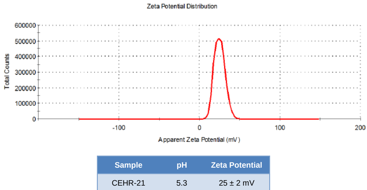
Figure VII-16. The averaged zeta potential distributions for CEHR-21 diluted 100-fold in deionized water.
