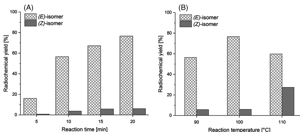
FIGURE 4 The effect of the reaction time and temperature on the radiochemical yields of ( E )- and ( Z )-[ 18 F] tert -Bu-FACH in tert -BuOH/acetoneitrile (ACN) (2:1): A, the reaction was accomplished at 100°C, and samples were taken at different time points; B, the reactions were carried out at different temperatures for 20 minutes ( n = 2 )
