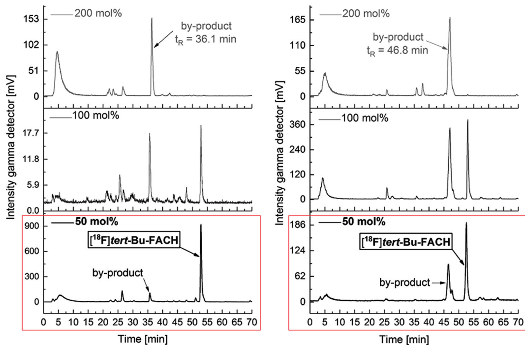
FIGURE 3 Representative radio-HPLC chromatograms showing the effect of different amounts of the K[^{18}\text{F}]F\text{-K}_{2.2.2} -carbonate complex on the radiochemical yields of [^{18}\text{F}]\text{tert-Bu-FACH} in dimethylsulfoxide (DMSO) at 135^\circ\text{C} (left) and acetonitrile (ACN) at 100^\circ\text{C} (right); condition A was applied for HPLC measurements (see supporting information)
