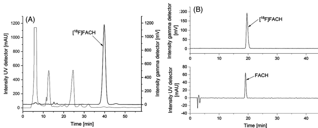
FIGURE 5 A, Representative semi-preparative radio- and UV-HPLC chromatograms of [^{18}\text{F}]\text{FACH} (conditions: Reprisil-Pur C18-AQ, 250 mm \times 10 mm, 46% acetonitrile (ACN)/20 mM \text{NH}_4\text{HCO}_2 aq., pH = 4-5, flow: 3.5 mL/min); B, Representative analytical radio- and UV-HPLC chromatograms of [^{18}\text{F}]\text{FACH} co-eluted with the reference FACH (conditions: Reprisil-Pur C18-AQ, 250 mm \times 4.6 mm, 46% ACN/20 mM \text{NH}_4\text{HCO}_2 aq., pH = 4-5, flow: 1.0 mL/min)
