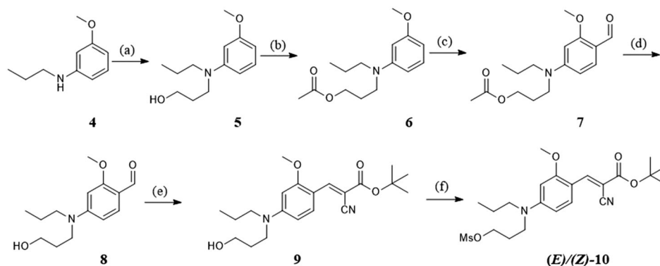
SCHEME 2 Synthesis of precursor 10 : (a) Br(CH 2 ) 3 OH, K 2 CO 3 , acetonitrile (ACN), reflux, 88%; (b) AcCl, pyridine, dichloromethane (DCM), R.T.; (c) POCl 3 /DMF, 80 °C, 79%; (d) K 2 CO 3 , MeOH/H 2 O (1:1), 30 minutes, R.T.; (e) tert -butyl cyanoacetate, piperidine, ACN, reflux, 90%; (f) MsCl, Et 3 N, DCM, 30 minutes, greater than 98%
