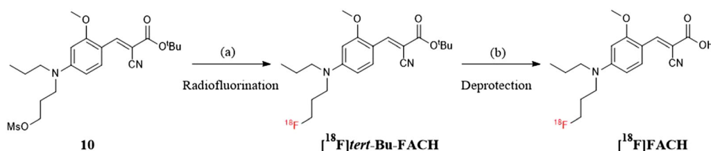
SCHEME 3 Two-step approach for the radiosynthesis of the novel monocarboxylate transporter (MCT) radioligand [ 18 F] FACH : (a) K[ 18 F]F-K 2.2.2 -carbonate complex or [ 18 F]TBAF, acetonitrile (ACN), 15 minutes, 100°C; (b) i. trifluoroacetic acid (TFA), ACN, 15 minutes, r.t.; ii. Et 3 N
