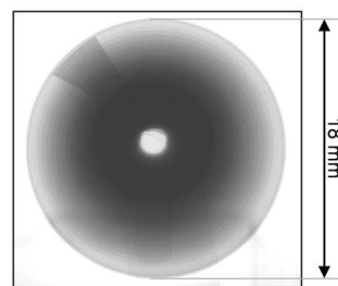
FIGURE 7 | (A) Discharge capacity of Equilibrium 20°C over 100 cycles and Equilibrium 0°C and Transient 40 to 0°C cells to 25% capacity fade. X-ray radiograph after 30% capacity fade for cells subjected to (B) Equilibrium 0°C and (C) Transient 40 to 0°C with evidence of jellyroll collapse, contrasted to the Equilibrium 20°C cell cycled 100 times without mechanical degradation (D) .
